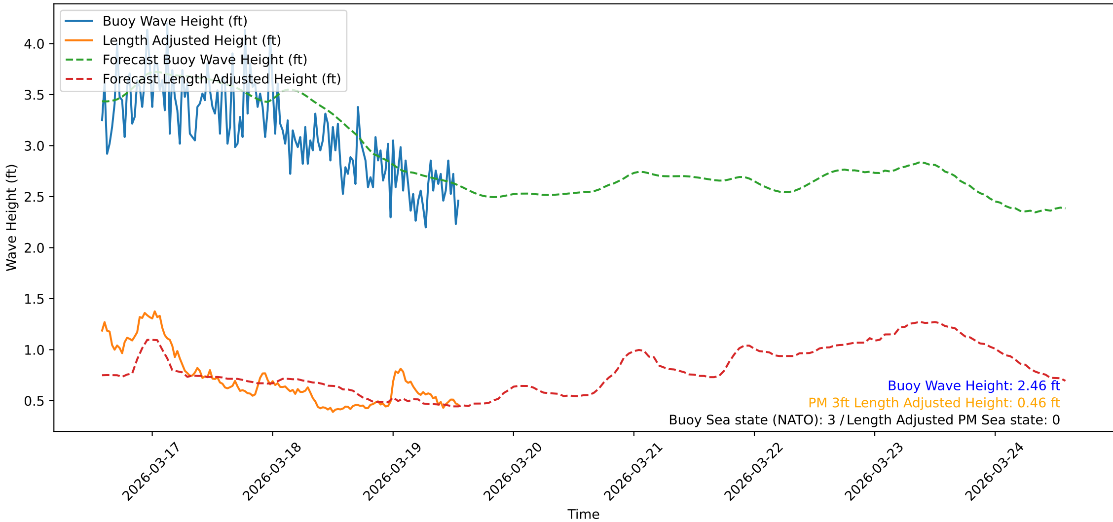
Wave Heights over Time for Green Beach at 2026-03-19 13:51:09
