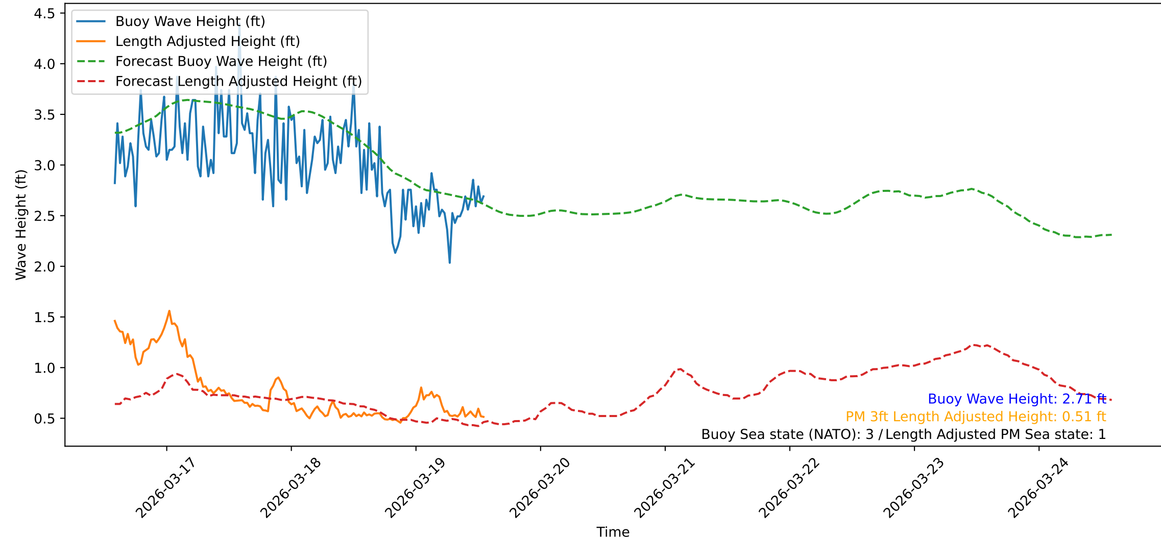
Wave Heights over Time for Oceanside Harbor at 2026-03-19 13:50:31
