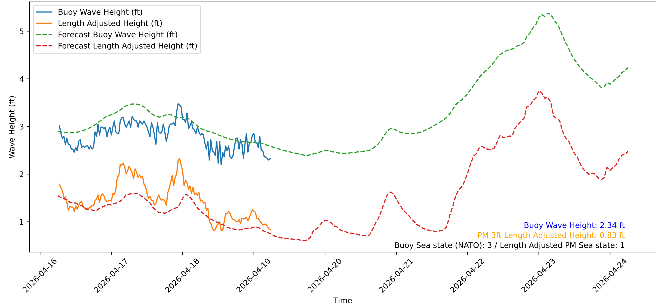
Wave Heights over Time for Green Beach at 2026-04-19 06:21:13
