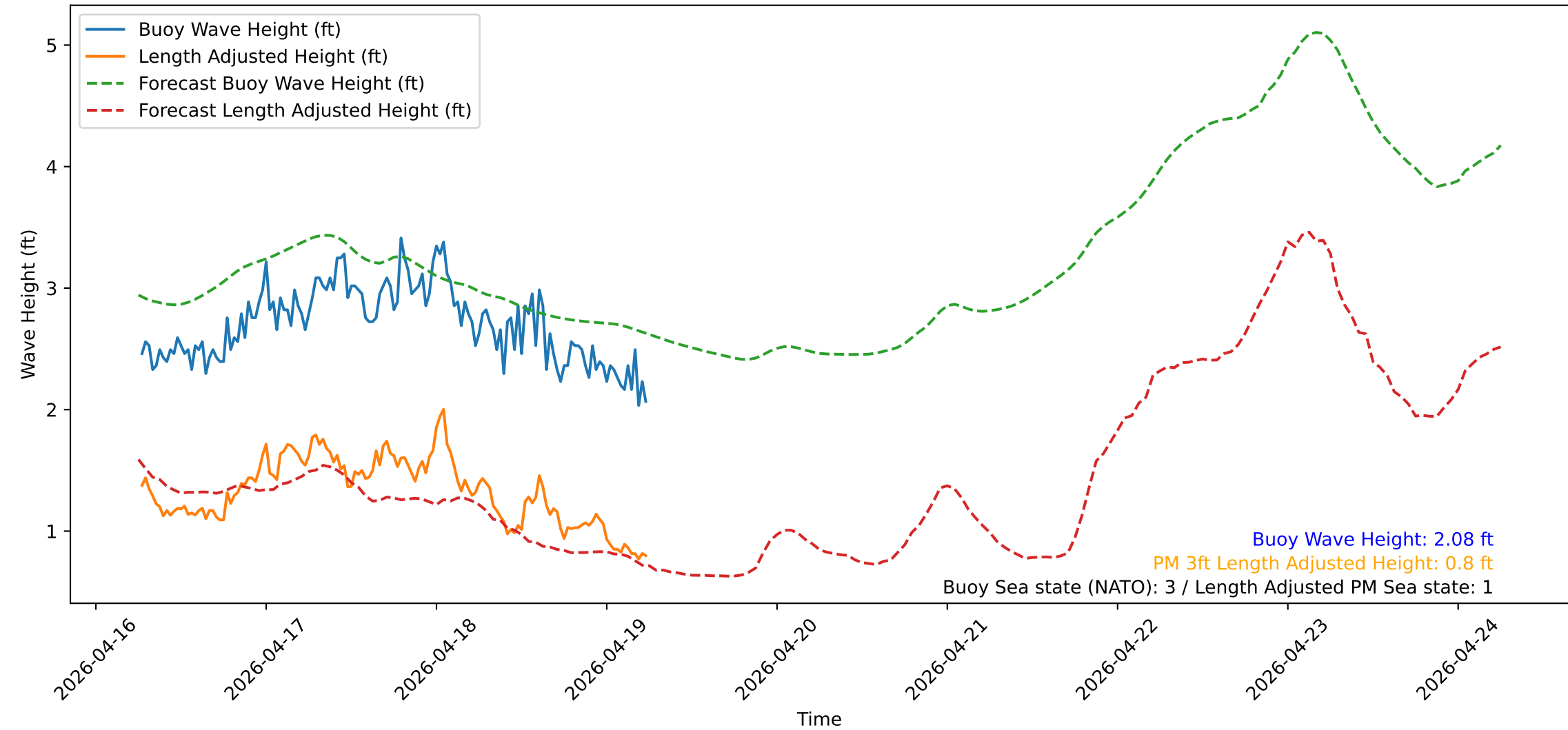
Wave Heights over Time for Oceanside Harbor at 2026-04-19 06:20:31
