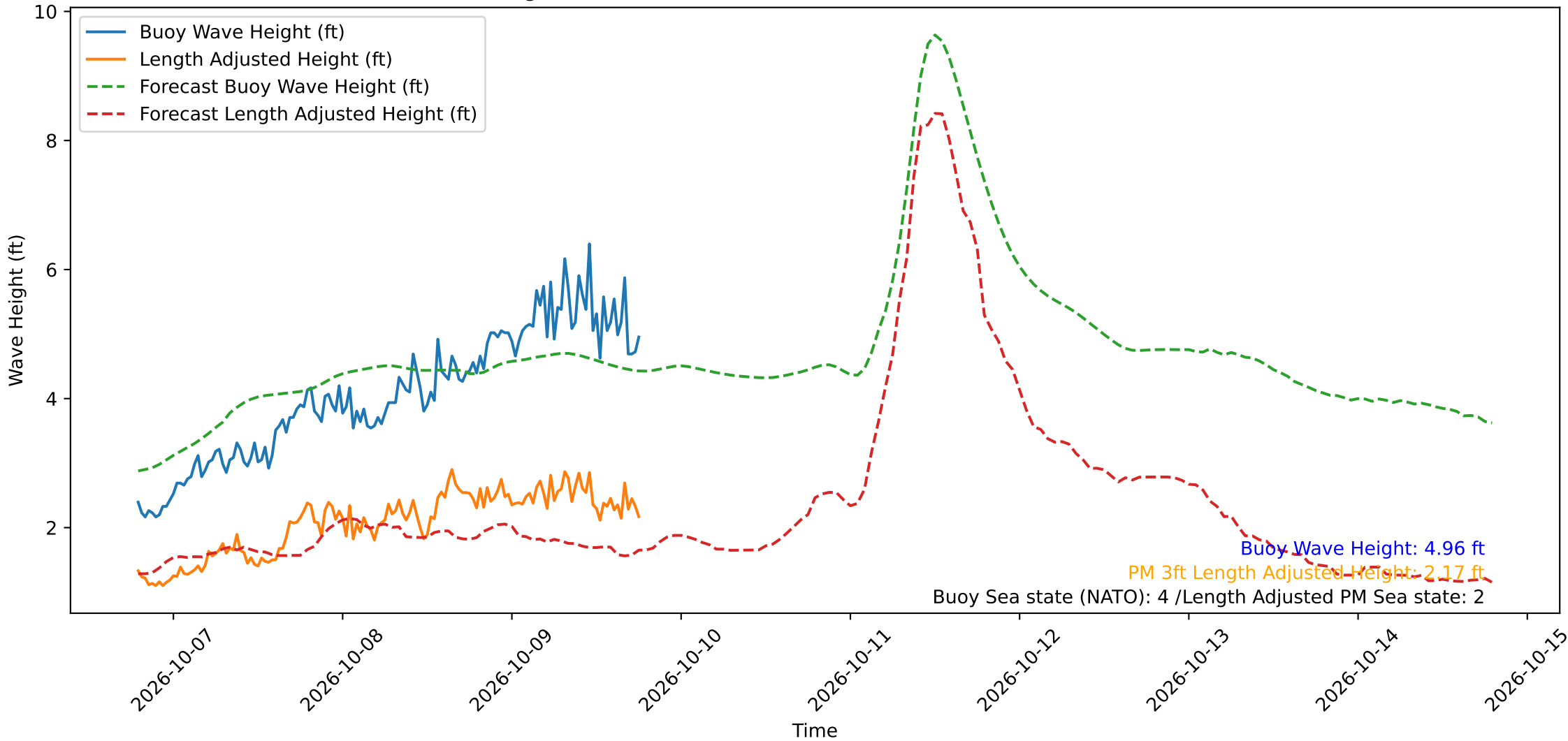
Wave Heights over Time for Oceanside Harbor at 2026-10-09 18:50:29
