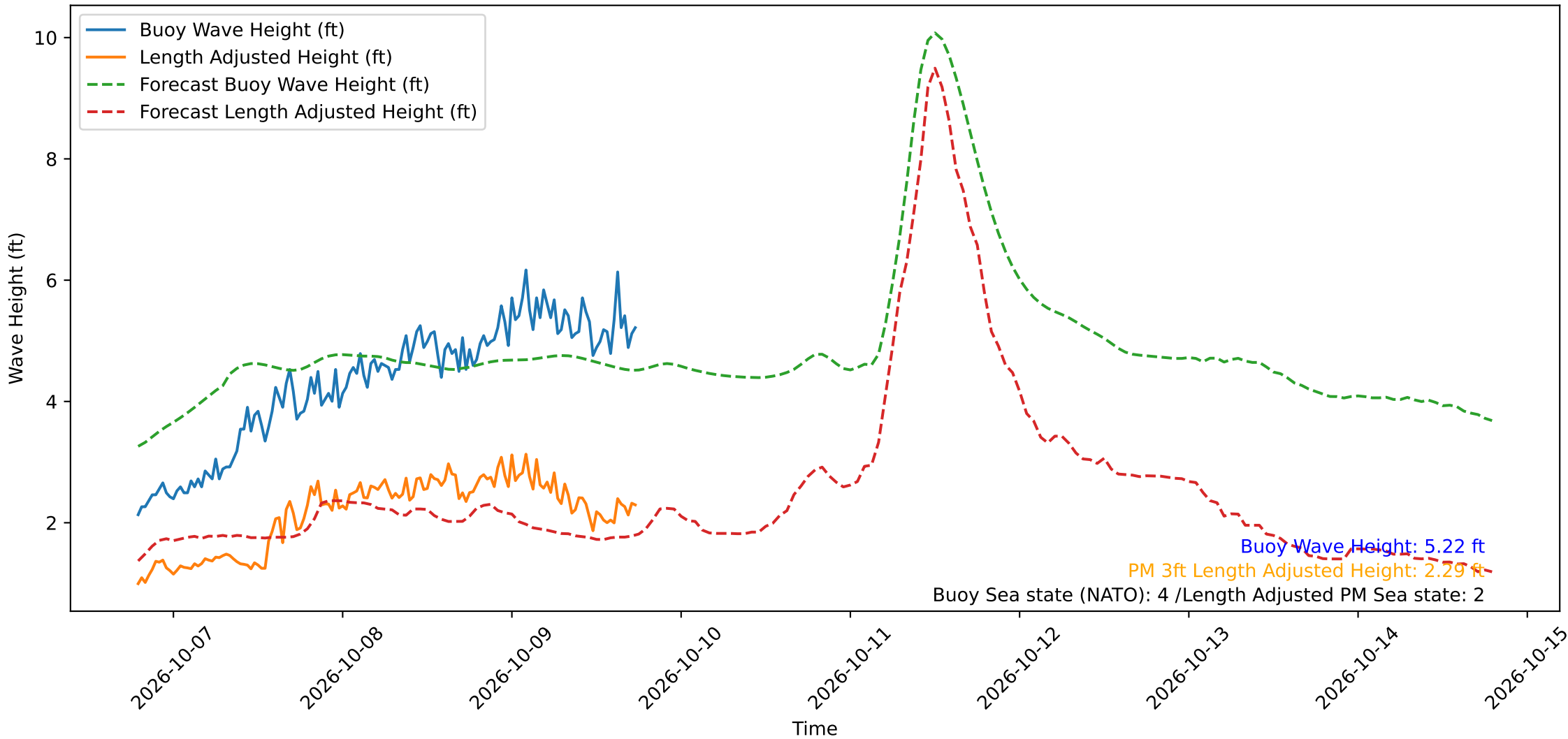
Wave Heights over Time for Green Beach at 2026-10-09 18:51:14
