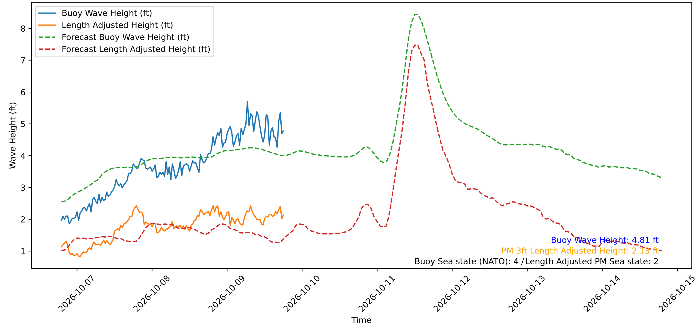
Wave Heights over Time for Red Beach at 2026-10-09 18:50:50
