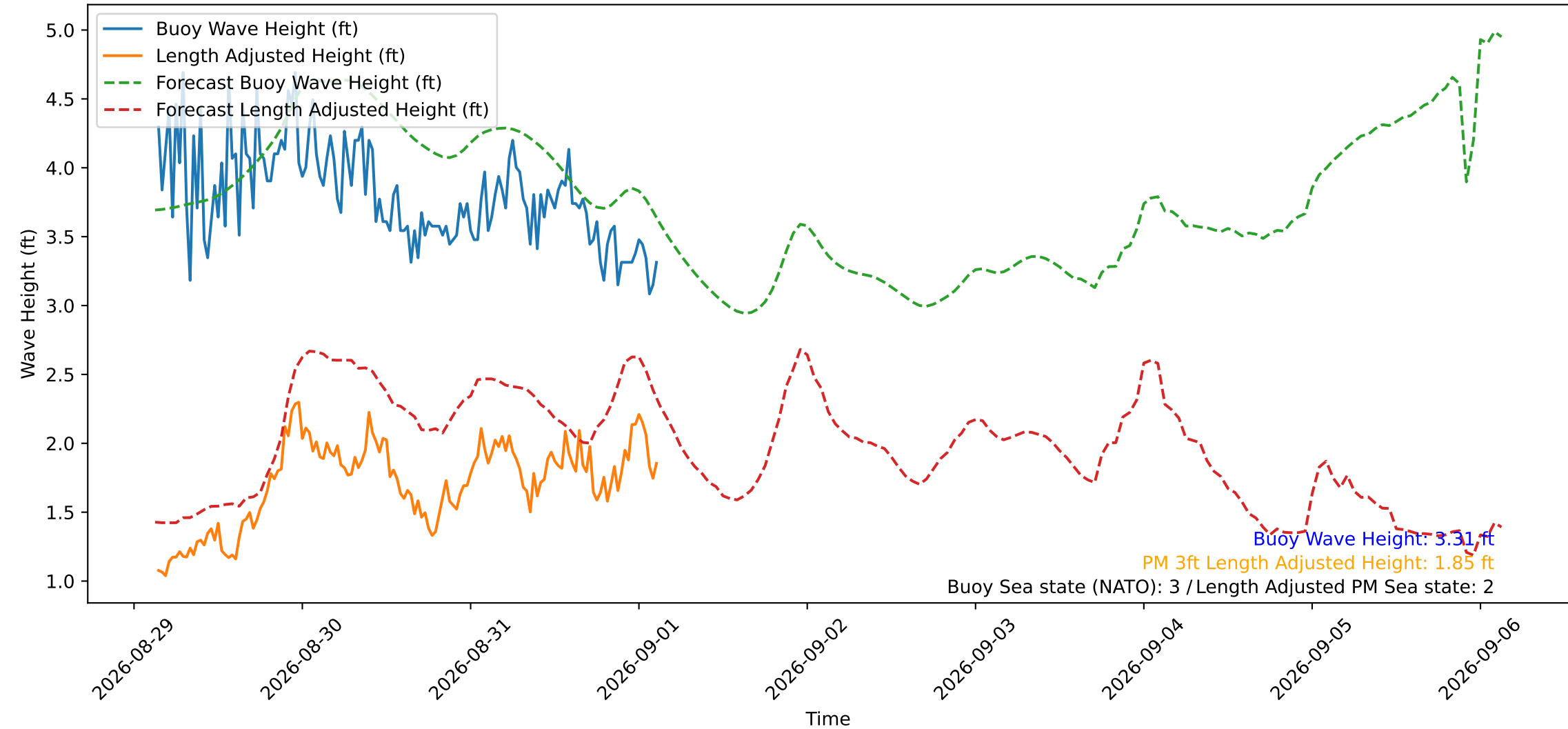
Wave Heights over Time for Red Beach at 2026-09-01 03:20:52
