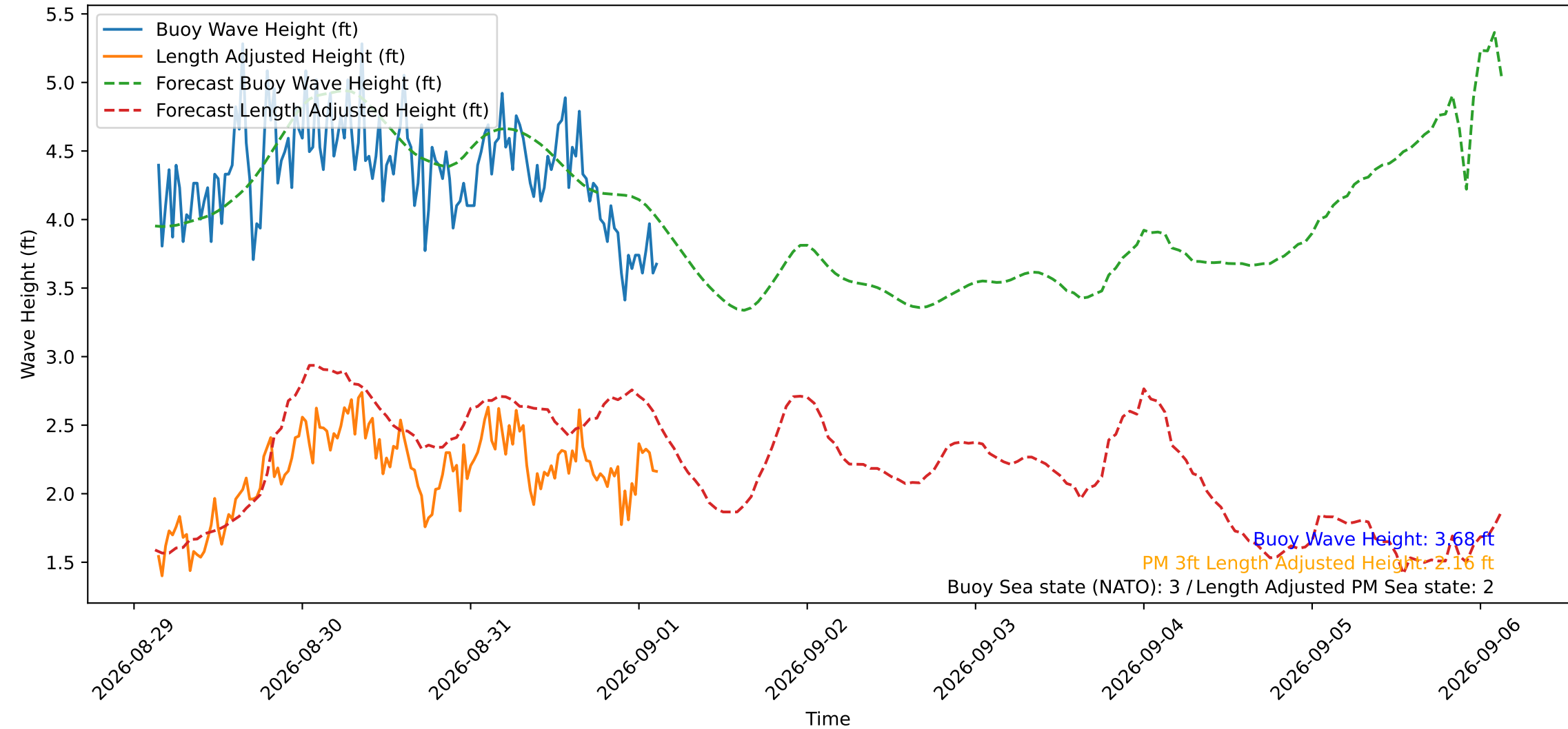
Wave Heights over Time for Oceanside Harbor at 2026-09-01 03:20:30
