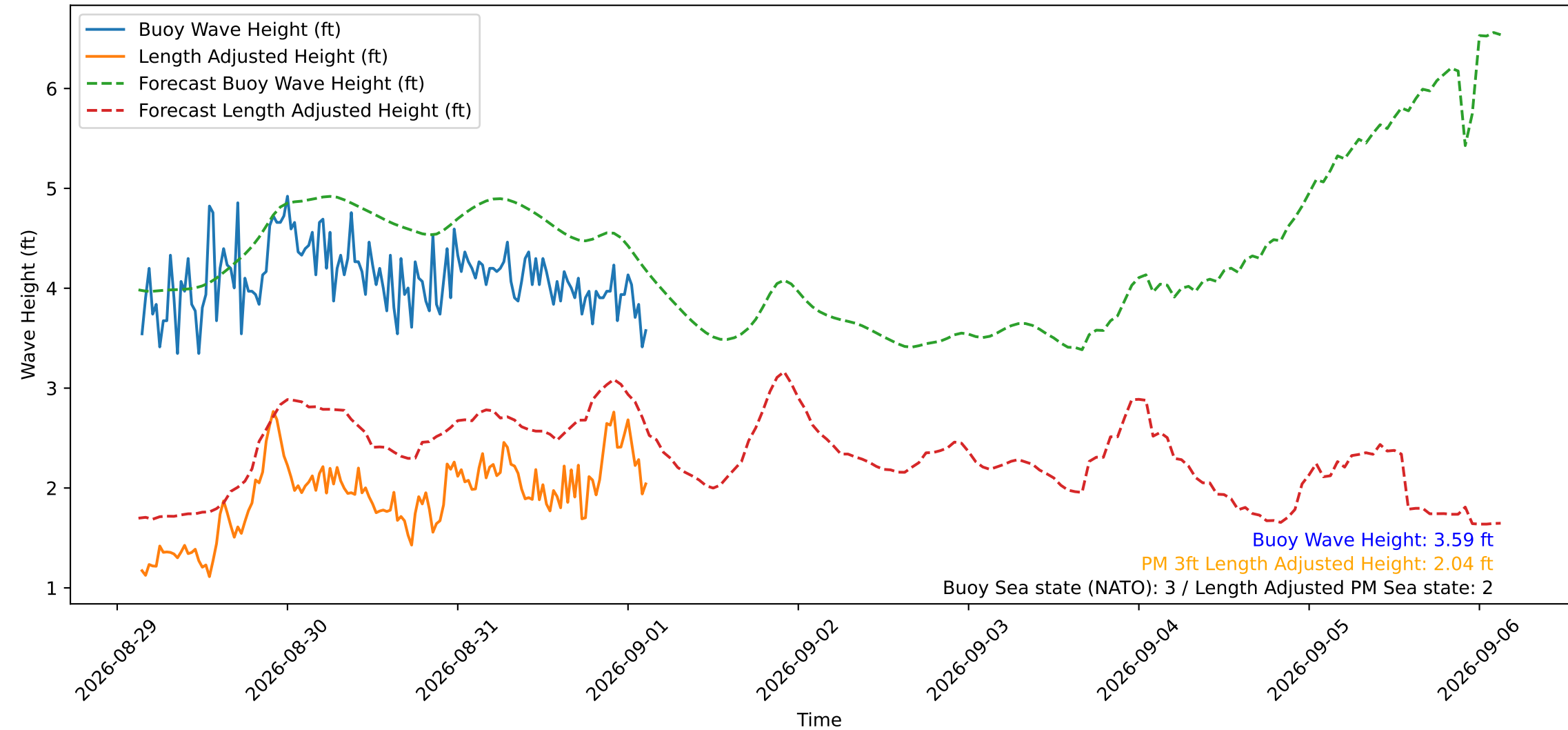
Wave Heights over Time for Green Beach at 2026-09-01 03:21:16
