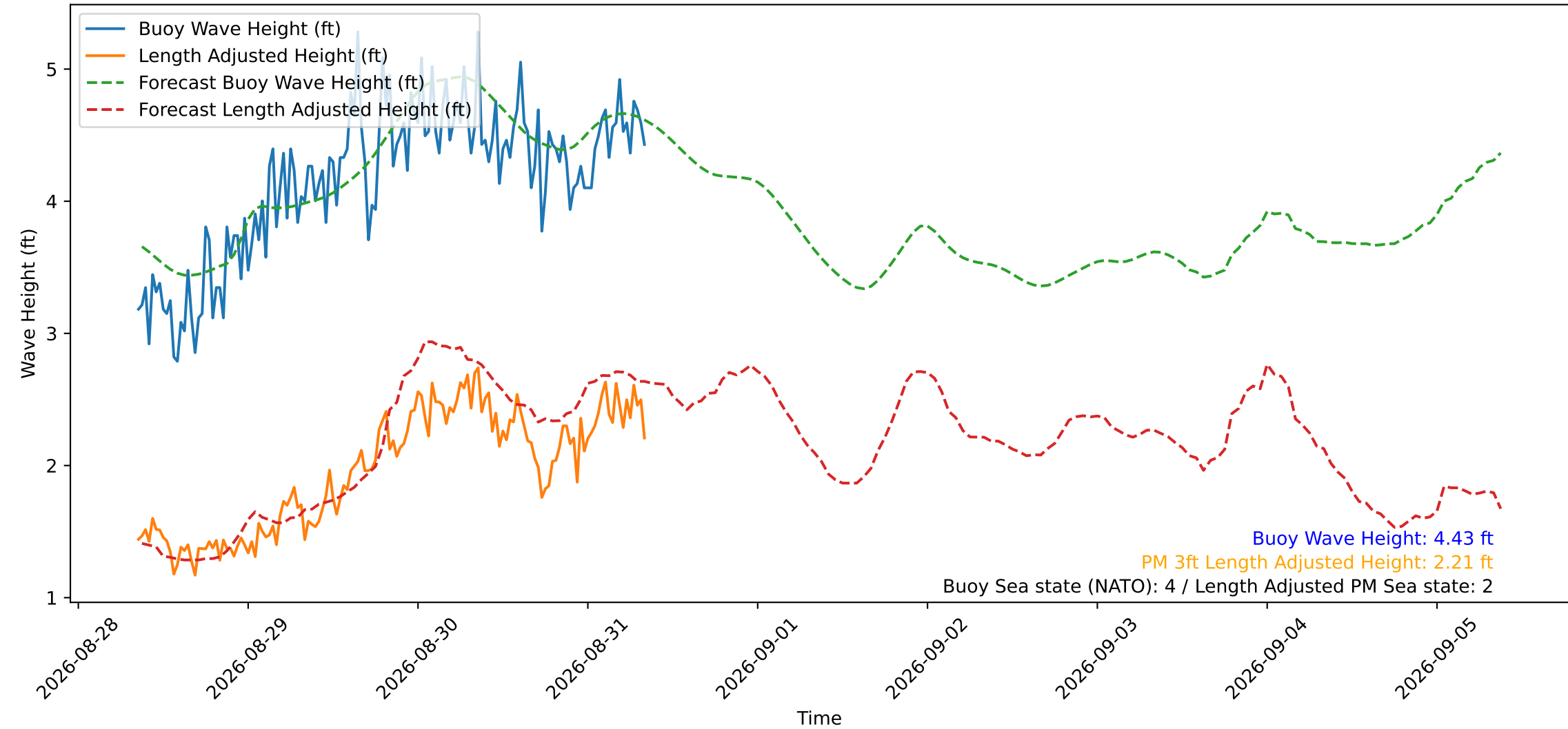
Wave Heights over Time for Oceanside Harbor at 2026-08-31 08:40:29
