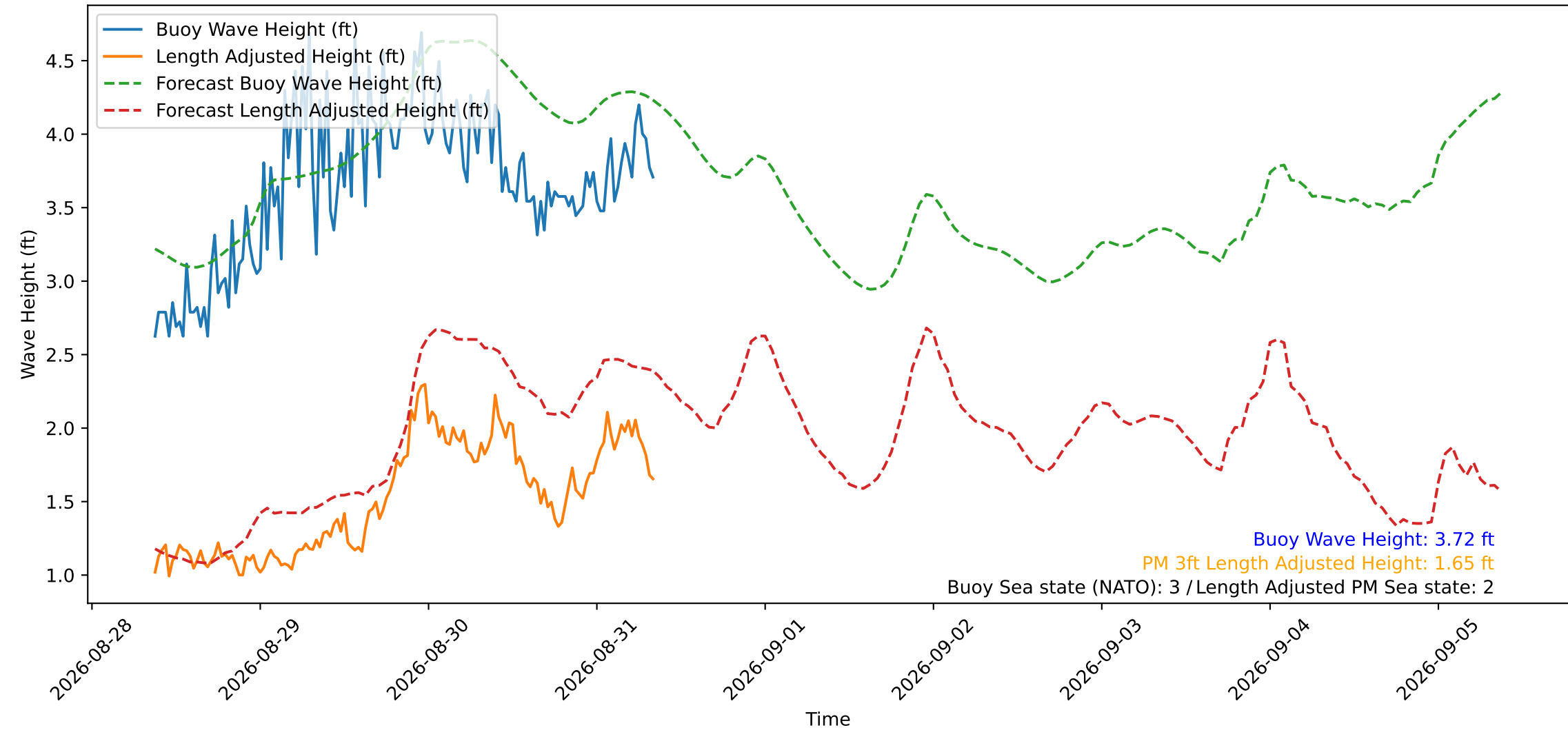
Wave Heights over Time for Red Beach at 2026-08-31 08:40:49
