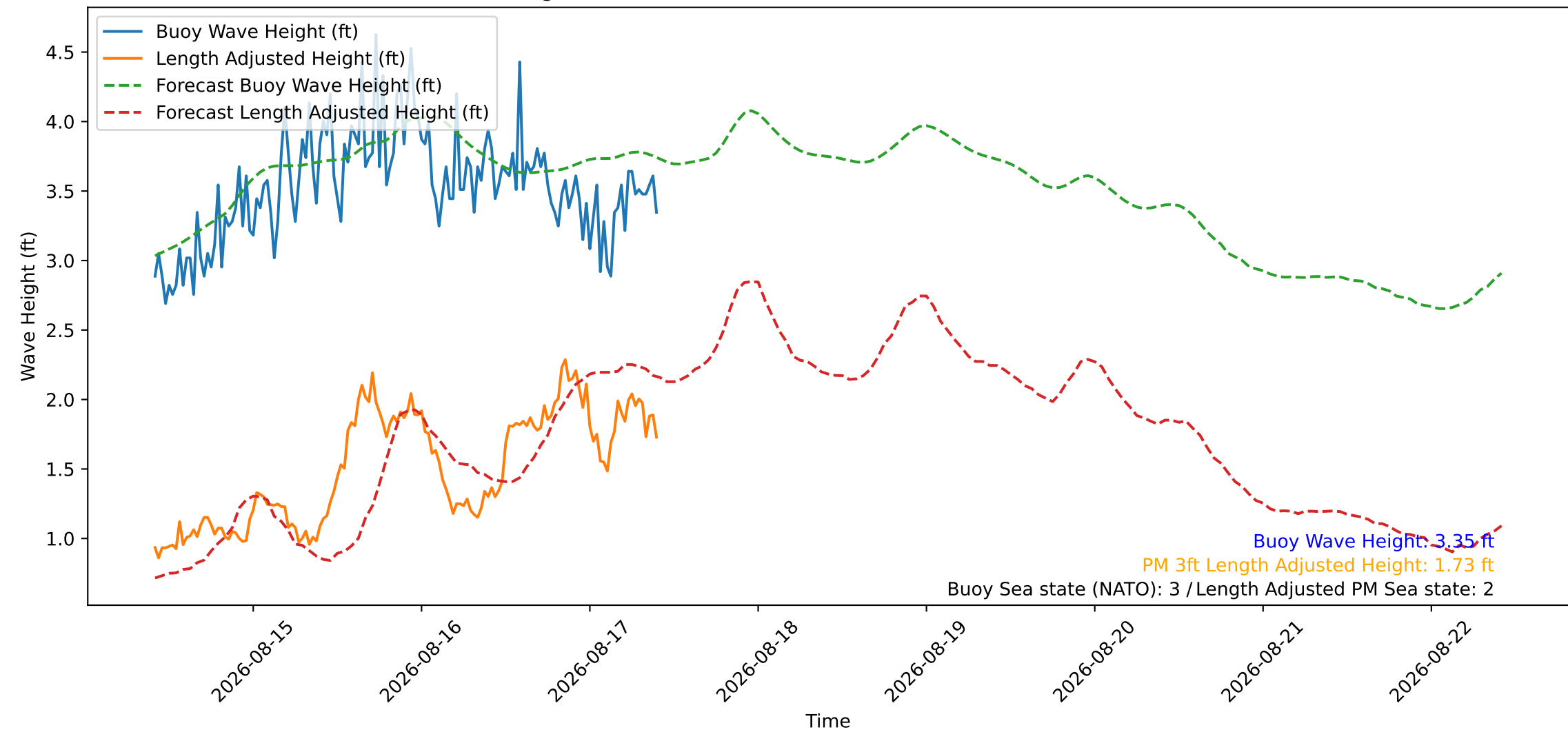
Wave Heights over Time for Oceanside Harbor at 2026-08-17 10:00:27
