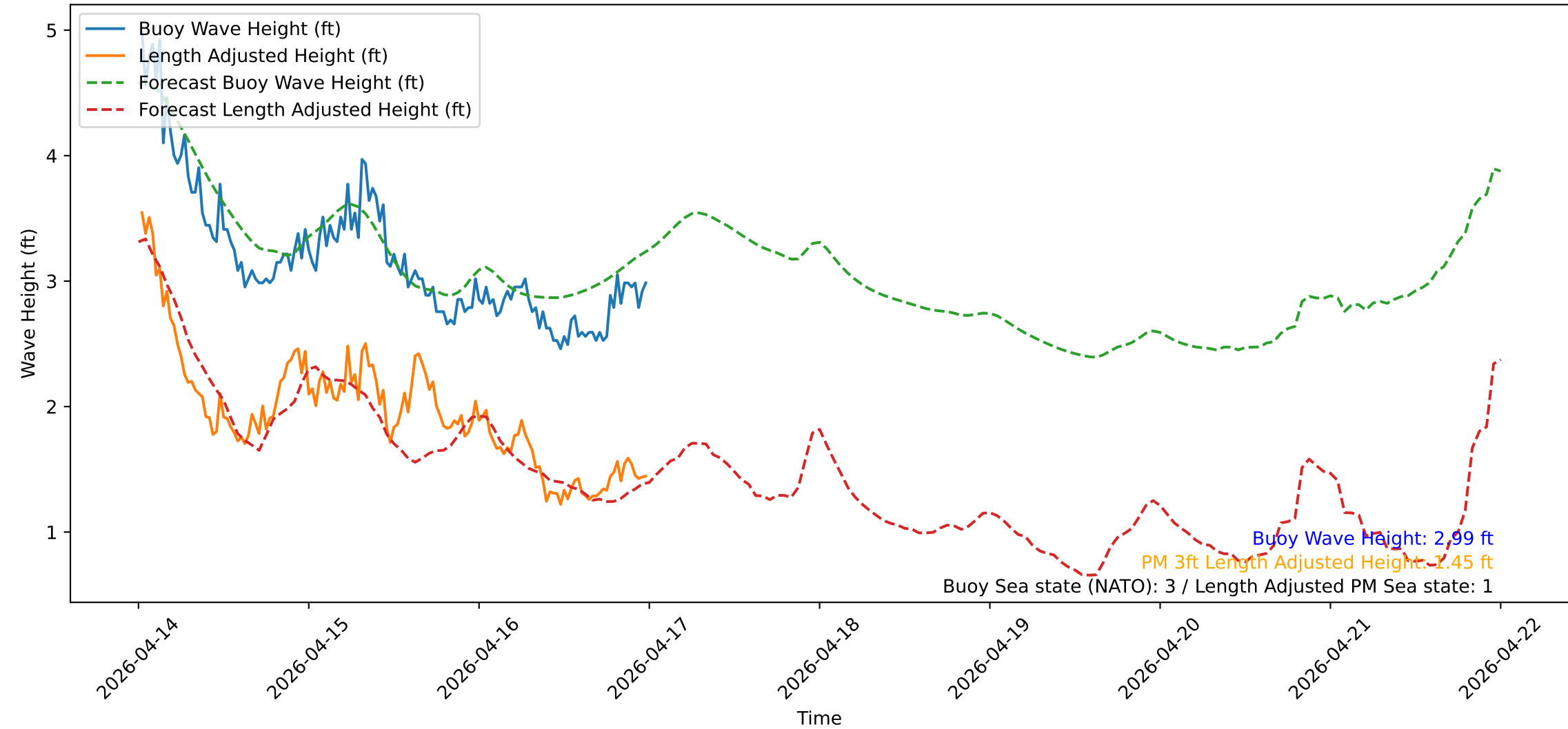
Wave Heights over Time for Green Beach at 2026-04-17 00:21:13
