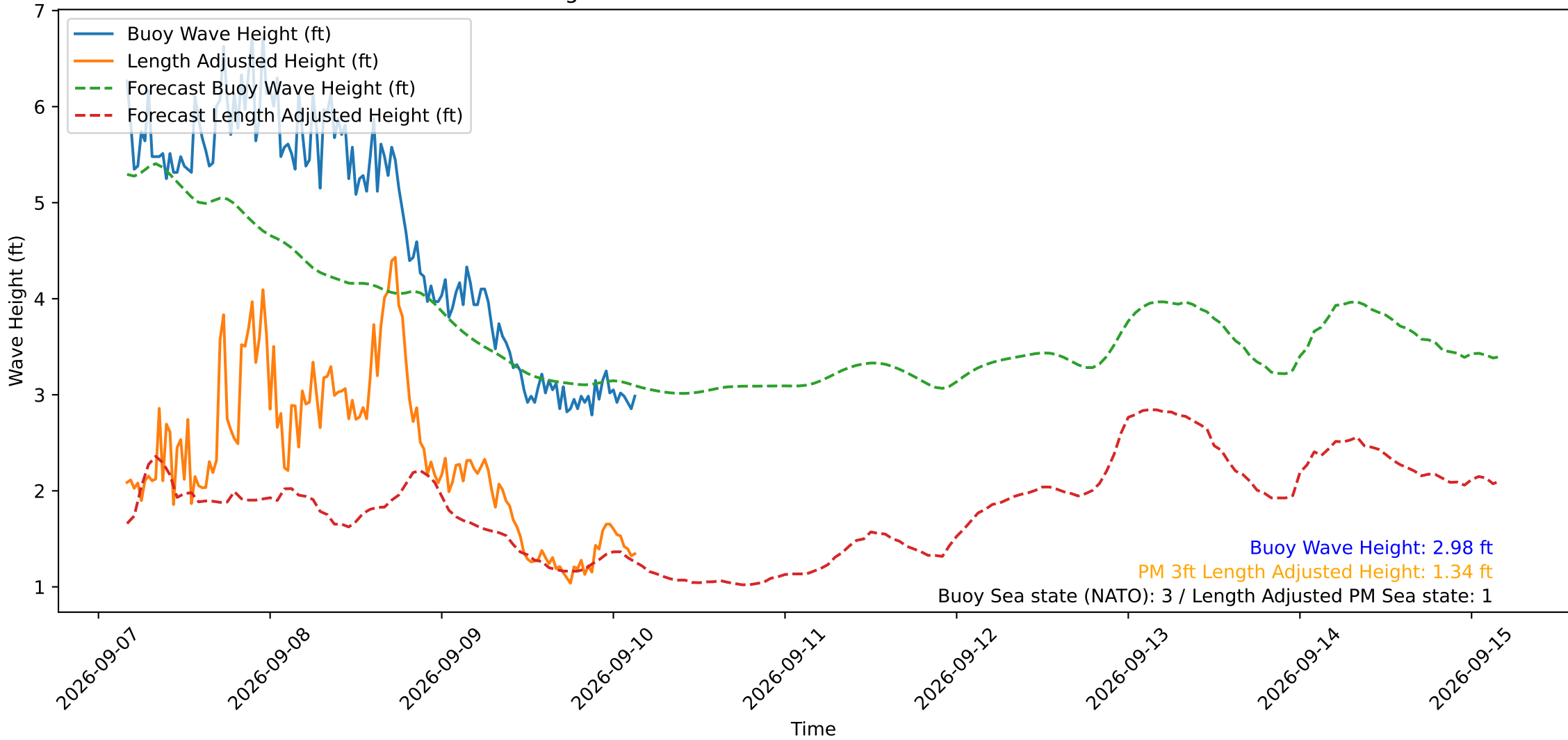
Wave Heights over Time for Red Beach at 2026-09-10 03:50:50
