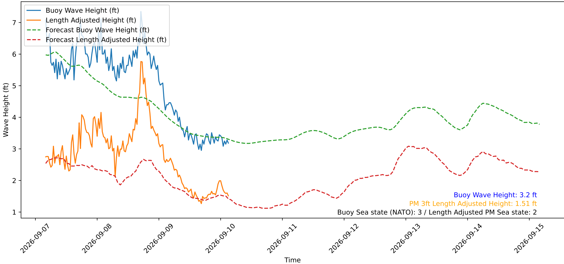
Wave Heights over Time for Oceanside Harbor at 2026-09-10 03:50:29
