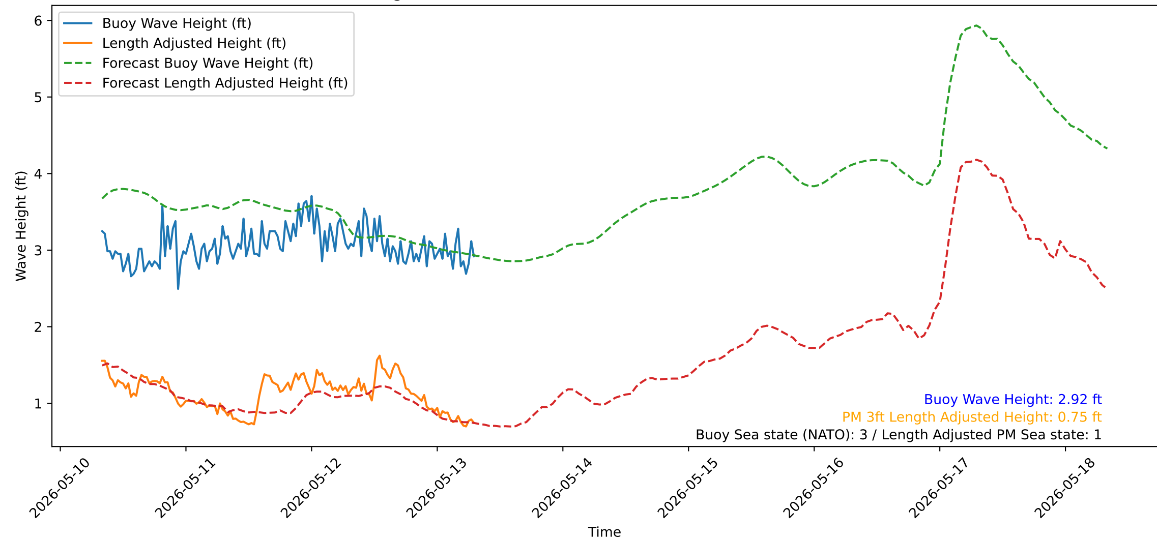
Wave Heights over Time for Oceanside Harbor at 2026-05-13 07:50:31
