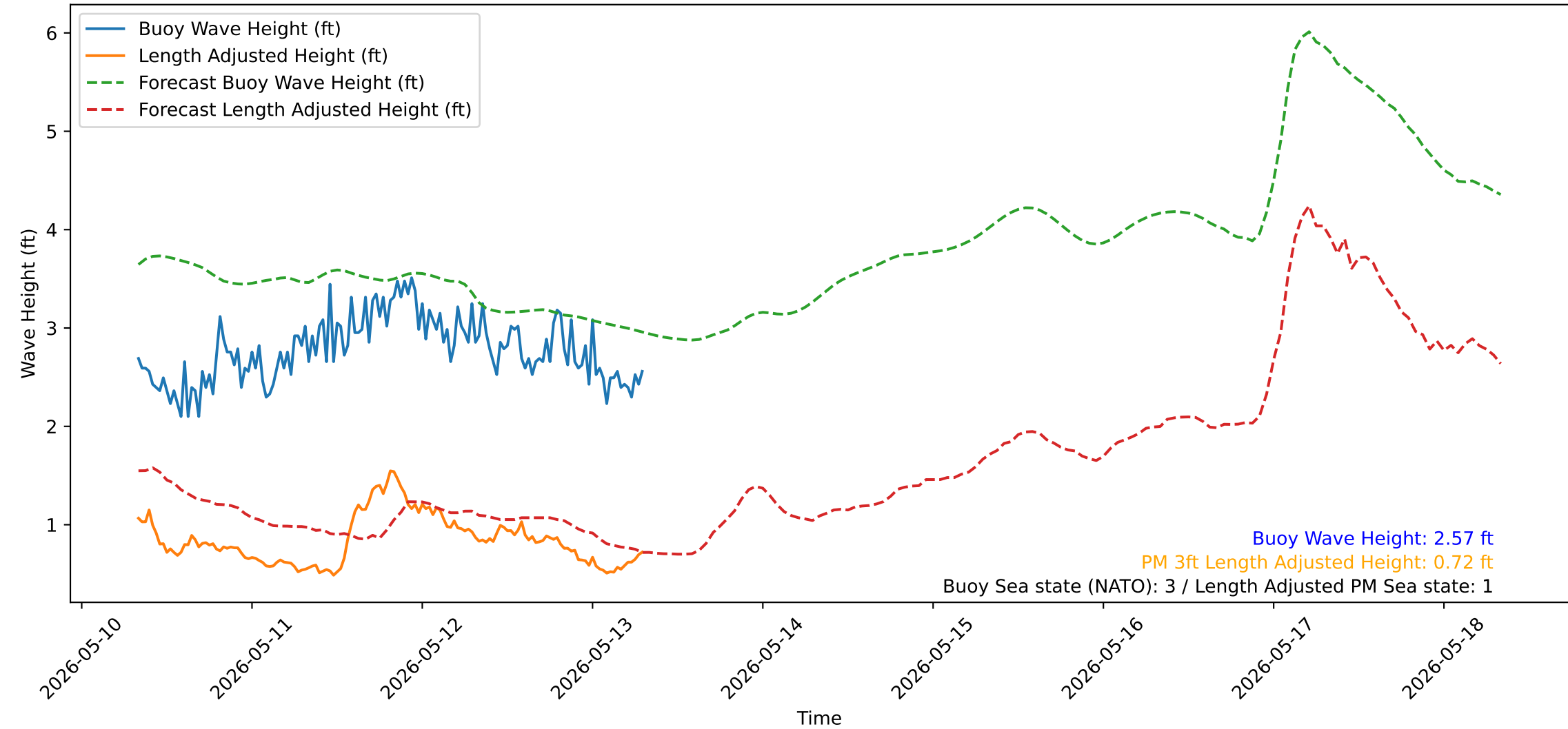
Wave Heights over Time for Green Beach at 2026-05-13 07:51:14
