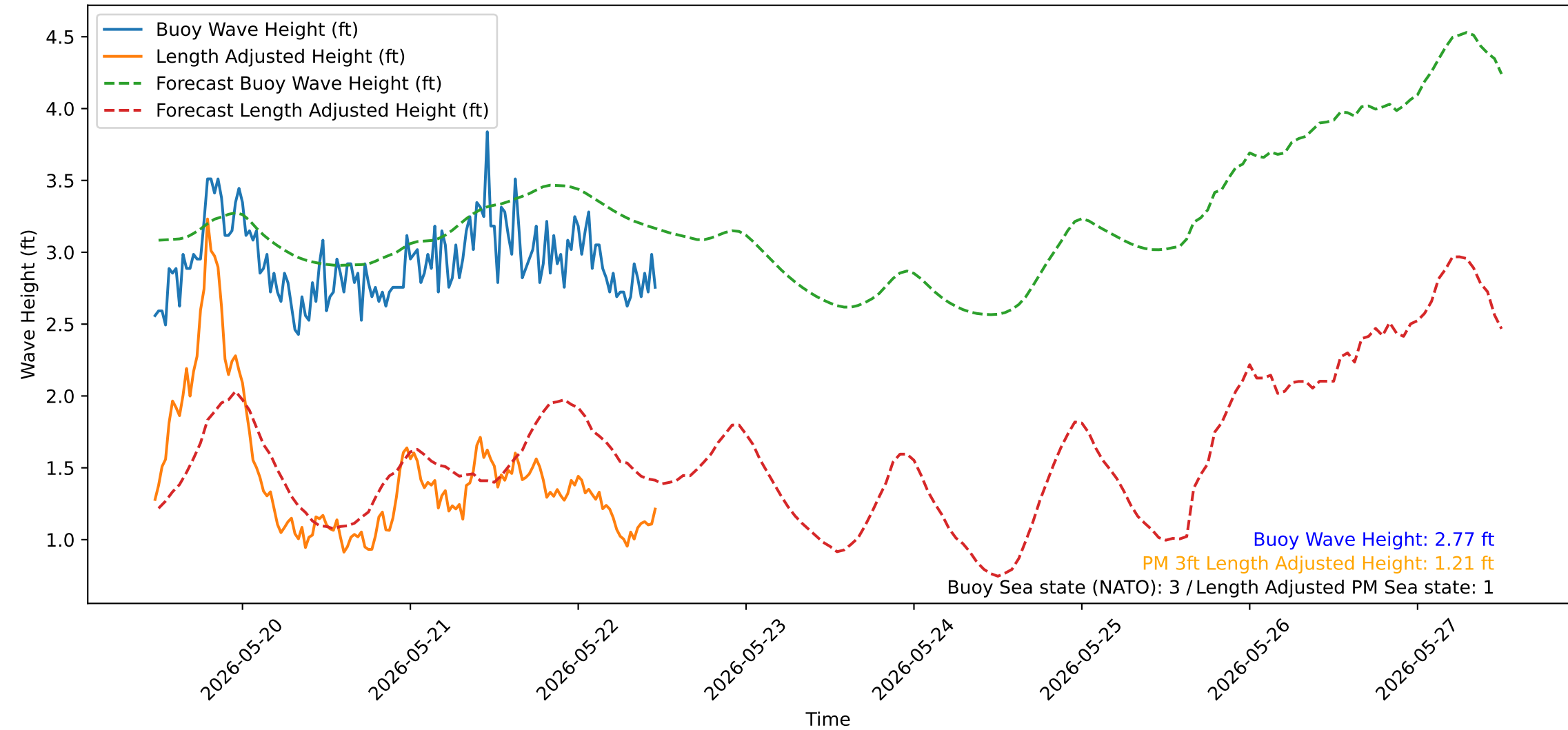
Wave Heights over Time for Oceanside Harbor at 2026-05-22 11:30:32
