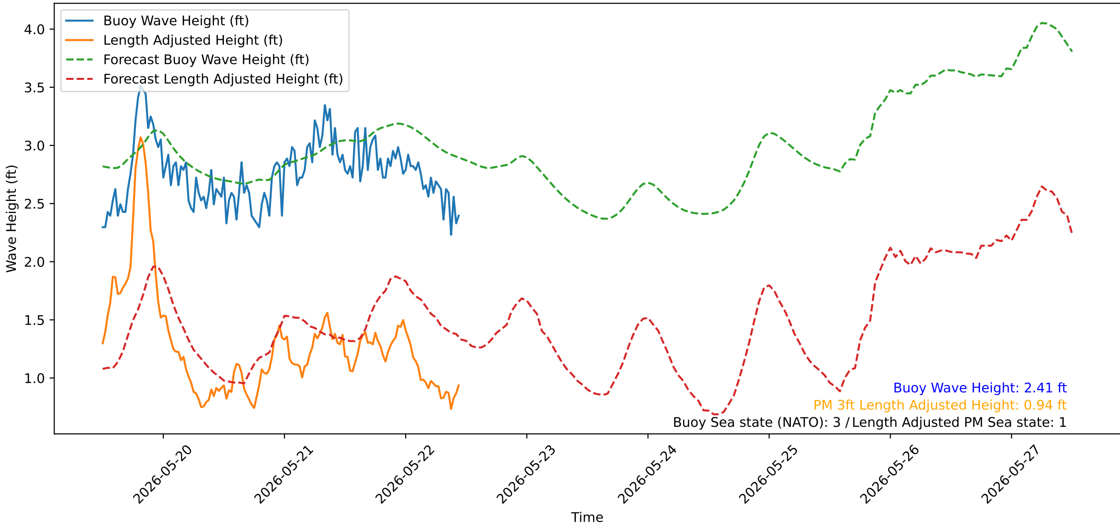
Wave Heights over Time for Red Beach at 2026-05-22 11:30:52
