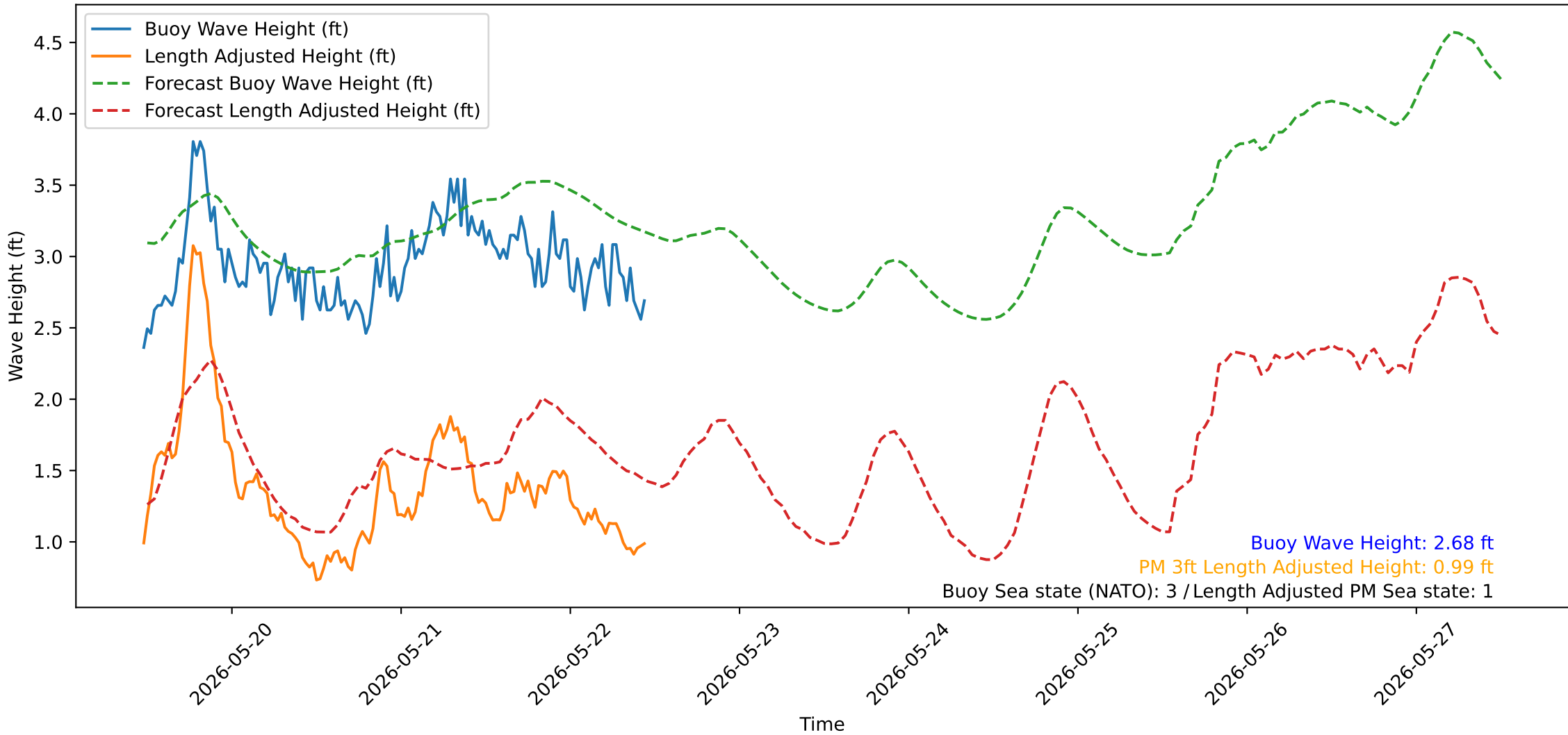
Wave Heights over Time for Green Beach at 2026-05-22 11:31:14
