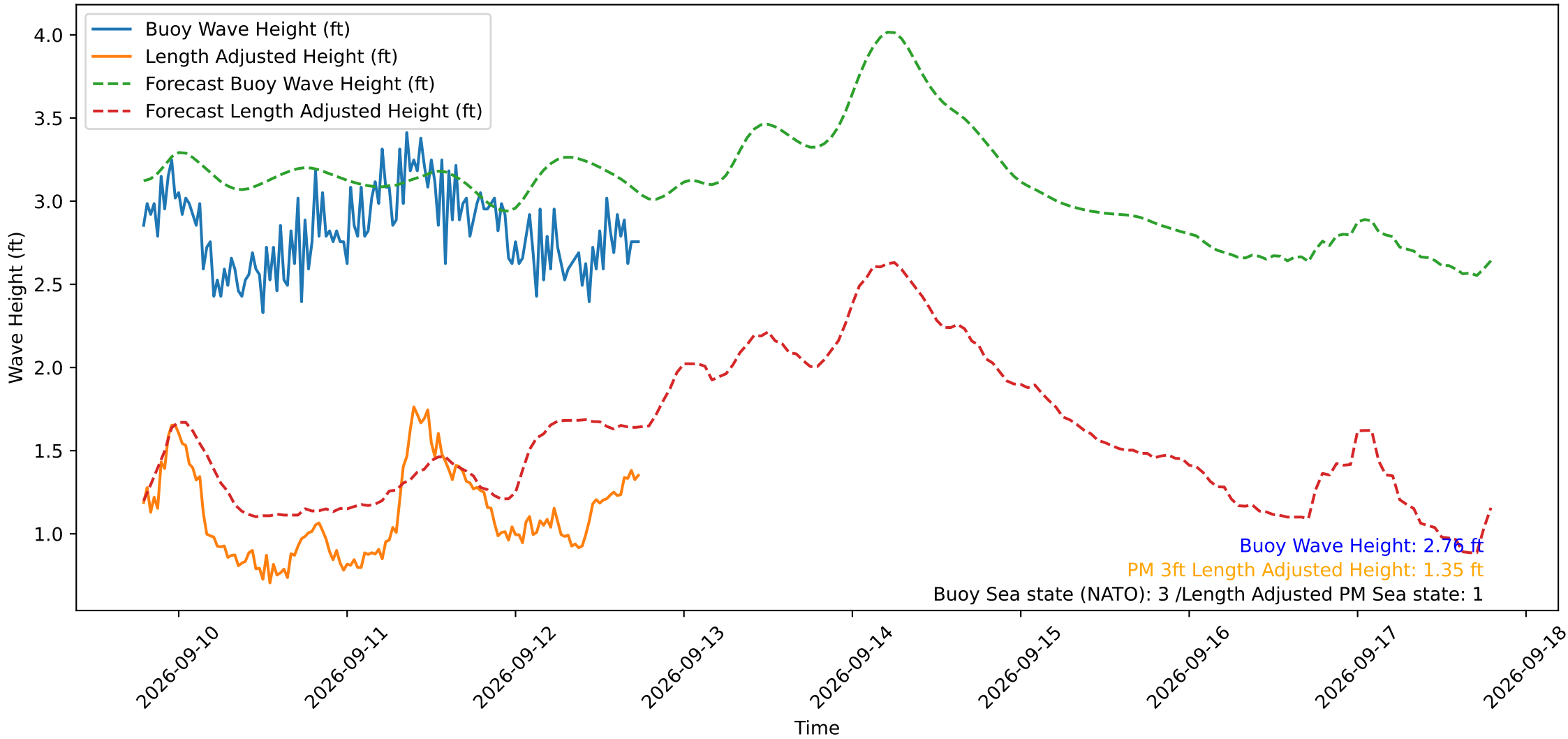
Wave Heights over Time for Red Beach at 2026-09-12 18:40:49
