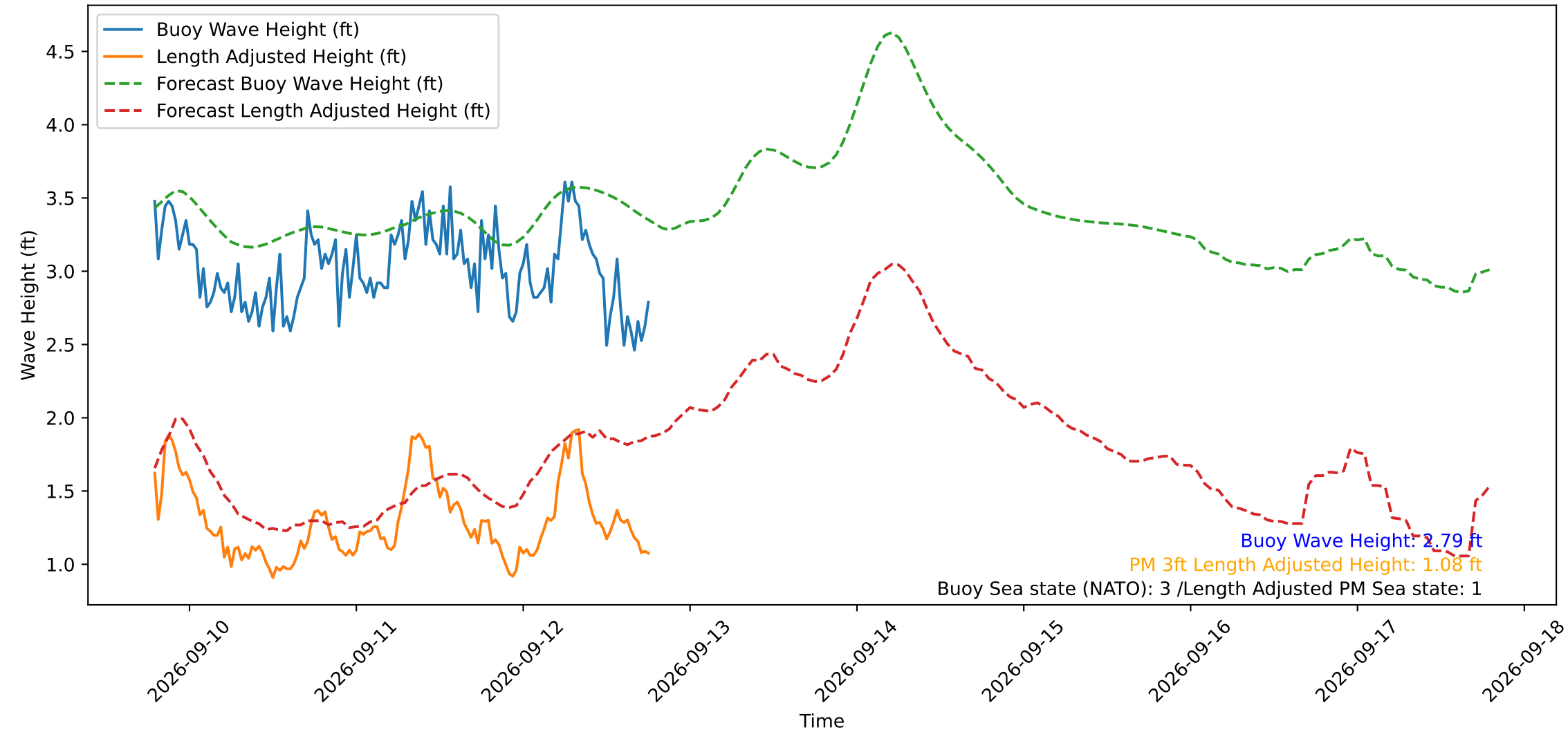
Wave Heights over Time for Green Beach at 2026-09-12 18:41:11
