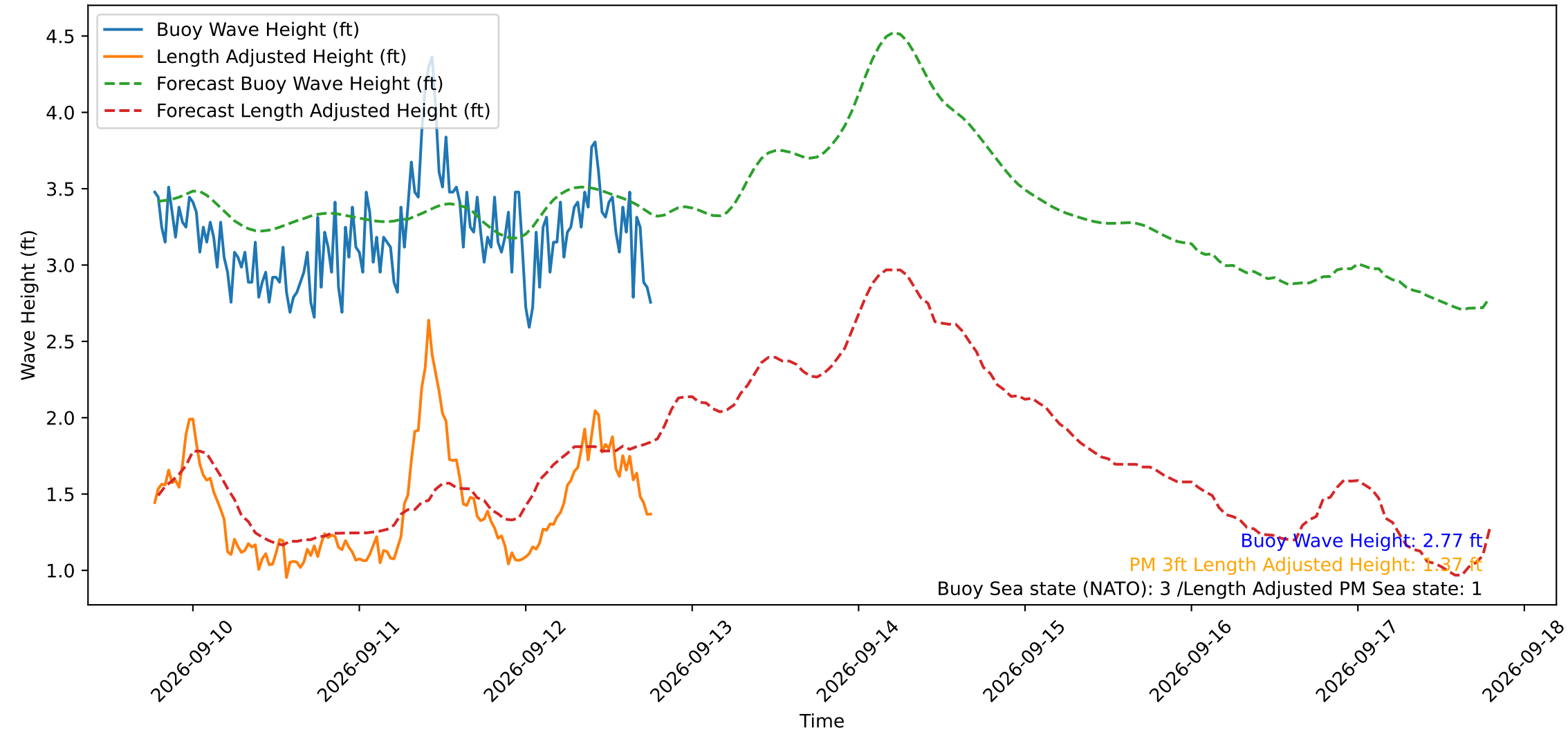
Wave Heights over Time for Oceanside Harbor at 2026-09-12 18:40:30
