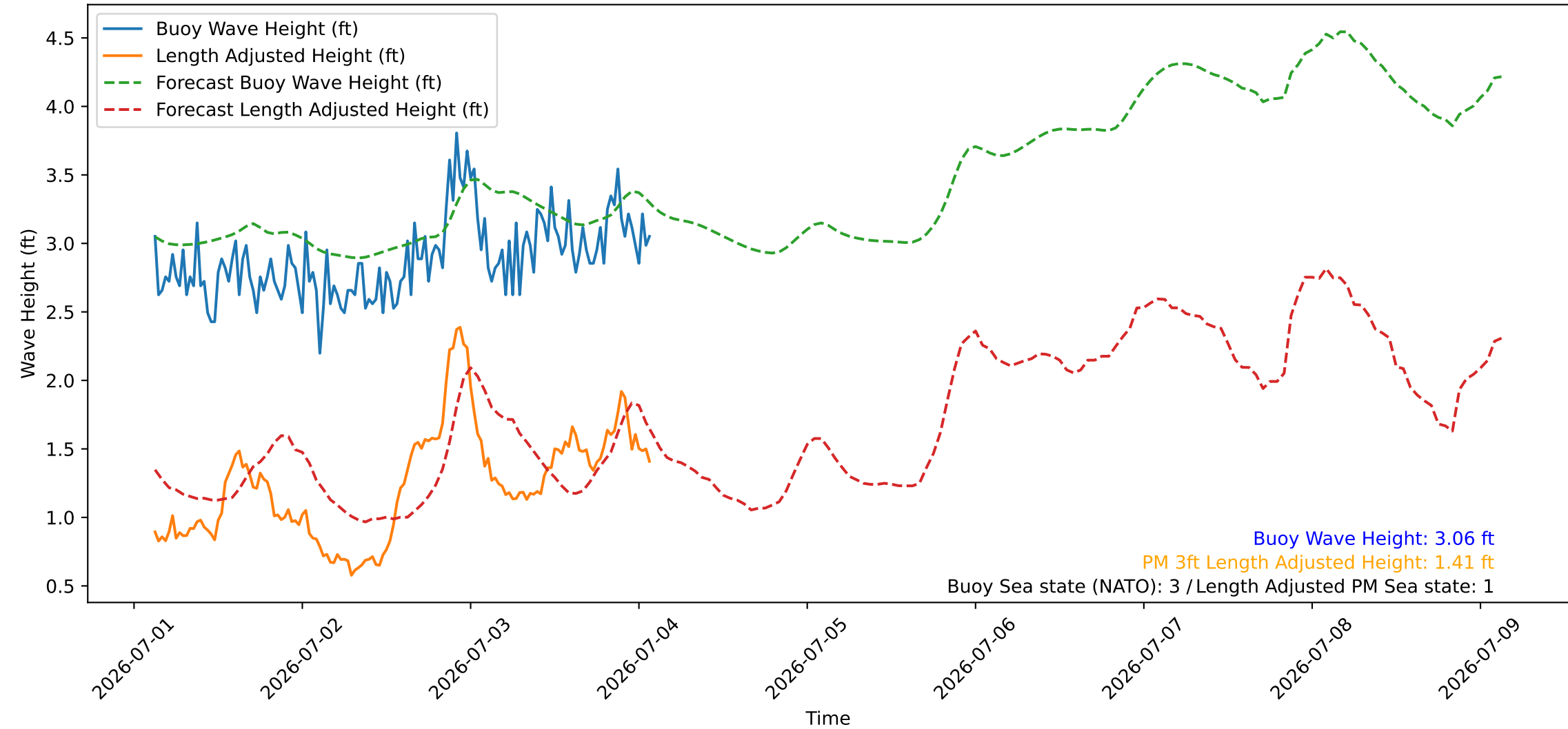
Wave Heights over Time for Red Beach at 2026-07-04 02:30:46
