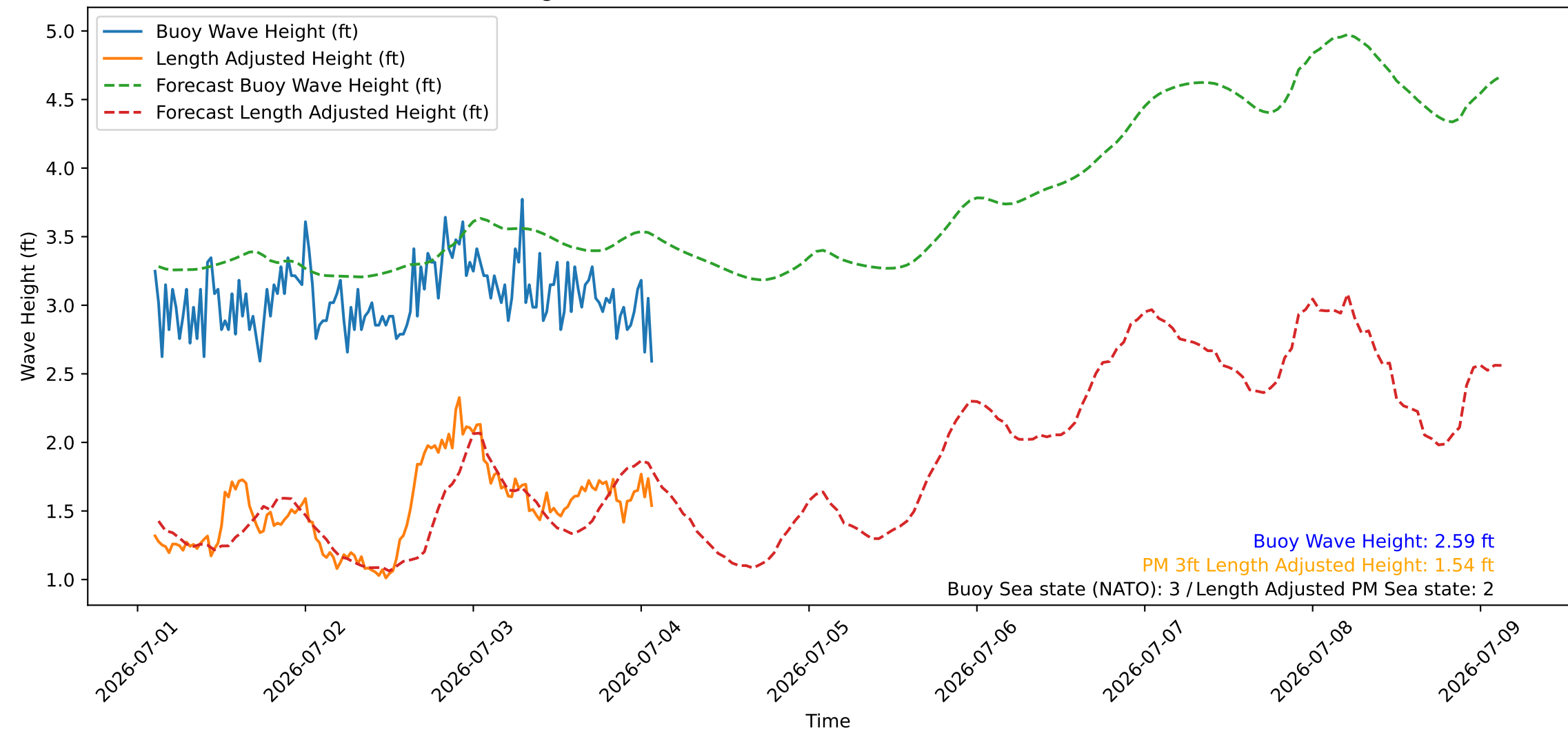
Wave Heights over Time for Oceanside Harbor at 2026-07-04 02:30:26
