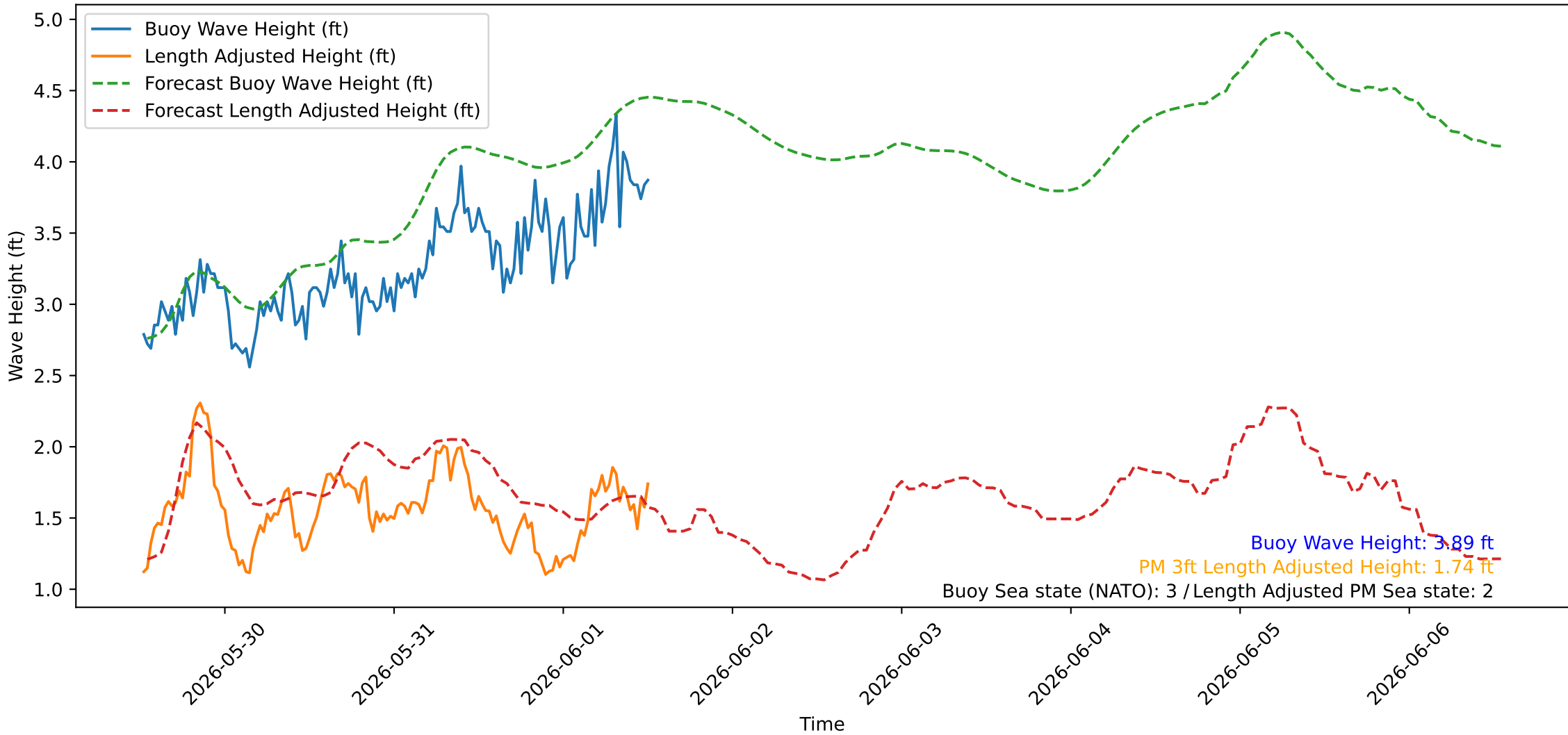
Wave Heights over Time for Green Beach at 2026-06-01 12:41:09
