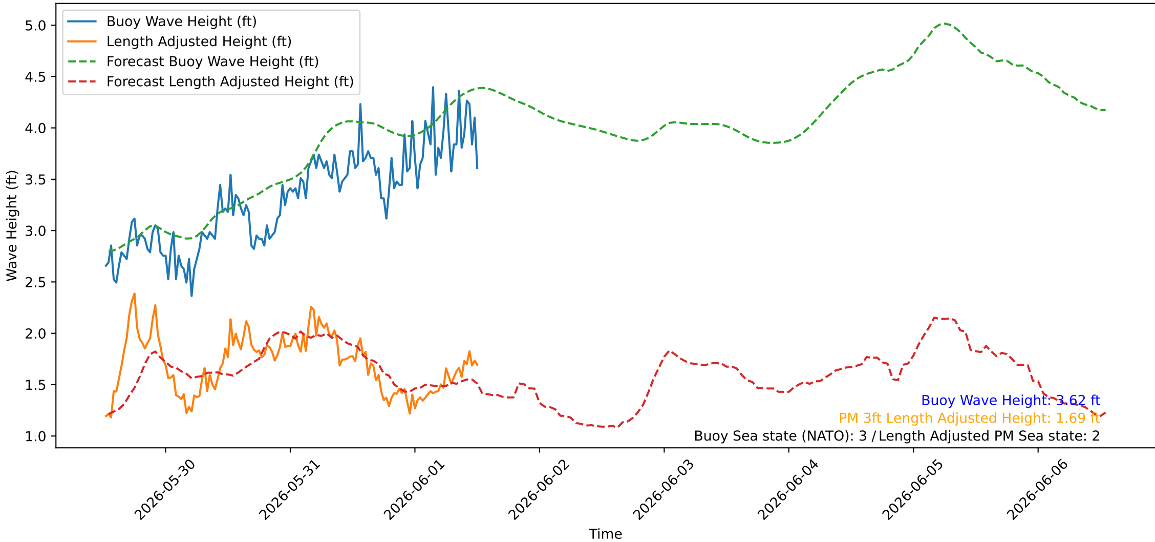
Wave Heights over Time for Oceanside Harbor at 2026-06-01 12:40:27
