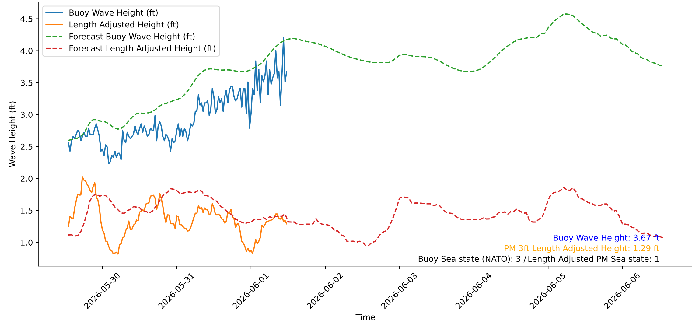
Wave Heights over Time for Red Beach at 2026-06-01 12:40:46
