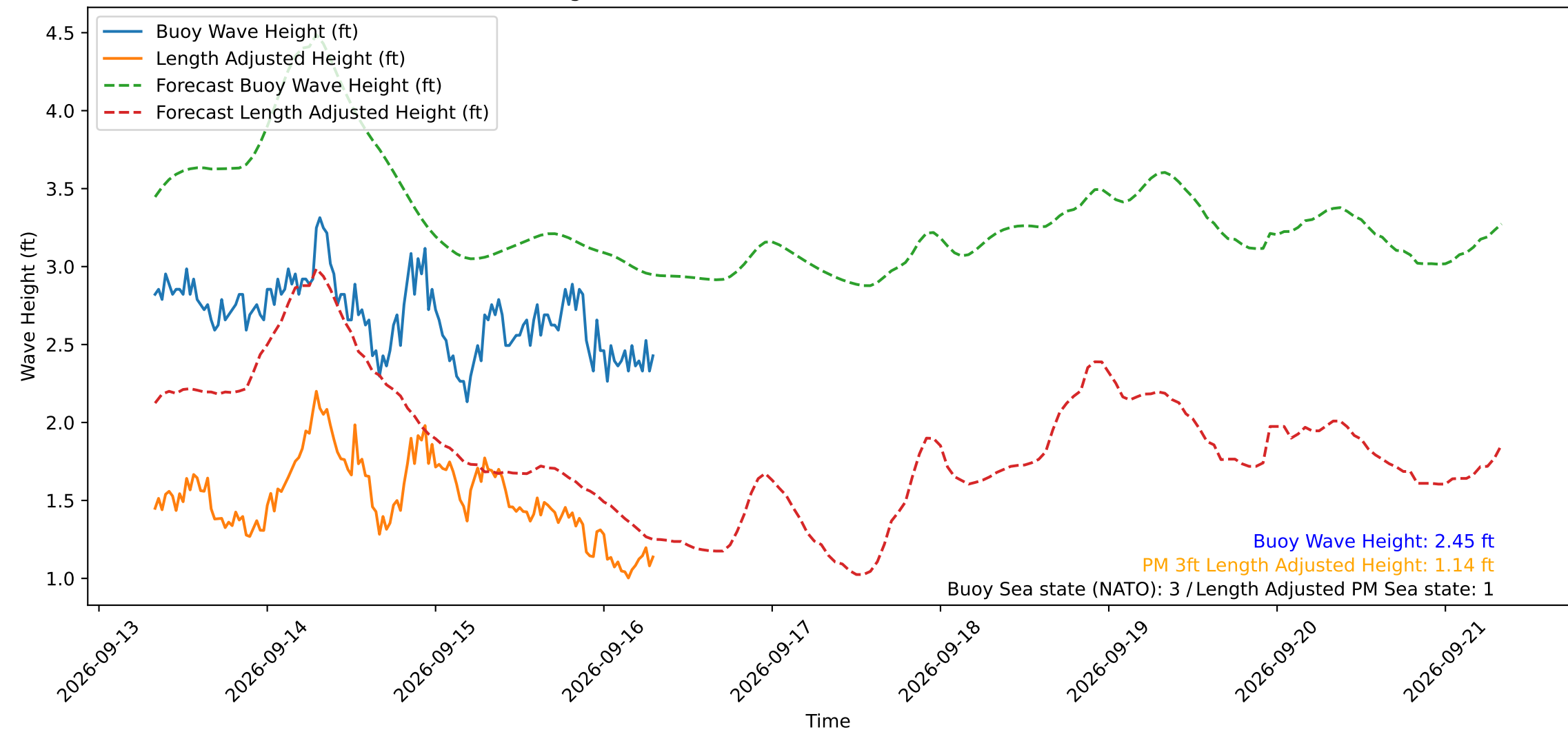
Wave Heights over Time for Green Beach at 2026-09-16 07:41:11
