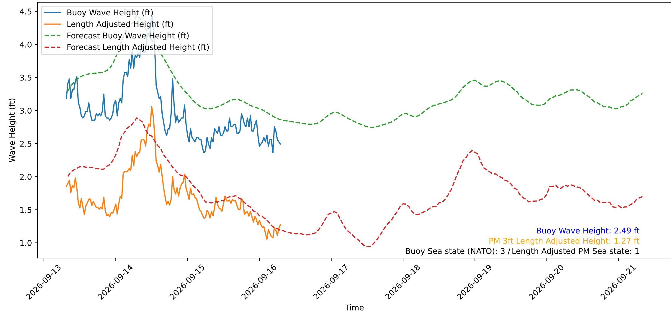
Wave Heights over Time for Oceanside Harbor at 2026-09-16 07:40:29
