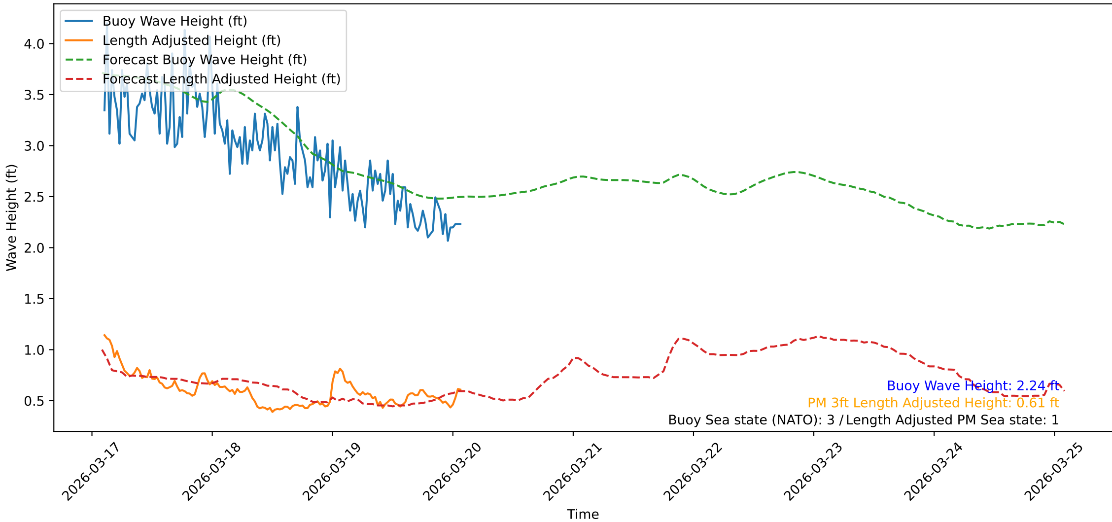
Wave Heights over Time for Green Beach at 2026-03-20 02:21:11
