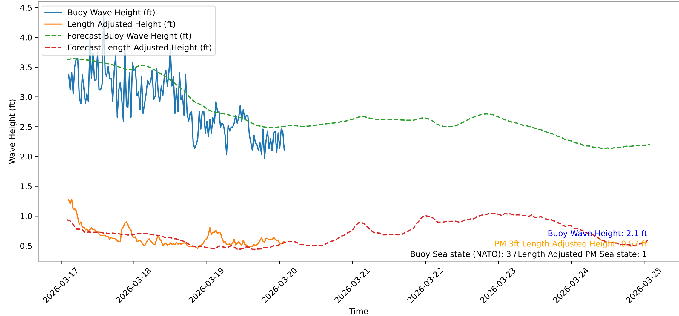
Wave Heights over Time for Oceanside Harbor at 2026-03-20 02:20:32
