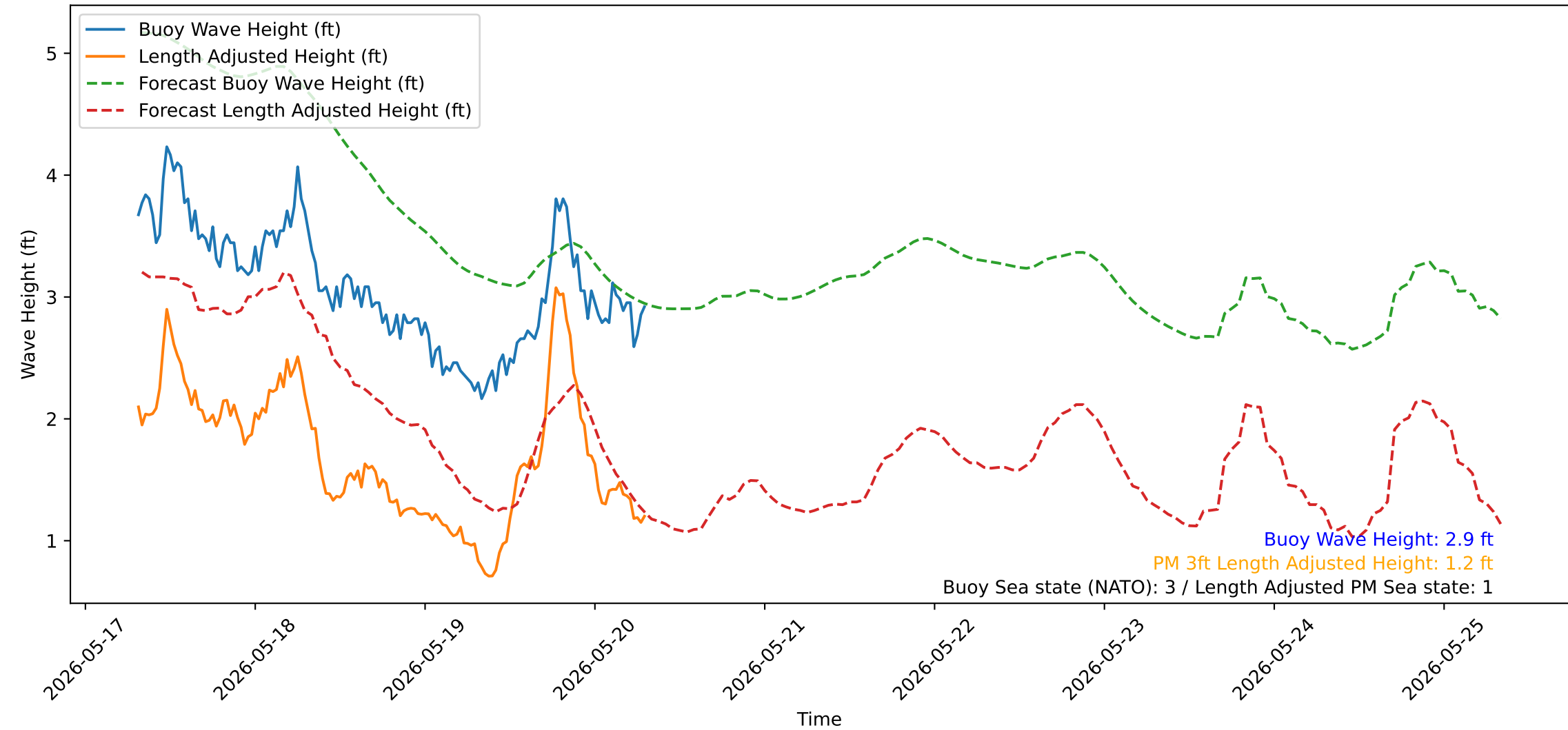
Wave Heights over Time for Green Beach at 2026-05-20 07:41:13
