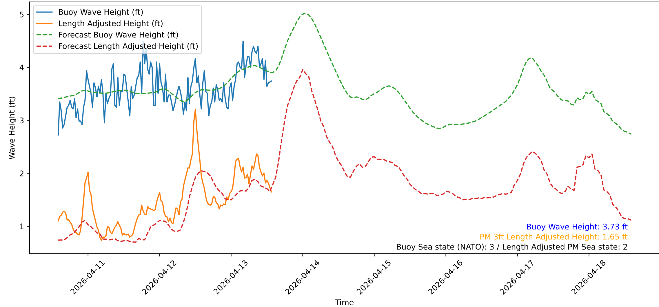
Wave Heights over Time for Green Beach at 2026-04-13 14:11:13
