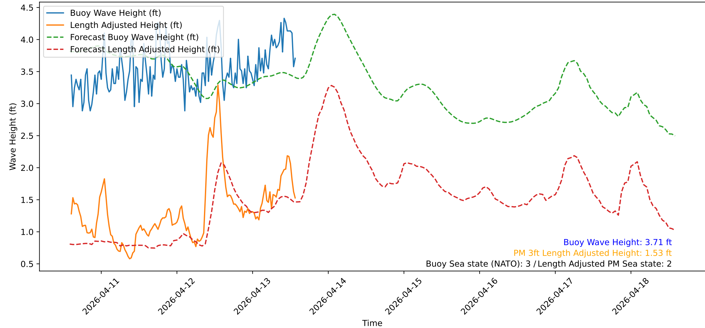
Wave Heights over Time for Red Beach at 2026-04-13 14:10:50
