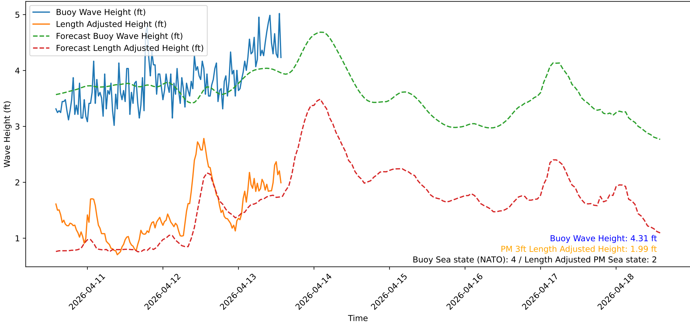
Wave Heights over Time for Oceanside Harbor at 2026-04-13 14:10:31
