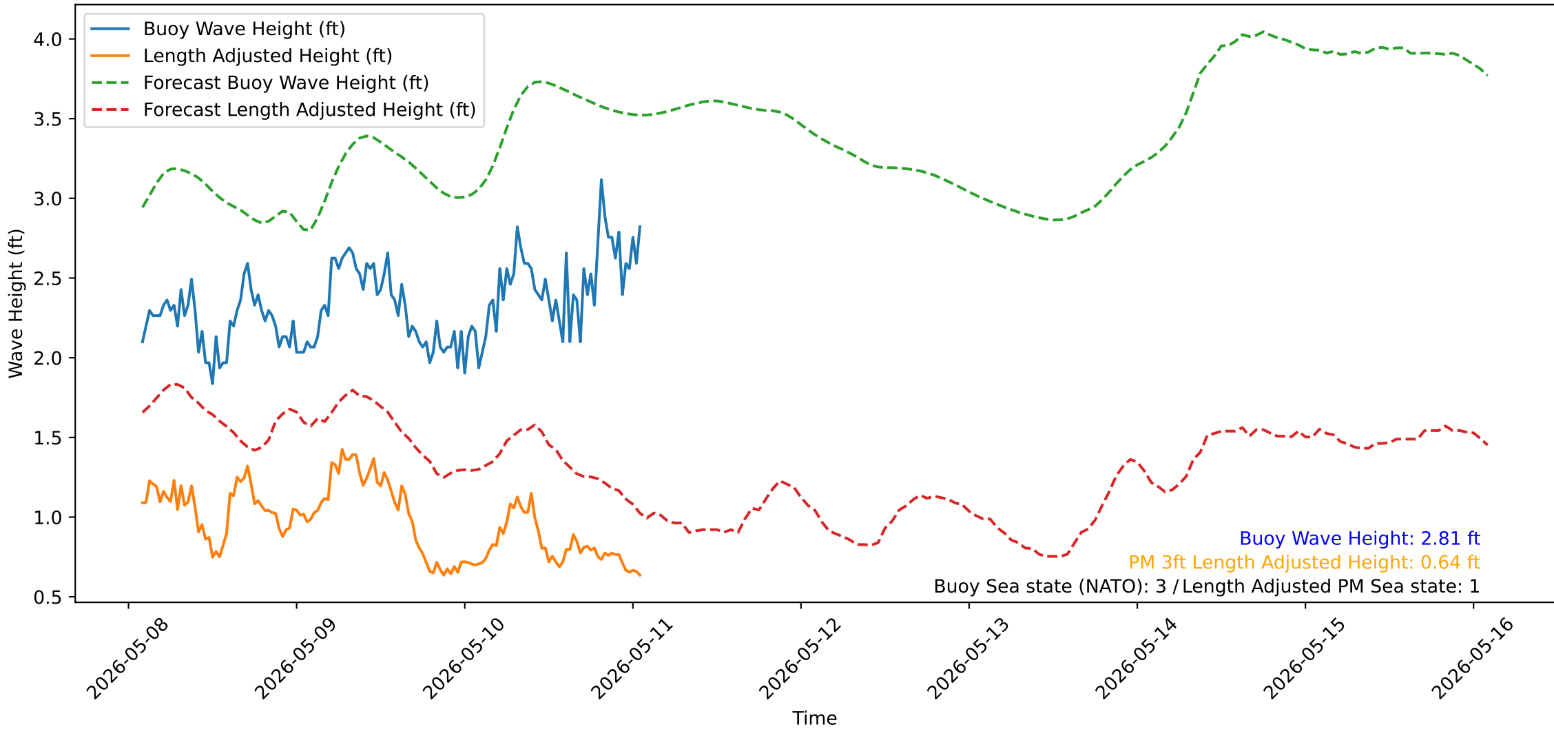
Wave Heights over Time for Green Beach at 2026-05-11 01:51:14
