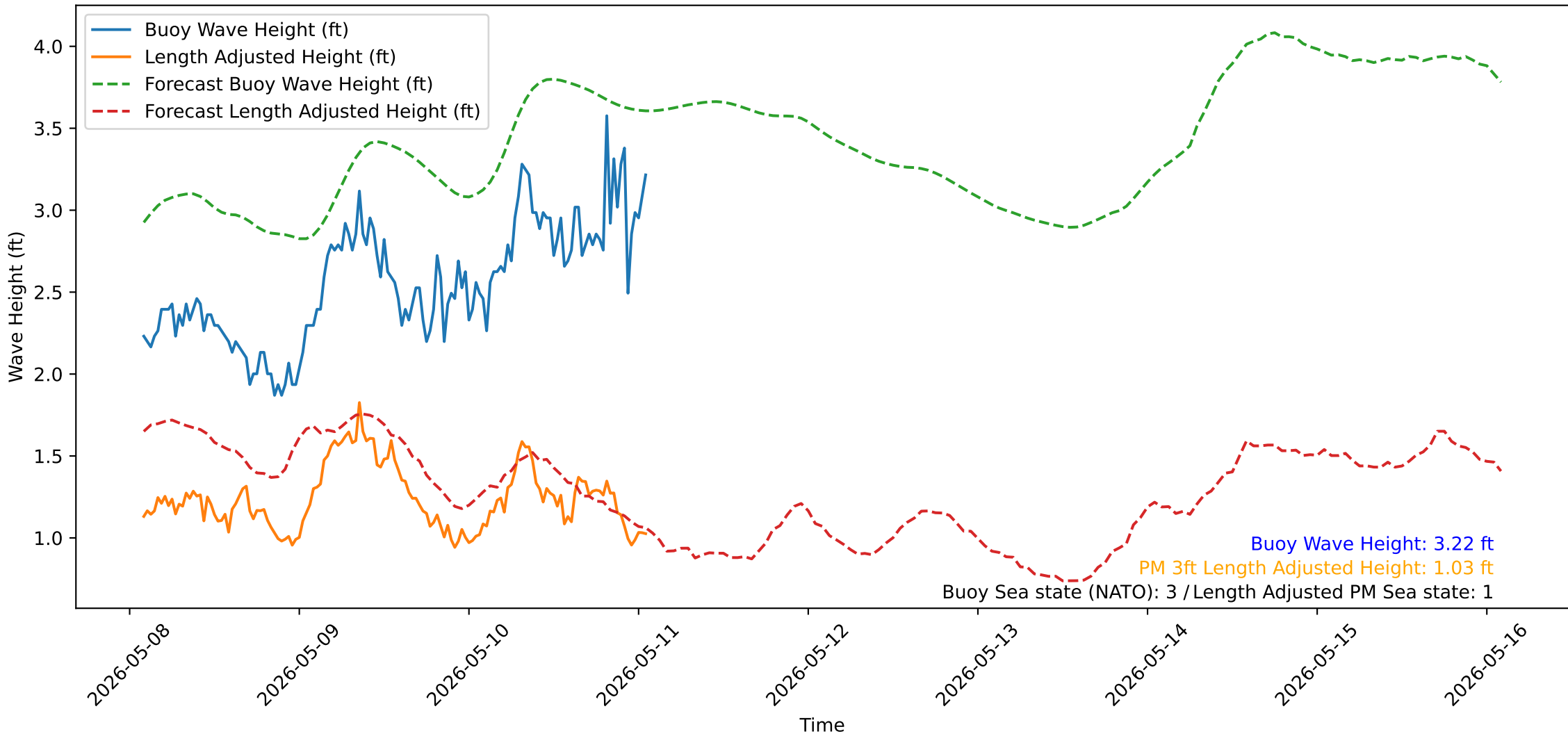
Wave Heights over Time for Oceanside Harbor at 2026-05-11 01:50:32
