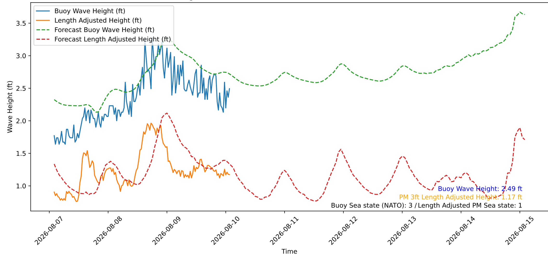
Wave Heights over Time for Oceanside Harbor at 2026-08-10 02:00:26
