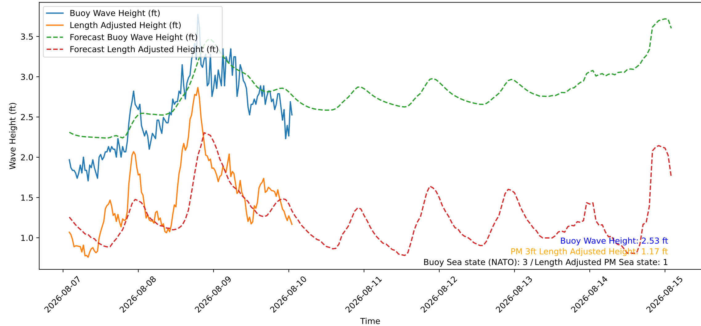
Wave Heights over Time for Green Beach at 2026-08-10 02:01:09
