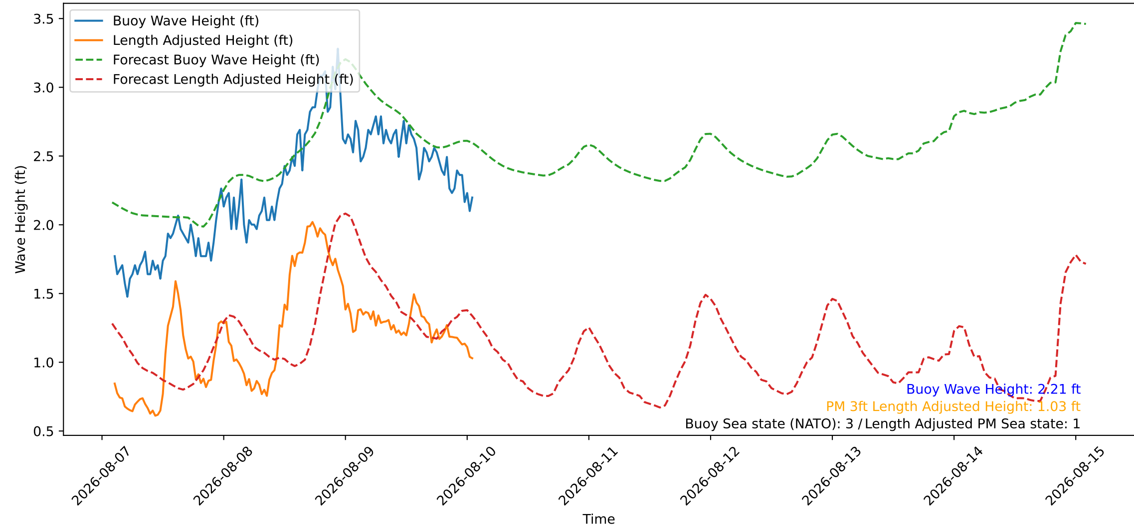
Wave Heights over Time for Red Beach at 2026-08-10 02:00:46
