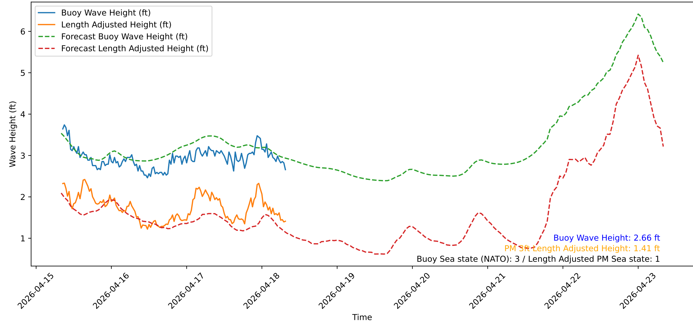
Wave Heights over Time for Green Beach at 2026-04-18 08:21:13
