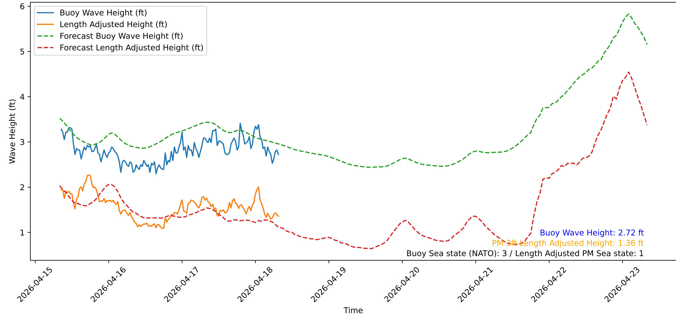
Wave Heights over Time for Oceanside Harbor at 2026-04-18 08:20:31
