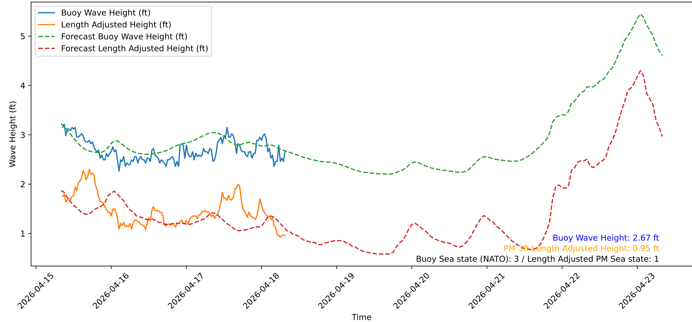
Wave Heights over Time for Red Beach at 2026-04-18 08:20:51
