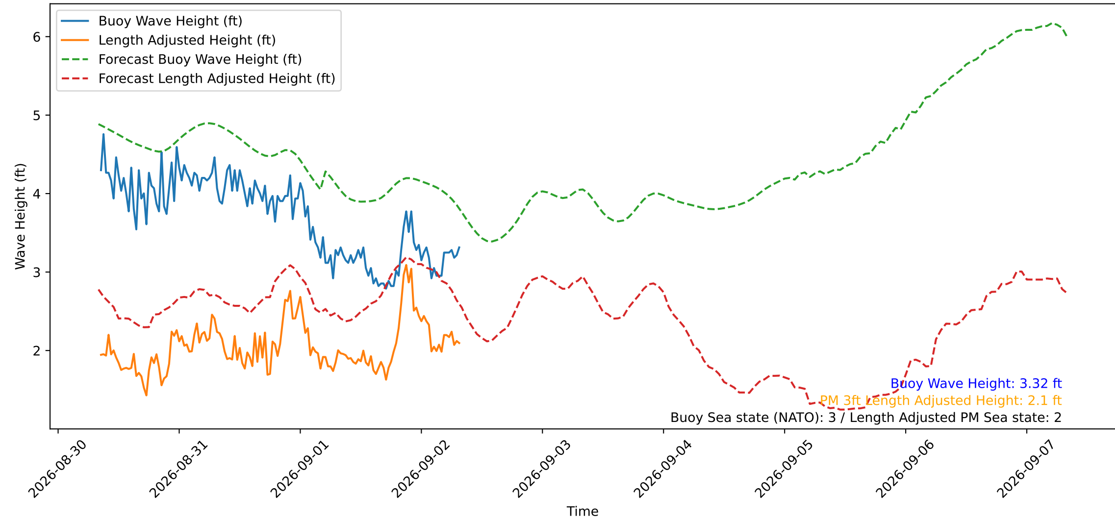
Wave Heights over Time for Green Beach at 2026-09-02 08:21:15
