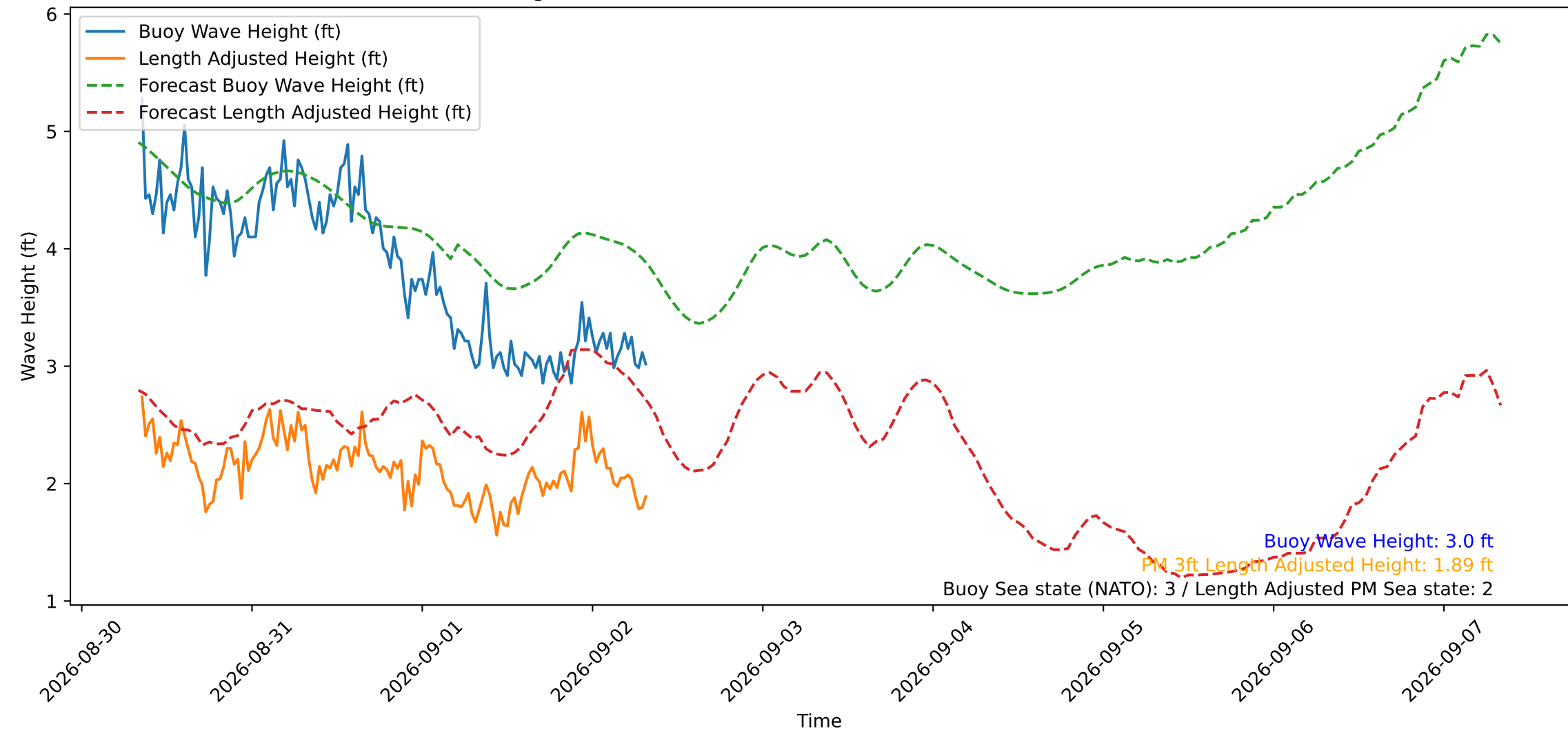
Wave Heights over Time for Oceanside Harbor at 2026-09-02 08:20:30
