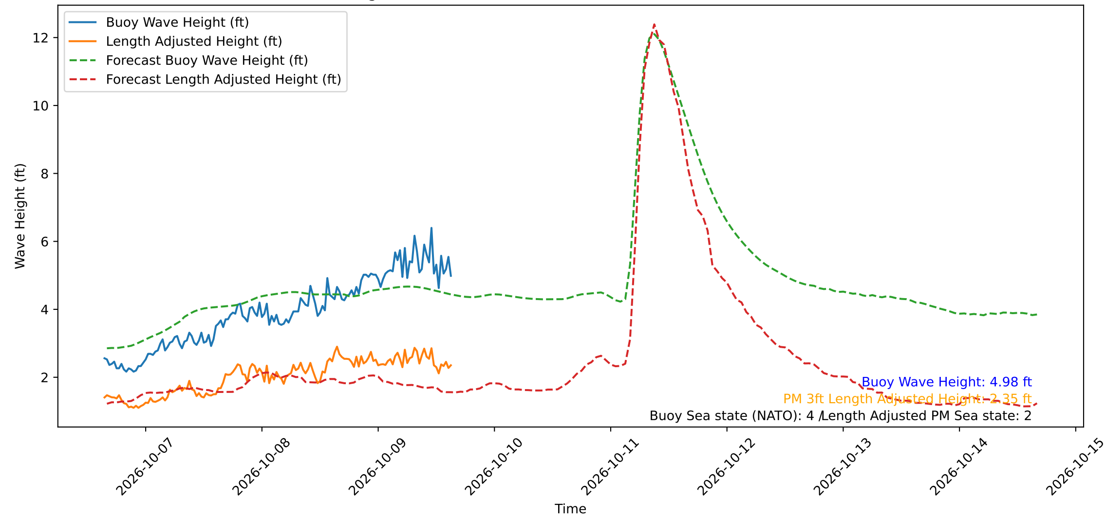
Wave Heights over Time for Oceanside Harbor at 2026-10-09 15:30:30
