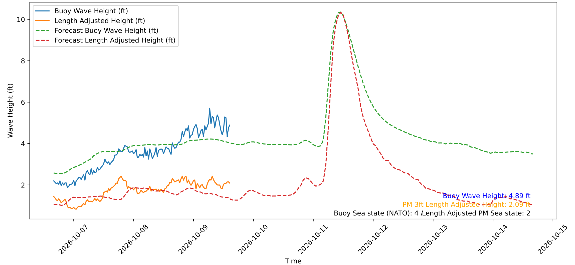
Wave Heights over Time for Red Beach at 2026-10-09 15:30:49
