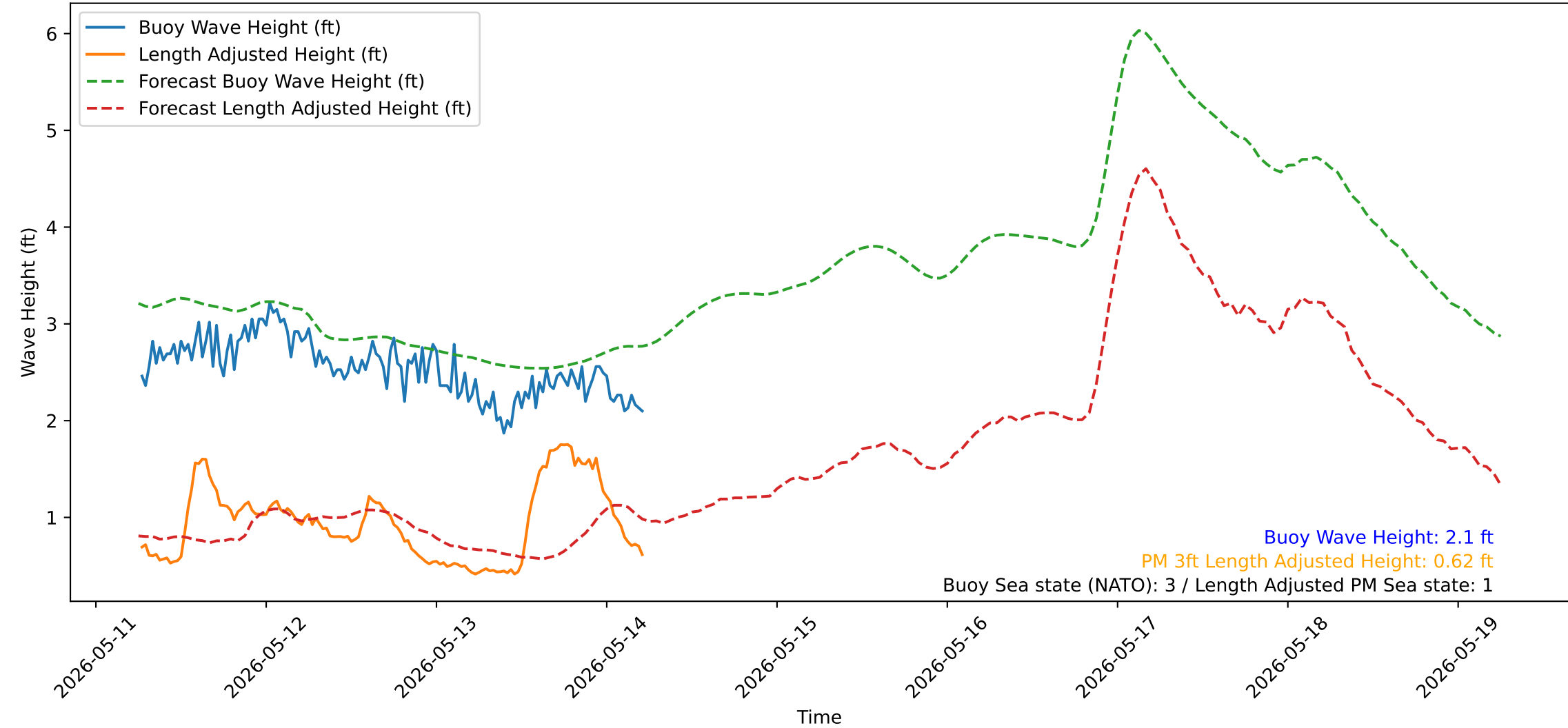
Wave Heights over Time for Red Beach at 2026-05-14 06:00:51
