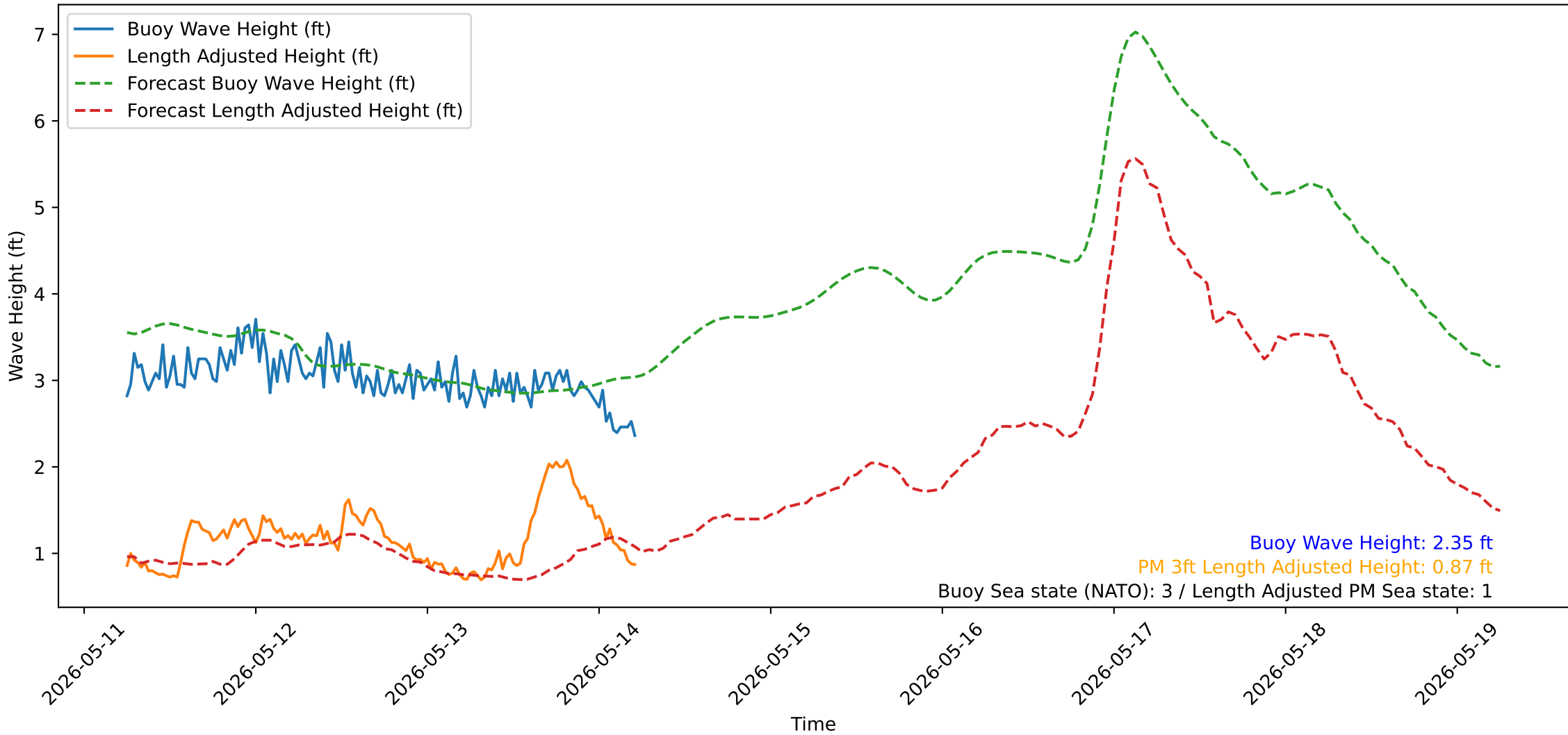
Wave Heights over Time for Oceanside Harbor at 2026-05-14 06:00:32
