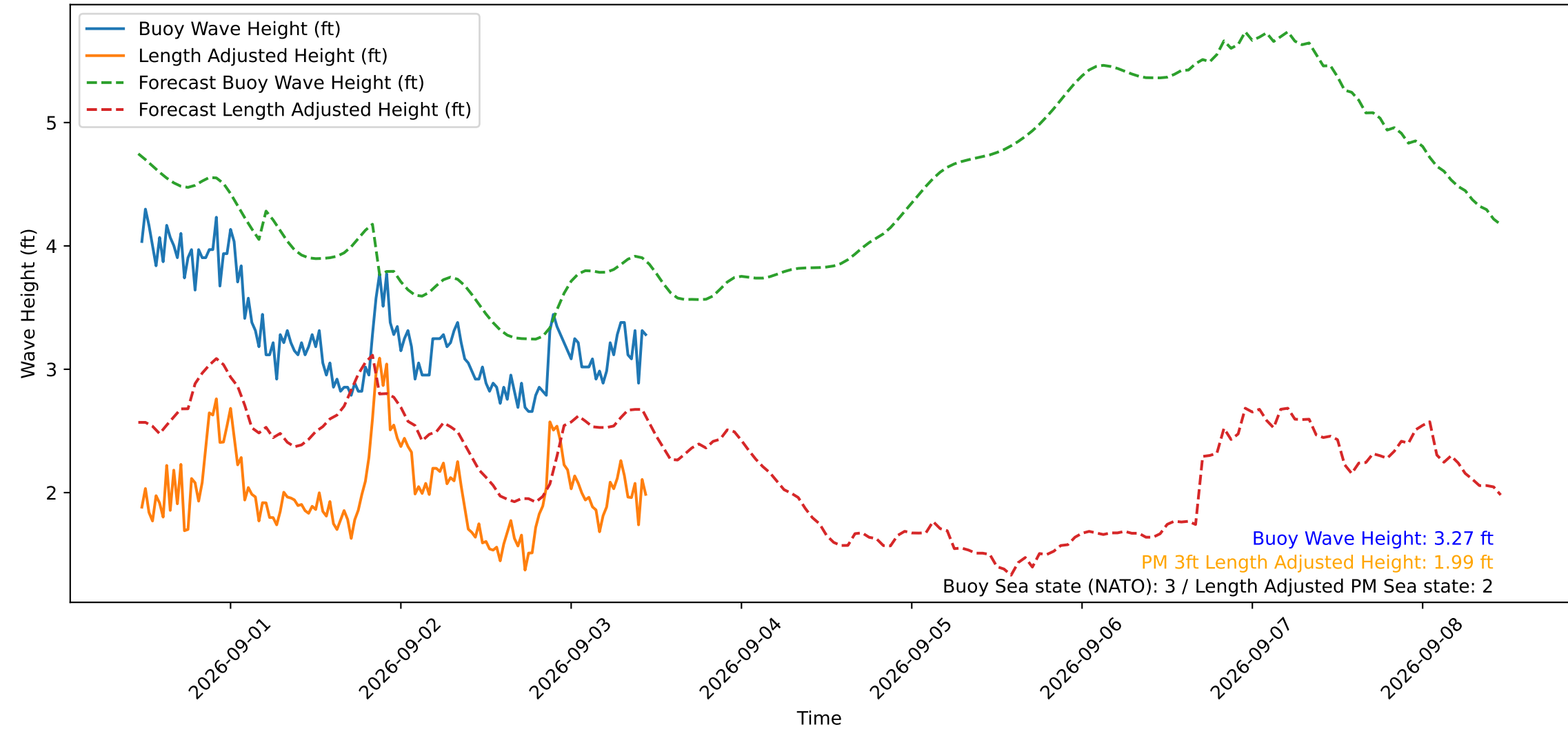
Wave Heights over Time for Green Beach at 2026-09-03 11:11:13
