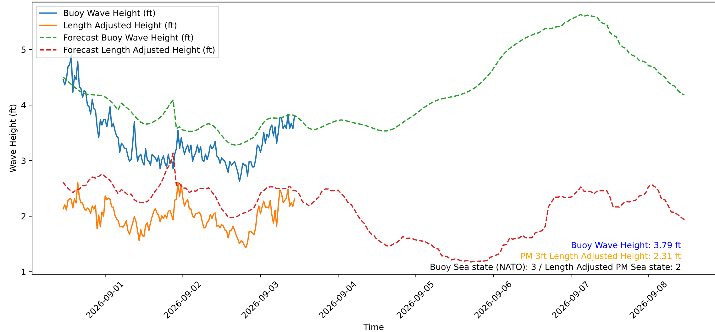
Wave Heights over Time for Oceanside Harbor at 2026-09-03 11:10:30
