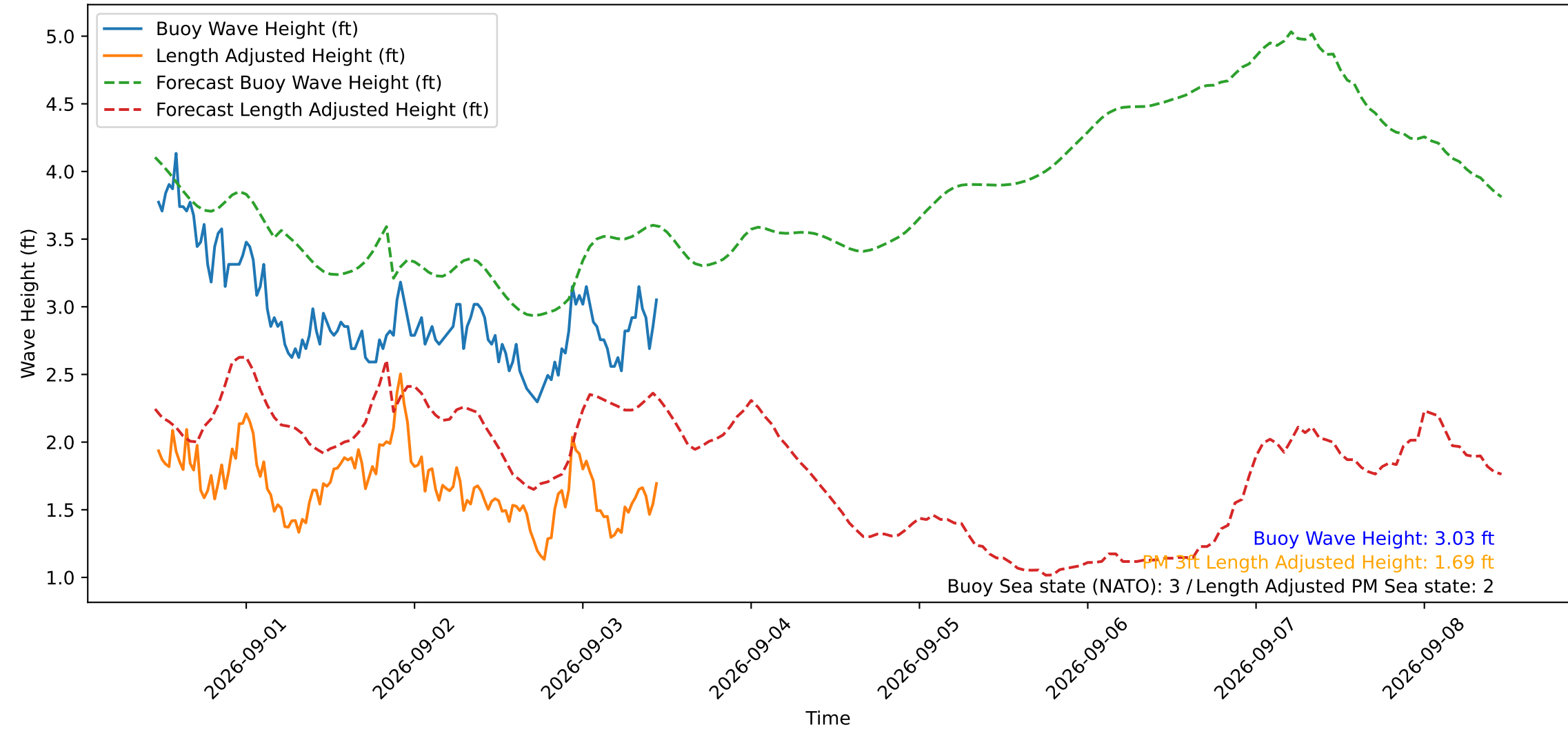
Wave Heights over Time for Red Beach at 2026-09-03 11:10:50
