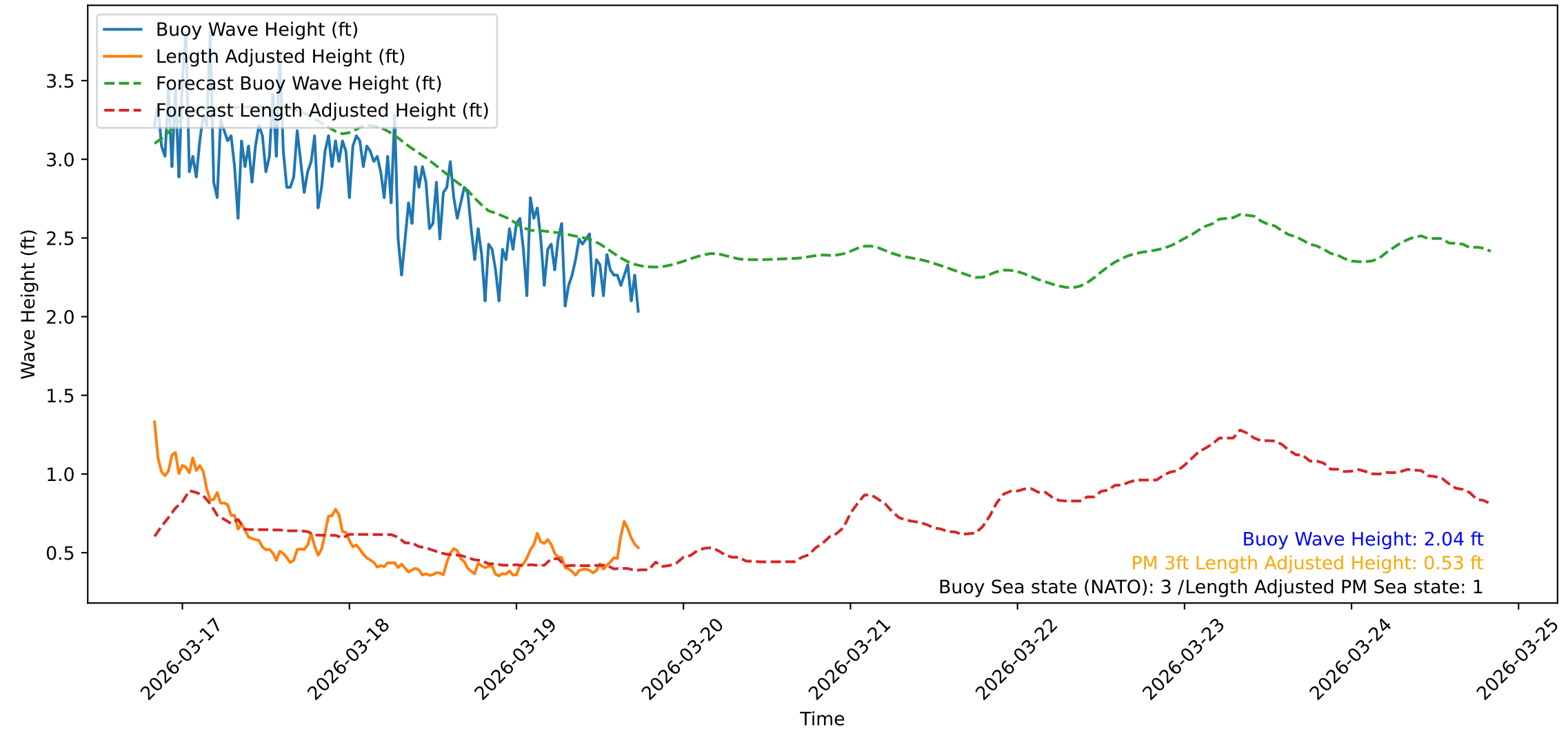
Wave Heights over Time for Red Beach at 2026-03-19 19:30:48
