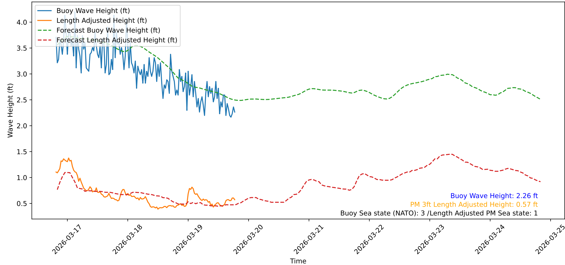
Wave Heights over Time for Green Beach at 2026-03-19 19:31:10
