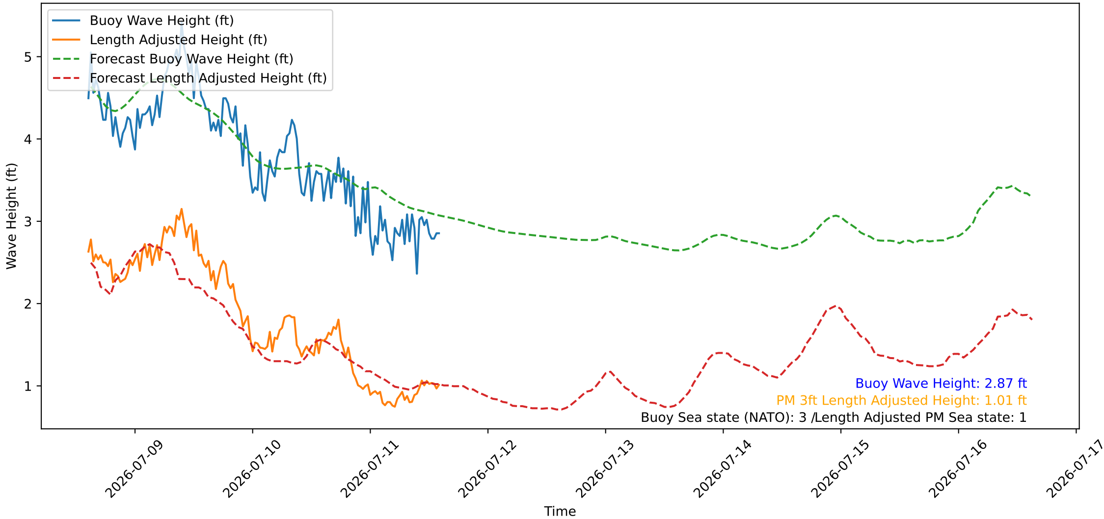
Wave Heights over Time for Oceanside Harbor at 2026-07-11 14:40:26
