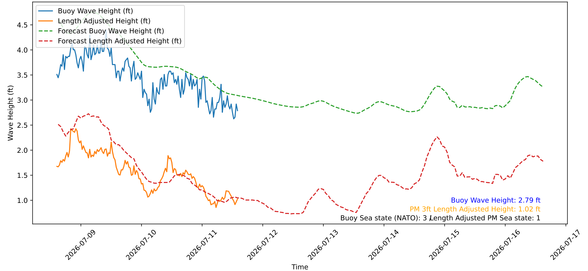
Wave Heights over Time for Green Beach at 2026-07-11 14:41:08
