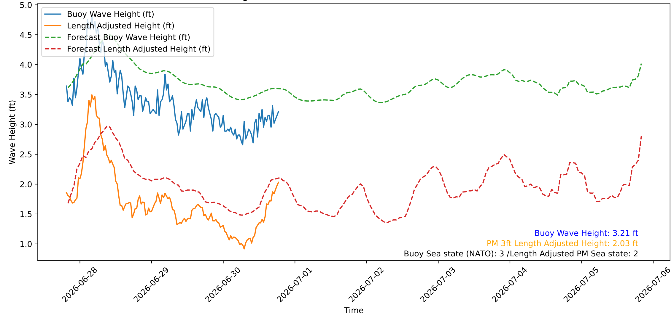
Wave Heights over Time for Green Beach at 2026-06-30 19:31:08
