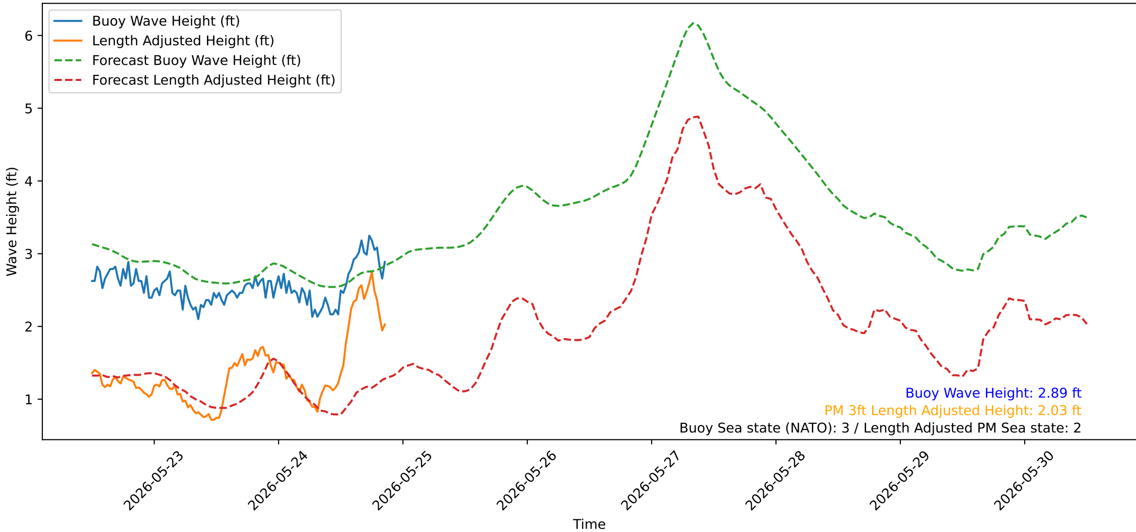
Wave Heights over Time for Oceanside Harbor at 2026-05-25 11:50:30
