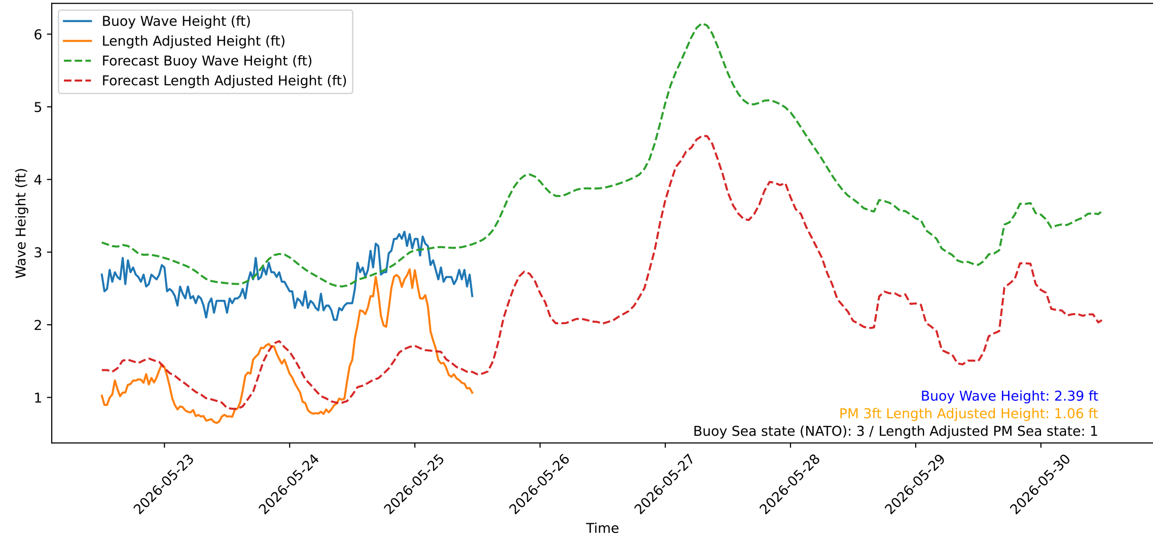
Wave Heights over Time for Green Beach at 2026-05-25 11:51:14
