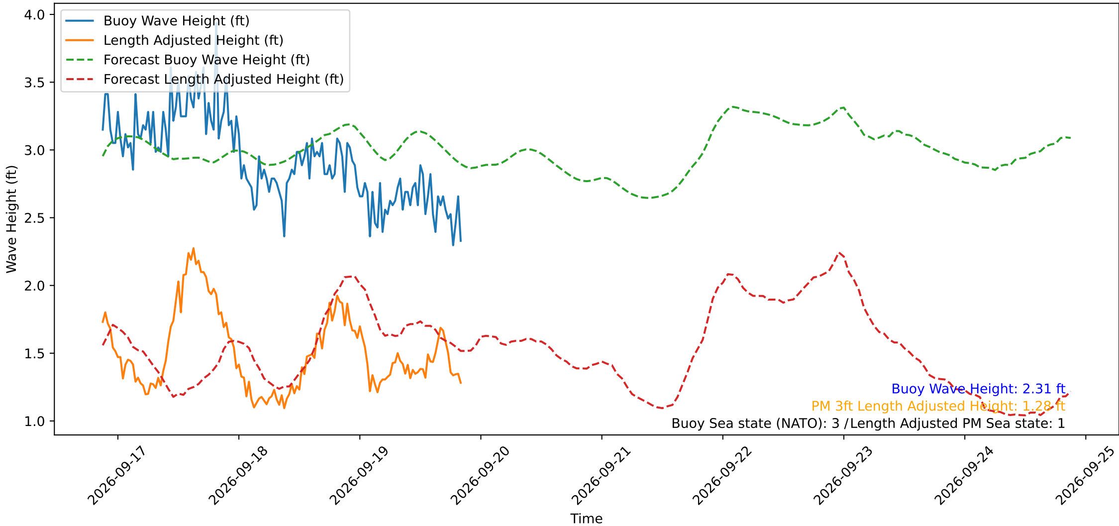
Wave Heights over Time for Oceanside Harbor at 2026-09-19 21:00:30
