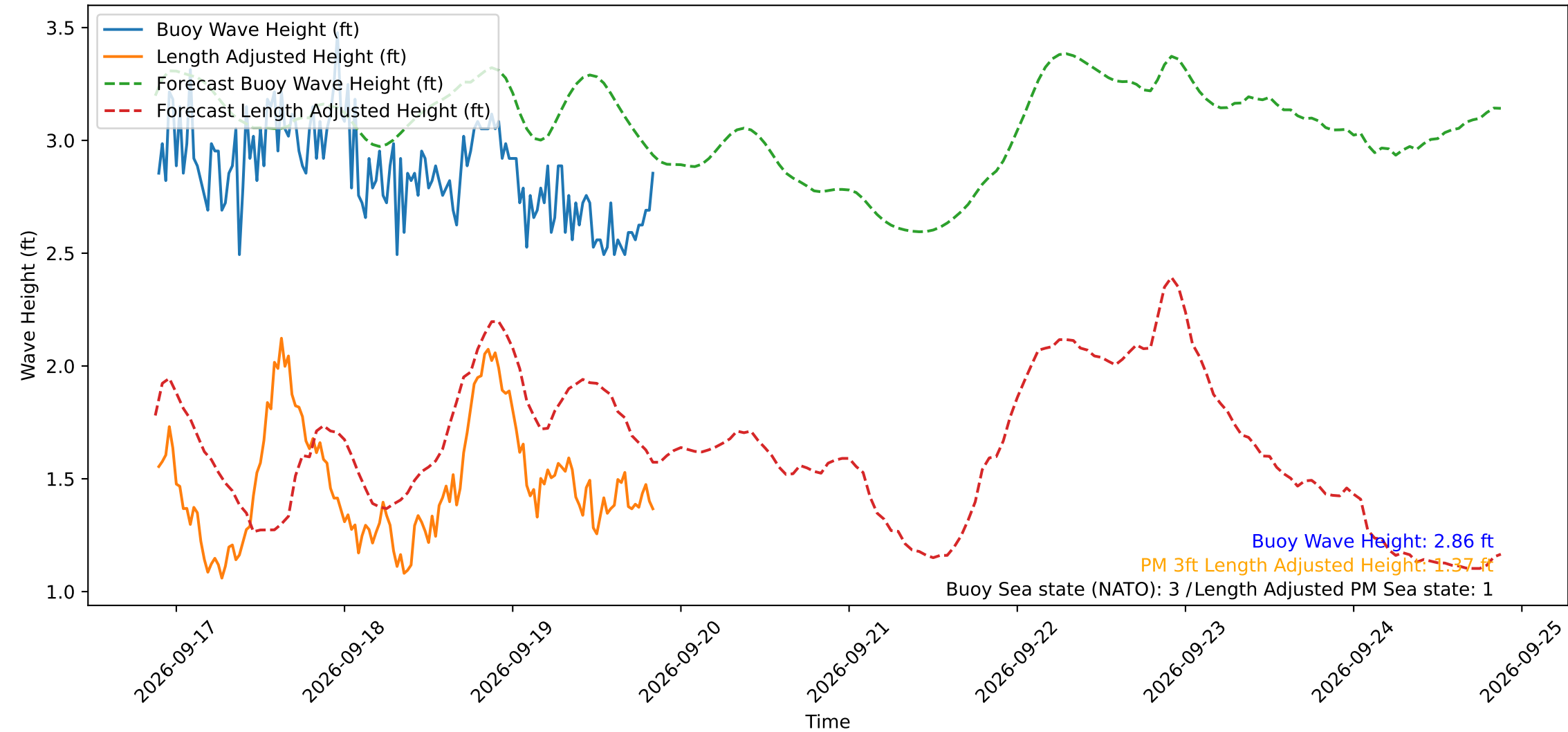
Wave Heights over Time for Green Beach at 2026-09-19 21:01:12
