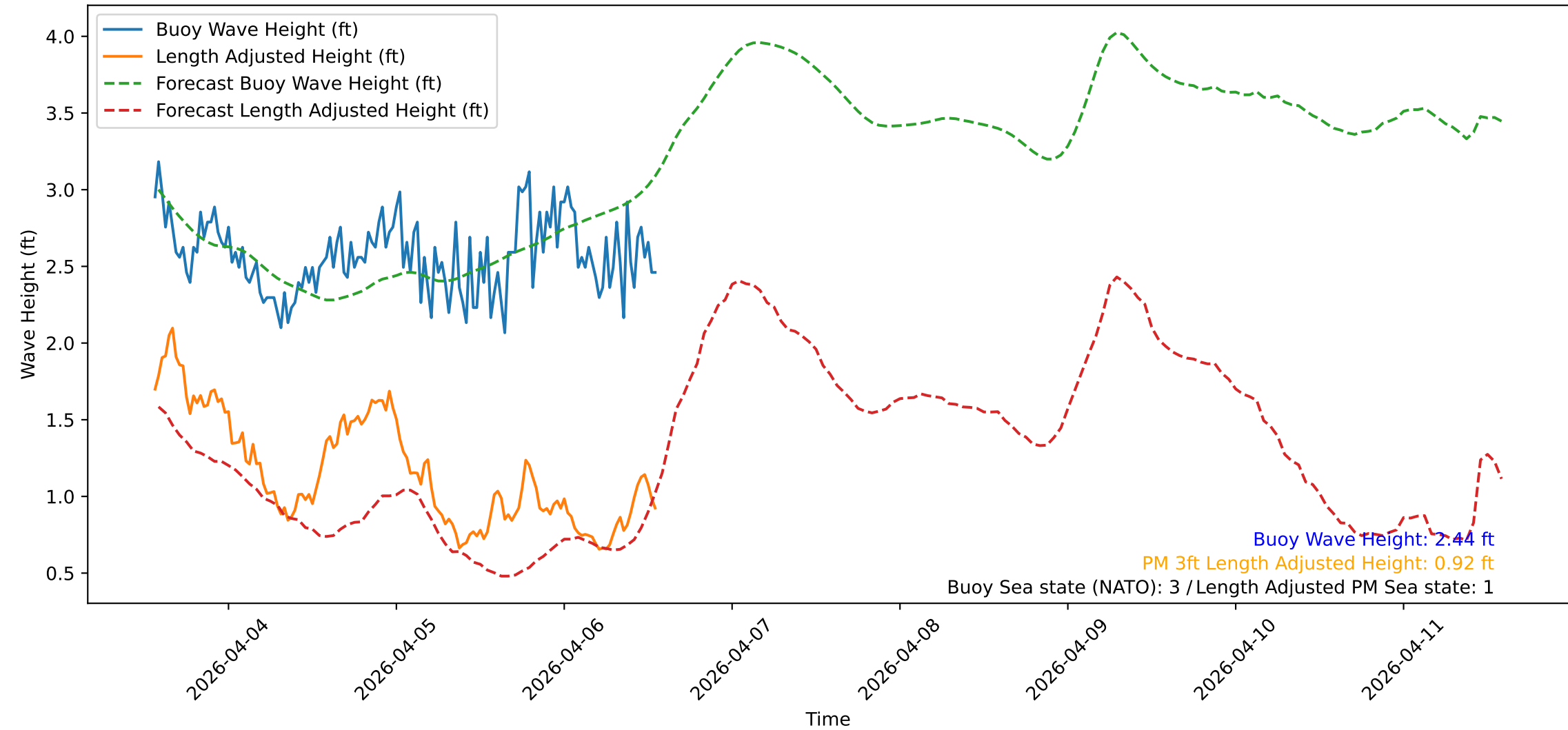
Wave Heights over Time for Oceanside Harbor at 2026-04-06 13:30:31
