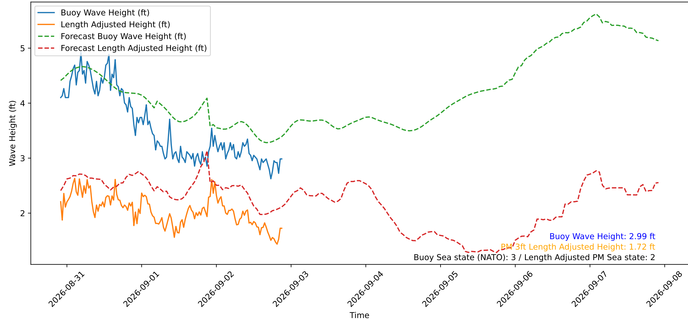
Wave Heights over Time for Oceanside Harbor at 2026-09-02 21:50:29
