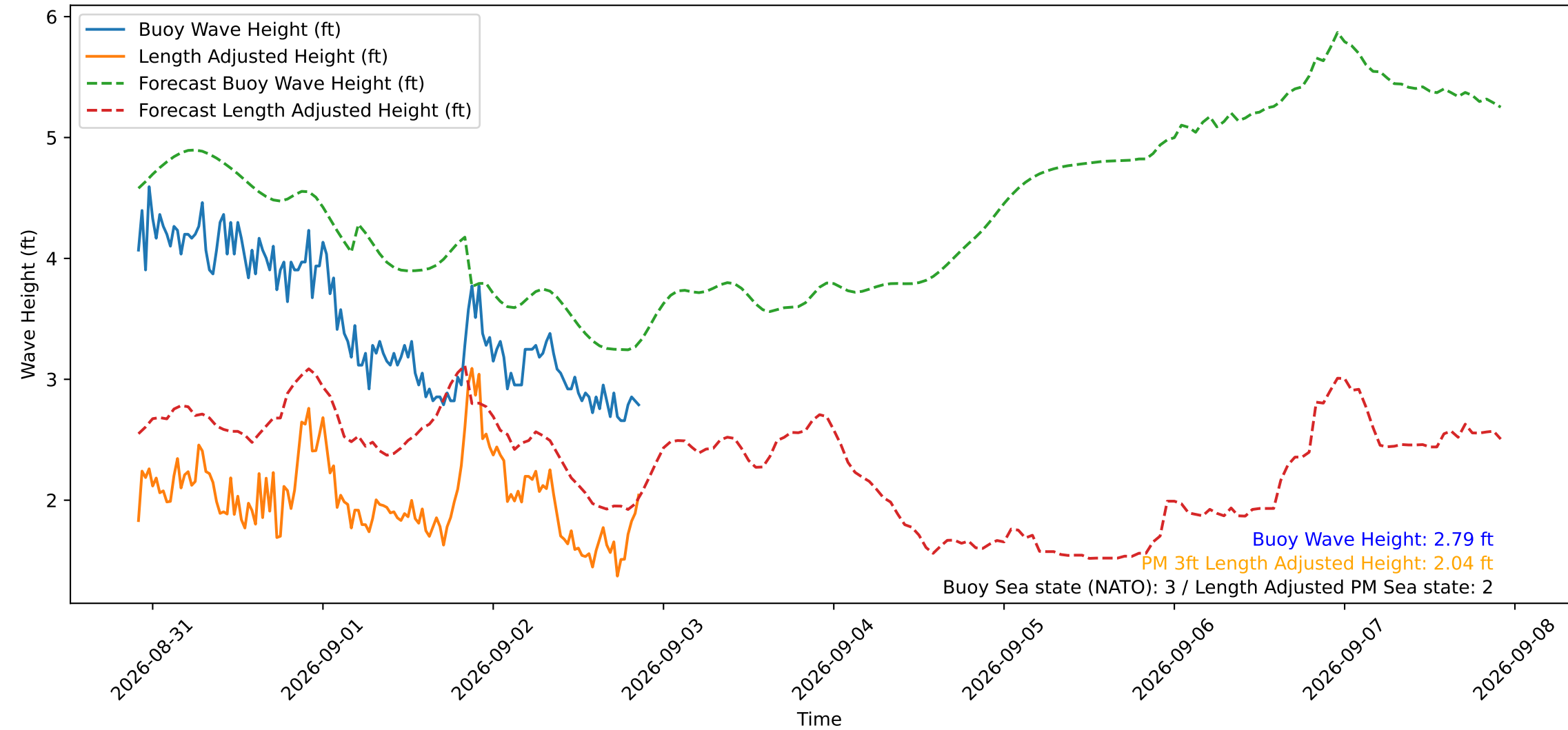
Wave Heights over Time for Green Beach at 2026-09-02 21:51:14
