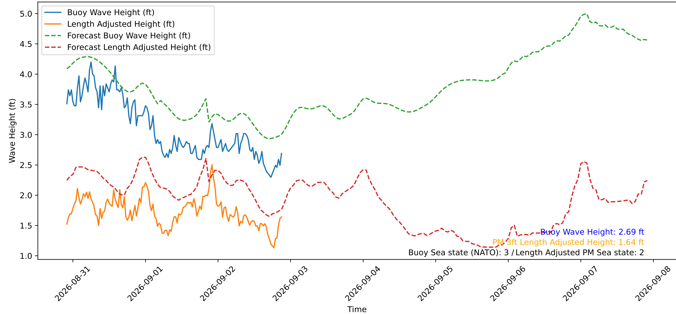
Wave Heights over Time for Red Beach at 2026-09-02 21:50:50
