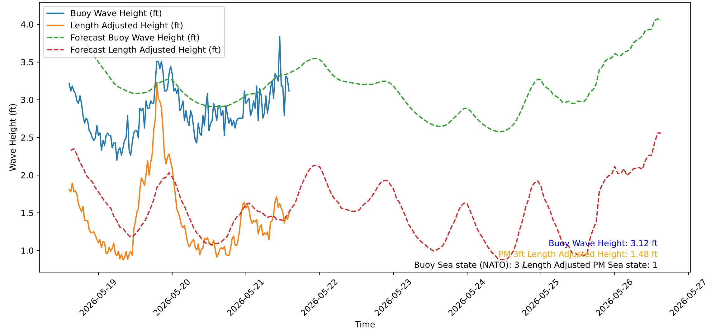
Wave Heights over Time for Oceanside Harbor at 2026-05-21 14:30:32
