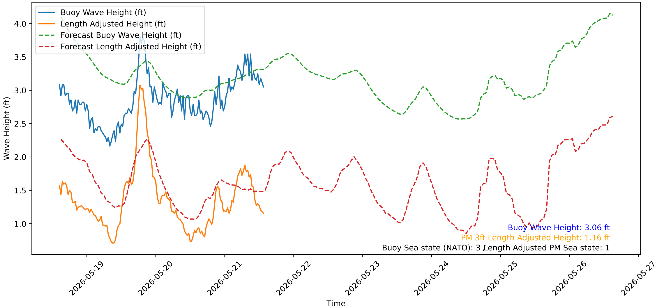
Wave Heights over Time for Green Beach at 2026-05-21 14:31:14
