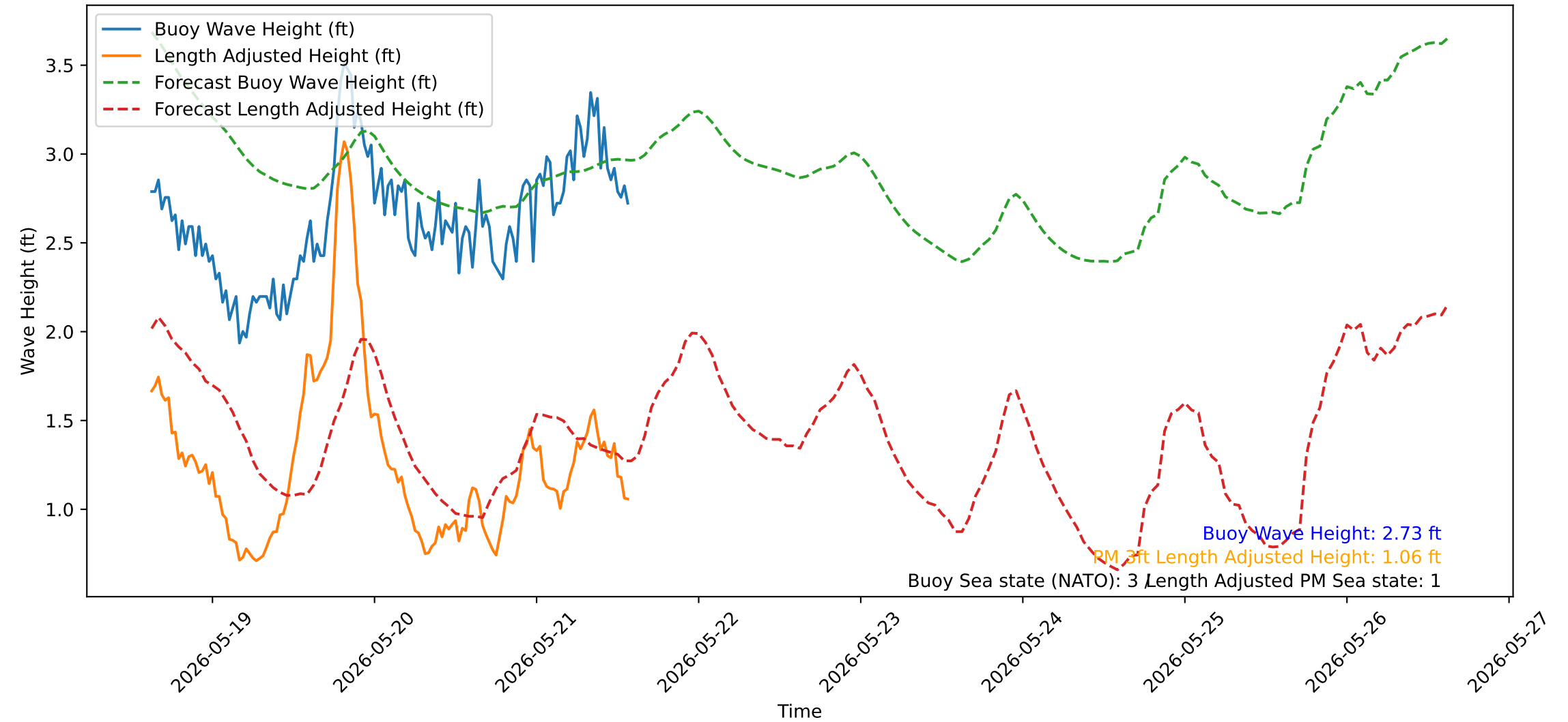
Wave Heights over Time for Red Beach at 2026-05-21 14:30:51
