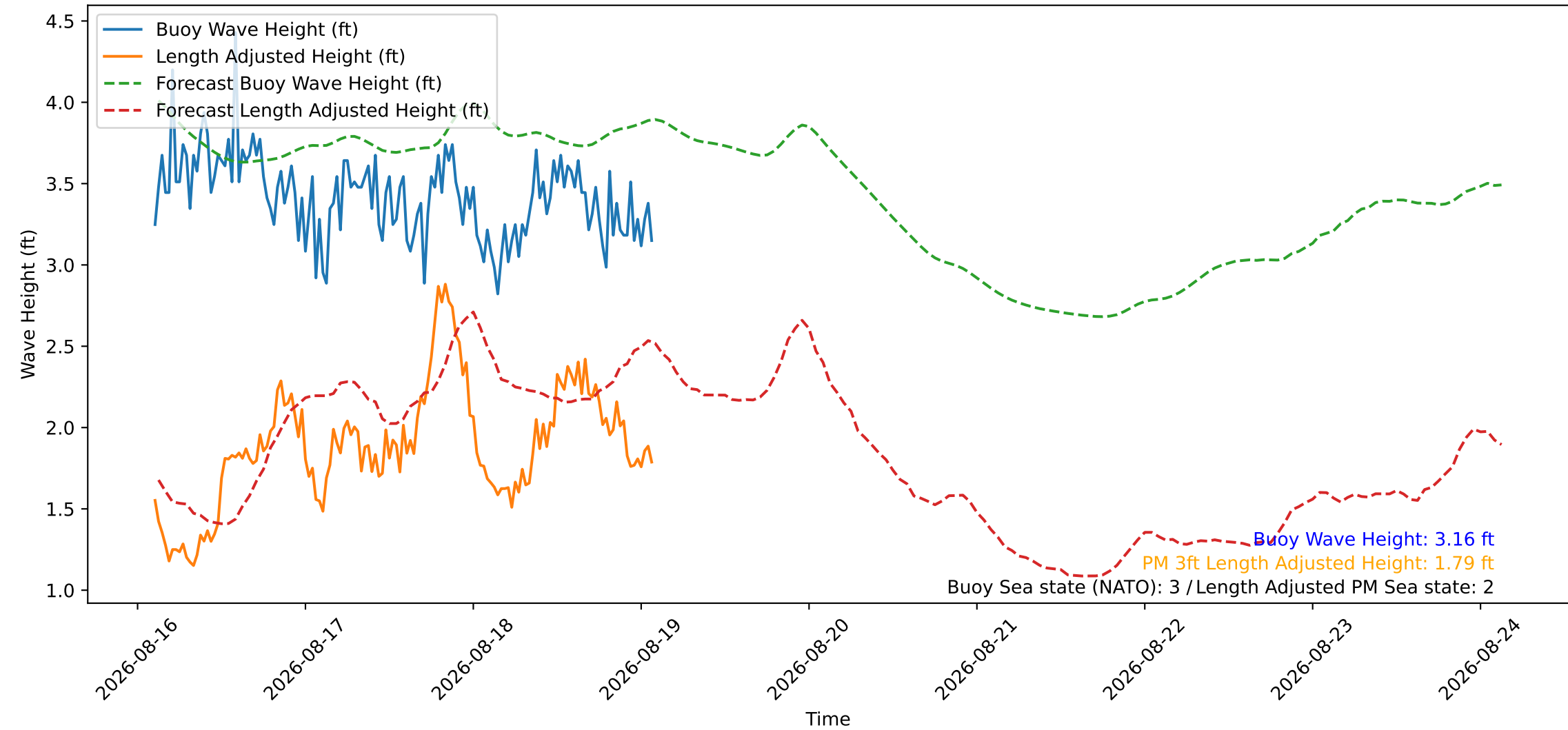
Wave Heights over Time for Oceanside Harbor at 2026-08-19 02:40:26
