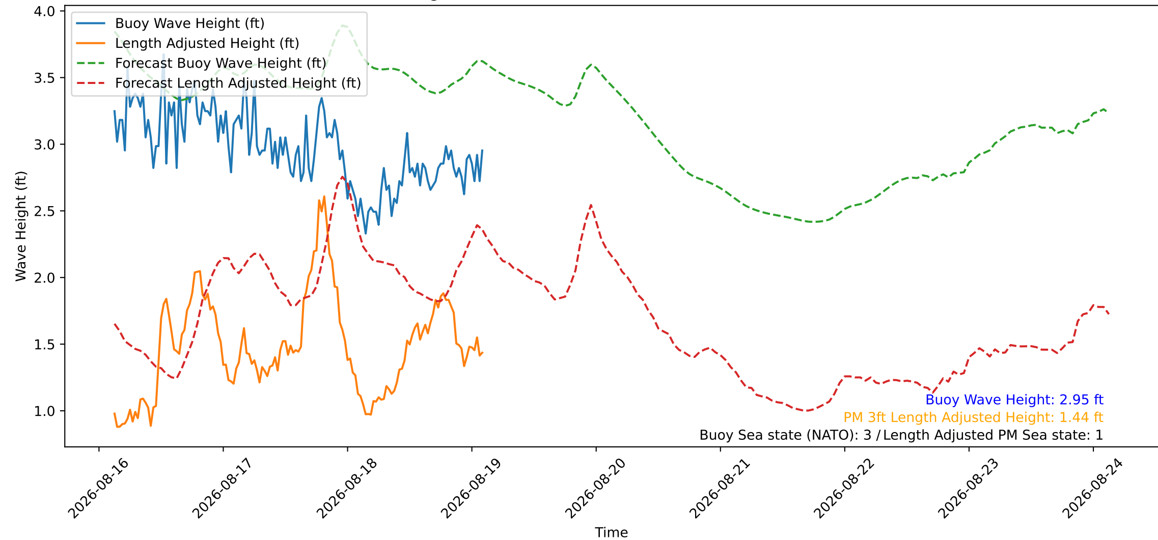
Wave Heights over Time for Red Beach at 2026-08-19 02:40:45
