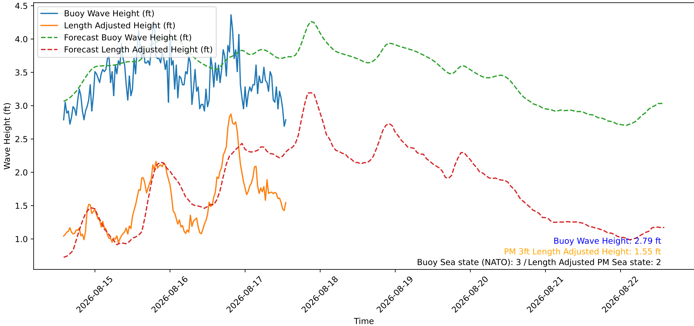
Wave Heights over Time for Green Beach at 2026-08-17 13:41:08
