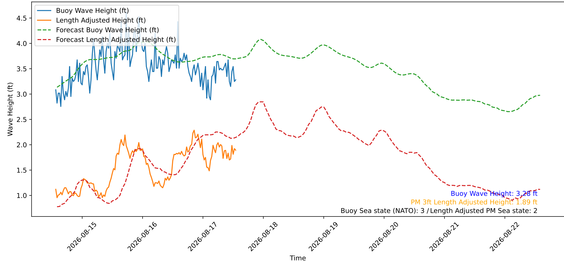
Wave Heights over Time for Oceanside Harbor at 2026-08-17 13:40:26
