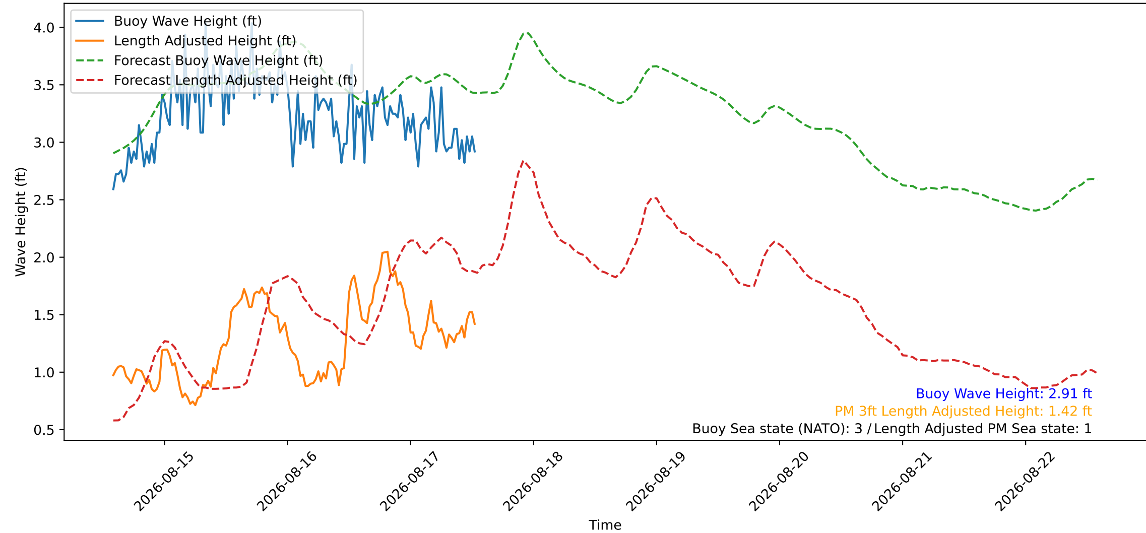
Wave Heights over Time for Red Beach at 2026-08-17 13:40:46
