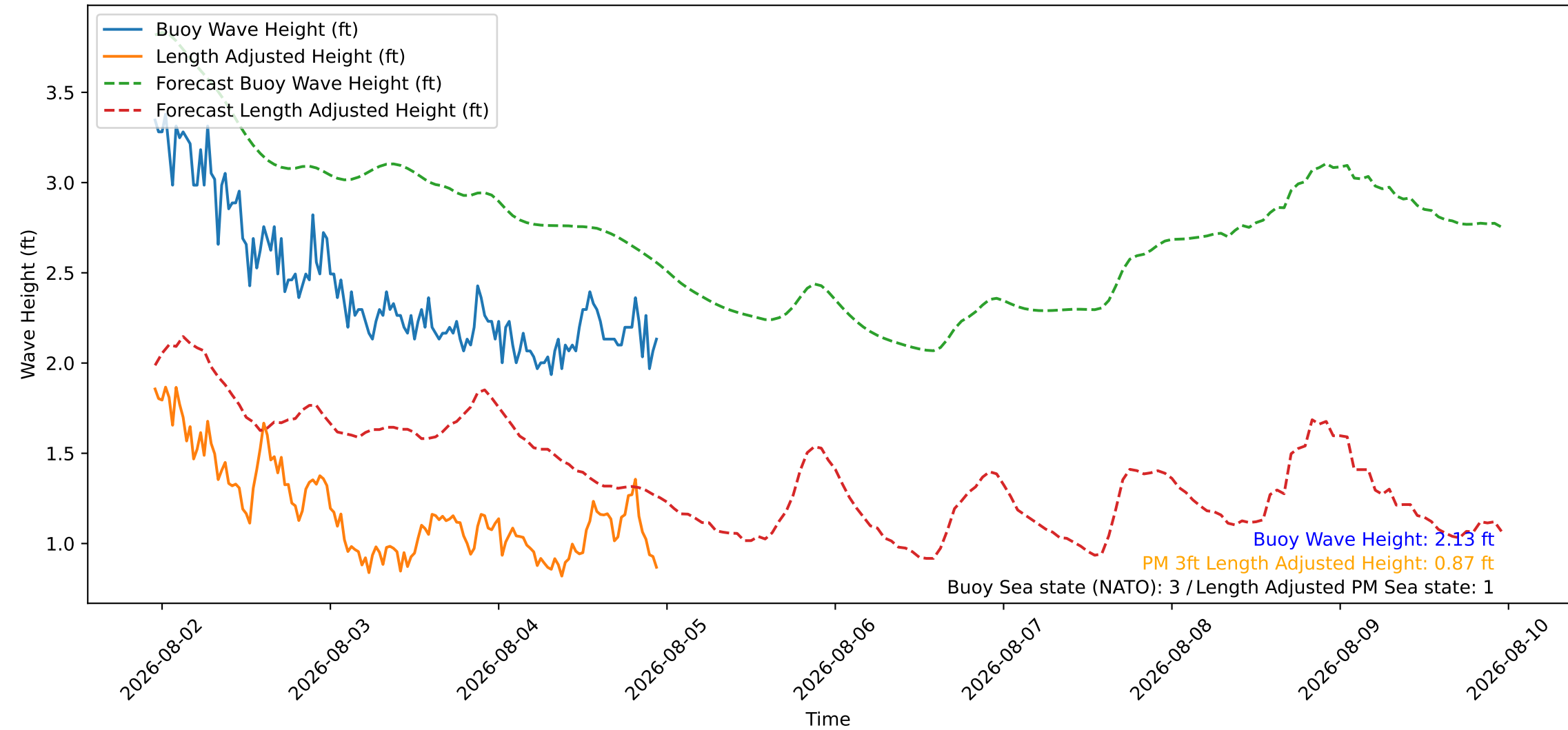
Wave Heights over Time for Green Beach at 2026-08-04 23:11:09
