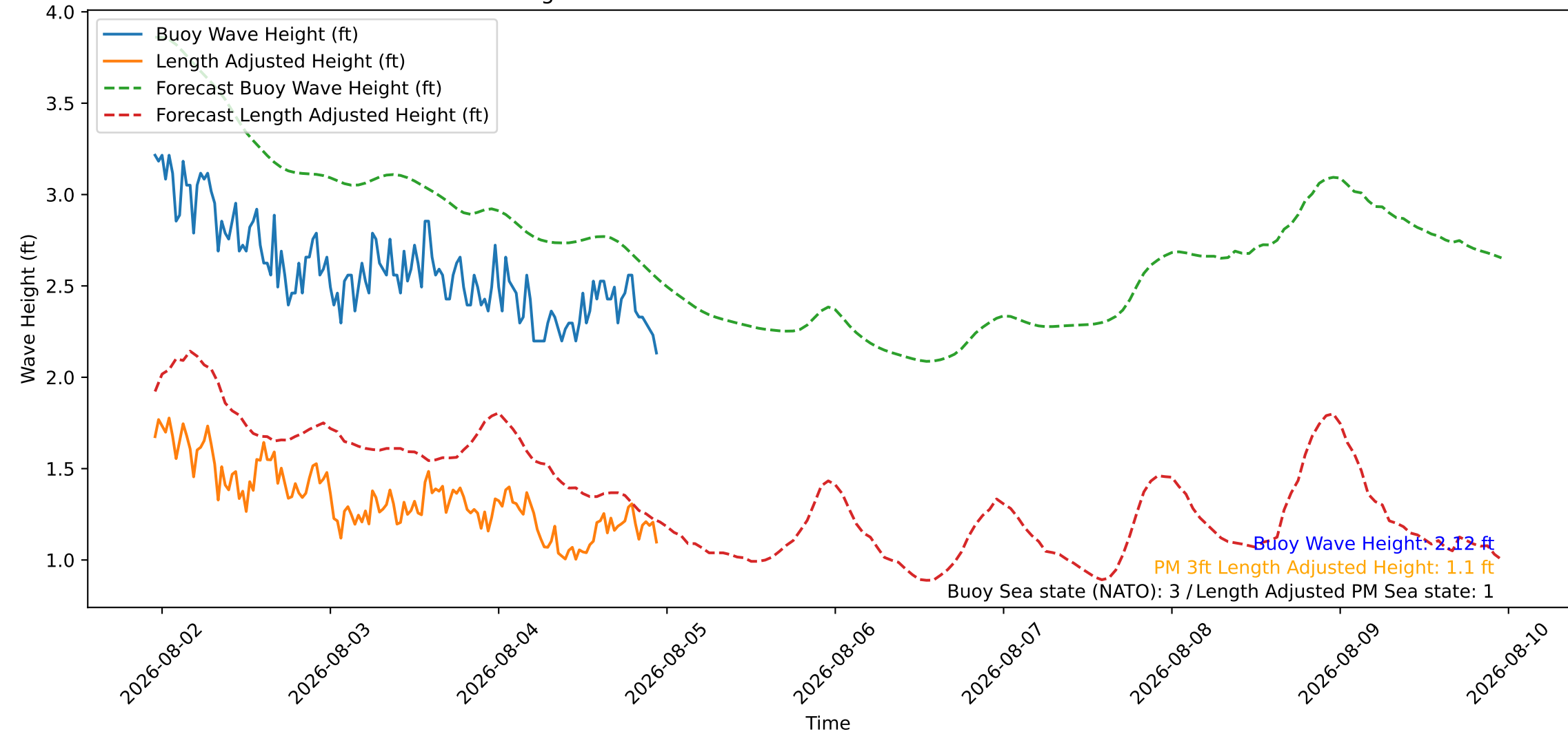
Wave Heights over Time for Oceanside Harbor at 2026-08-04 23:10:27
