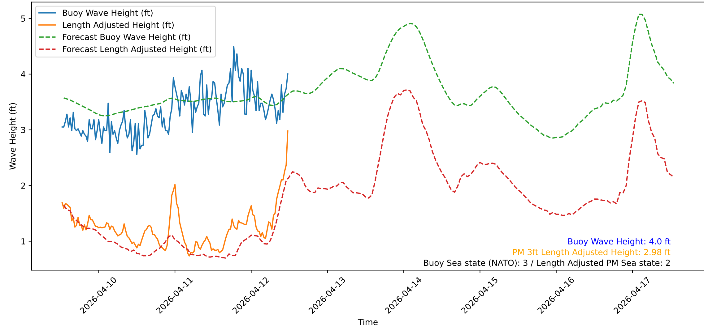
Wave Heights over Time for Green Beach at 2026-04-12 12:31:14
