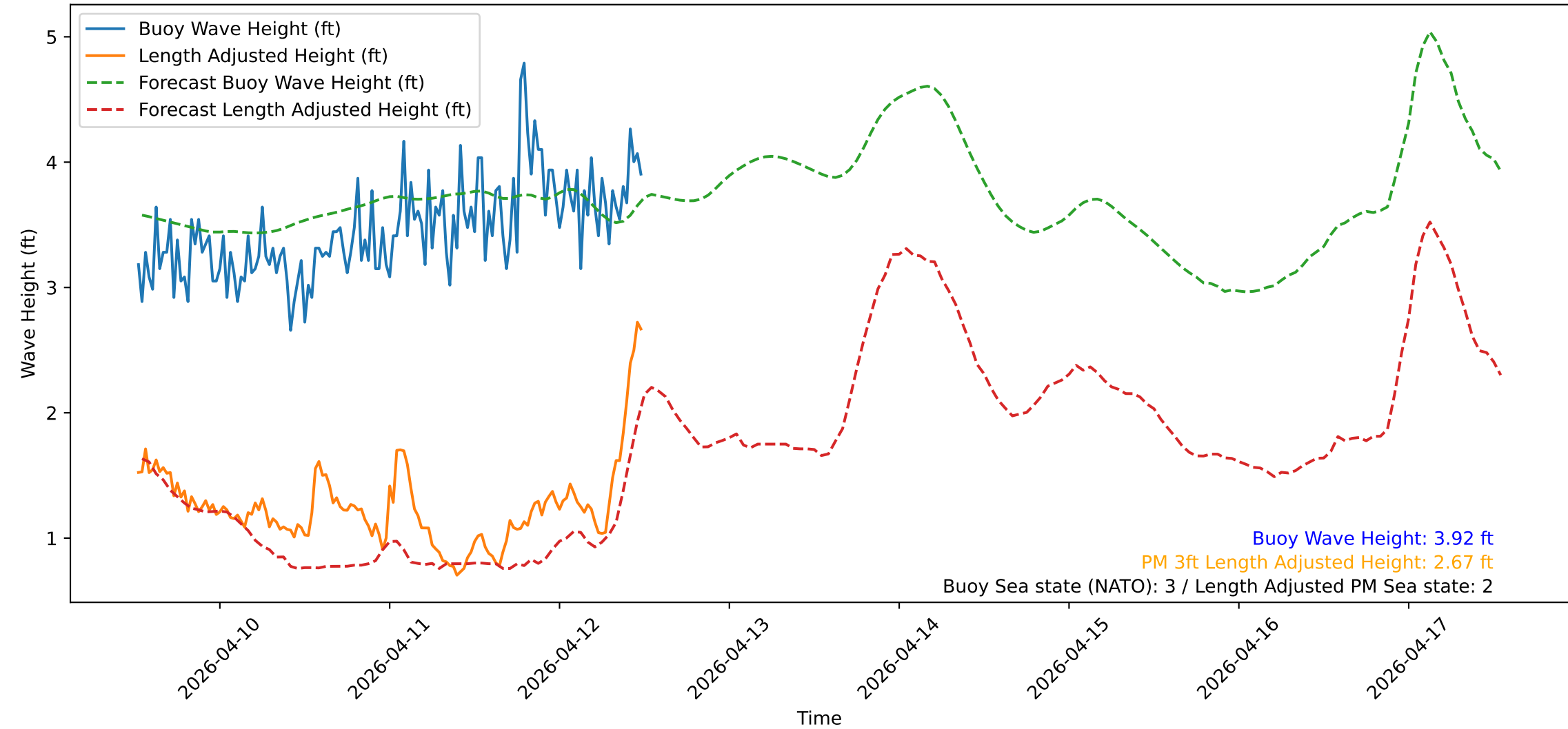
Wave Heights over Time for Oceanside Harbor at 2026-04-12 12:30:32
