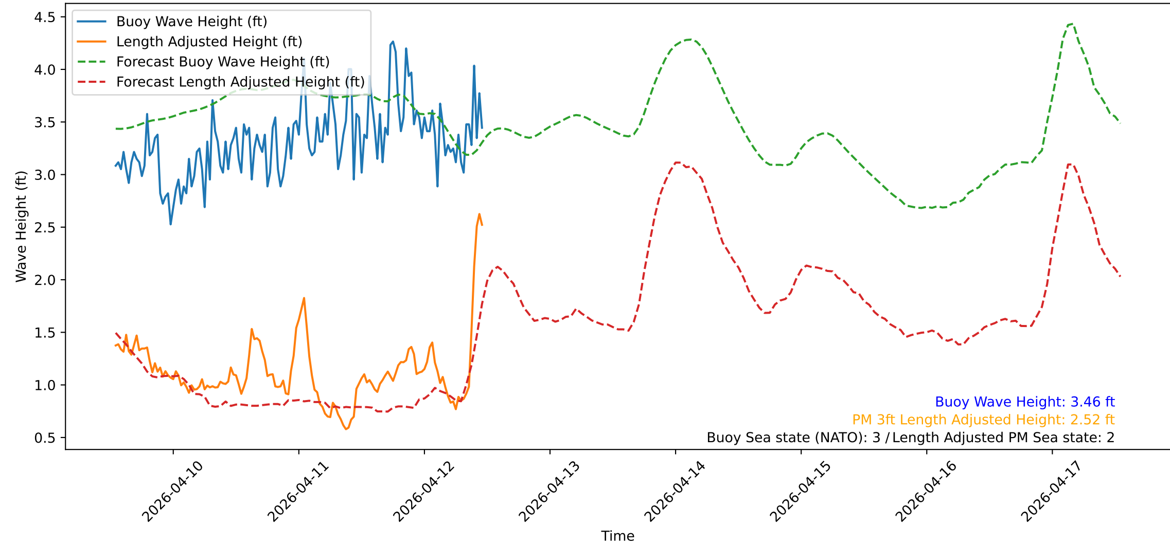
Wave Heights over Time for Red Beach at 2026-04-12 12:30:51
