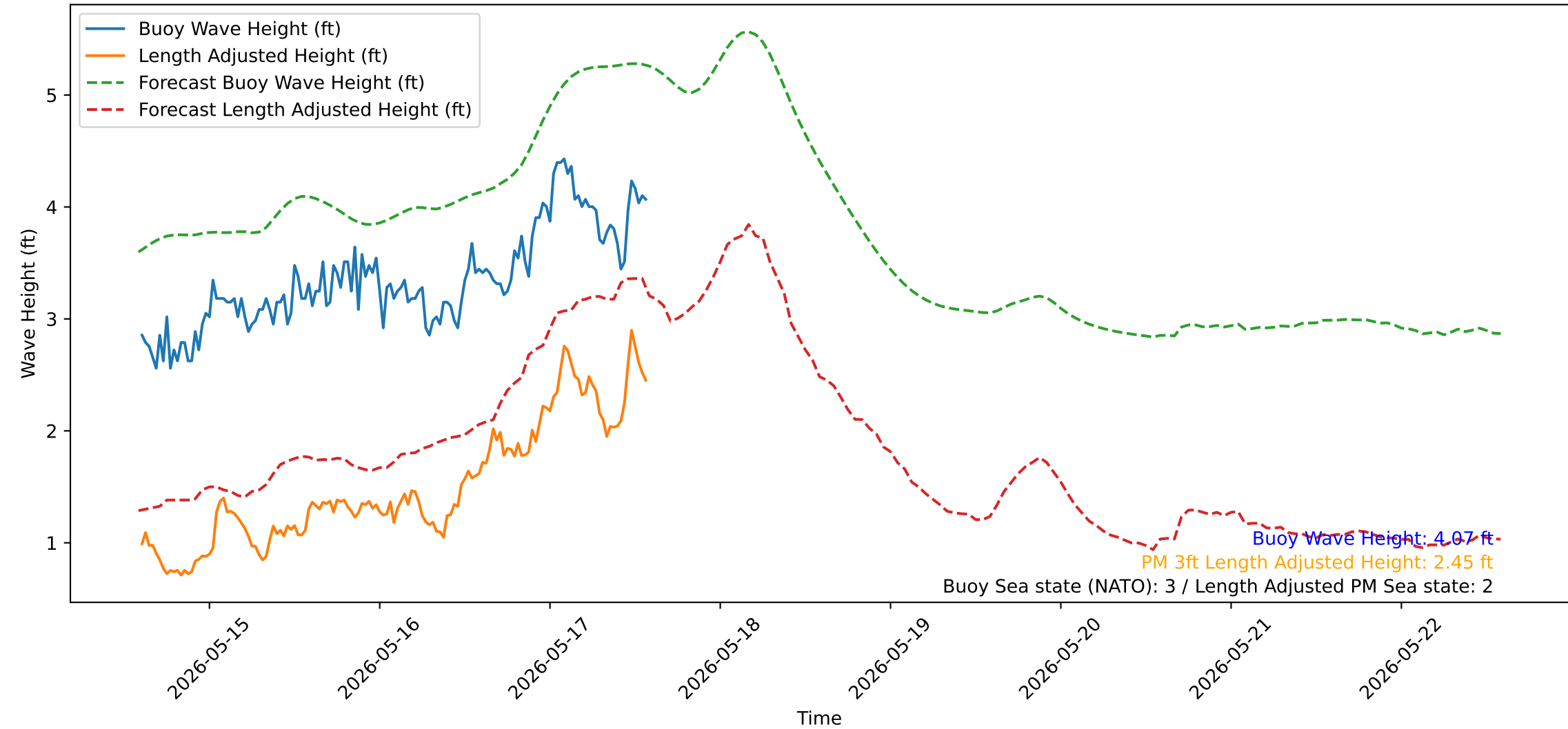
Wave Heights over Time for Green Beach at 2026-05-17 14:21:14
