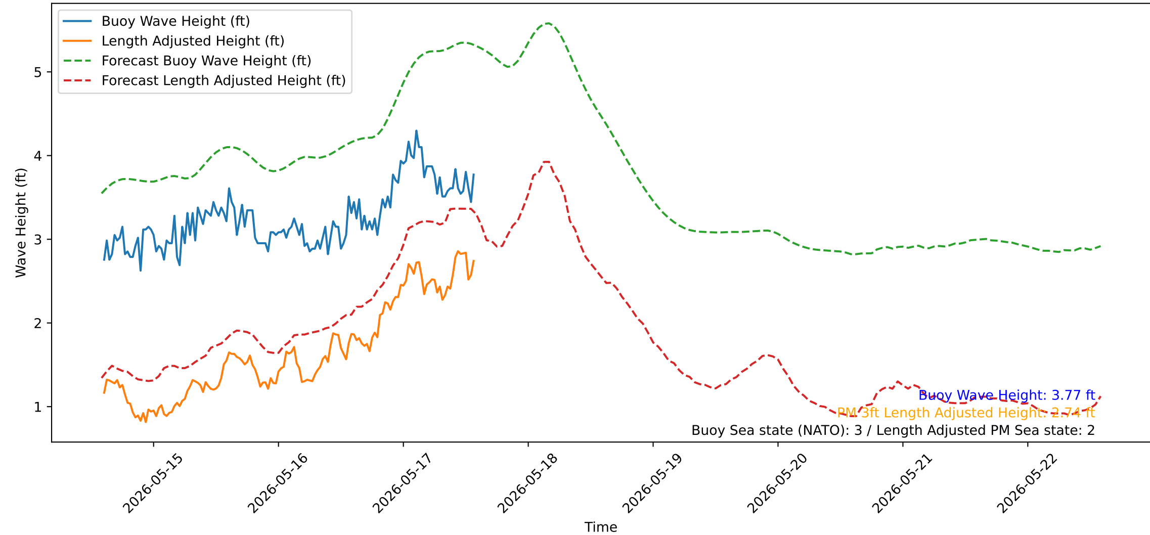
Wave Heights over Time for Oceanside Harbor at 2026-05-17 14:20:31
