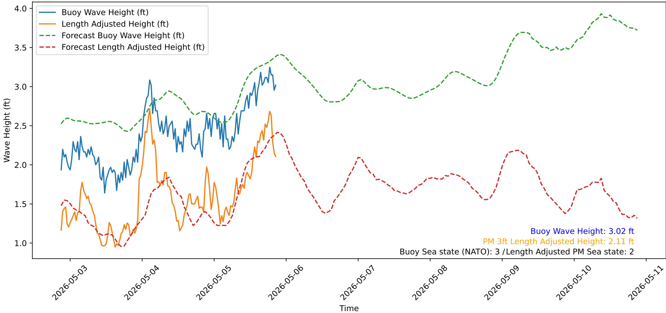
Wave Heights over Time for Oceanside Harbor at 2026-05-05 21:10:31
