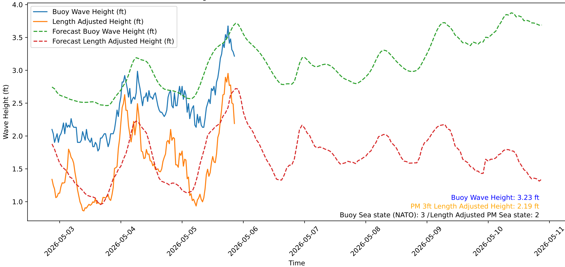
Wave Heights over Time for Green Beach at 2026-05-05 21:11:13
