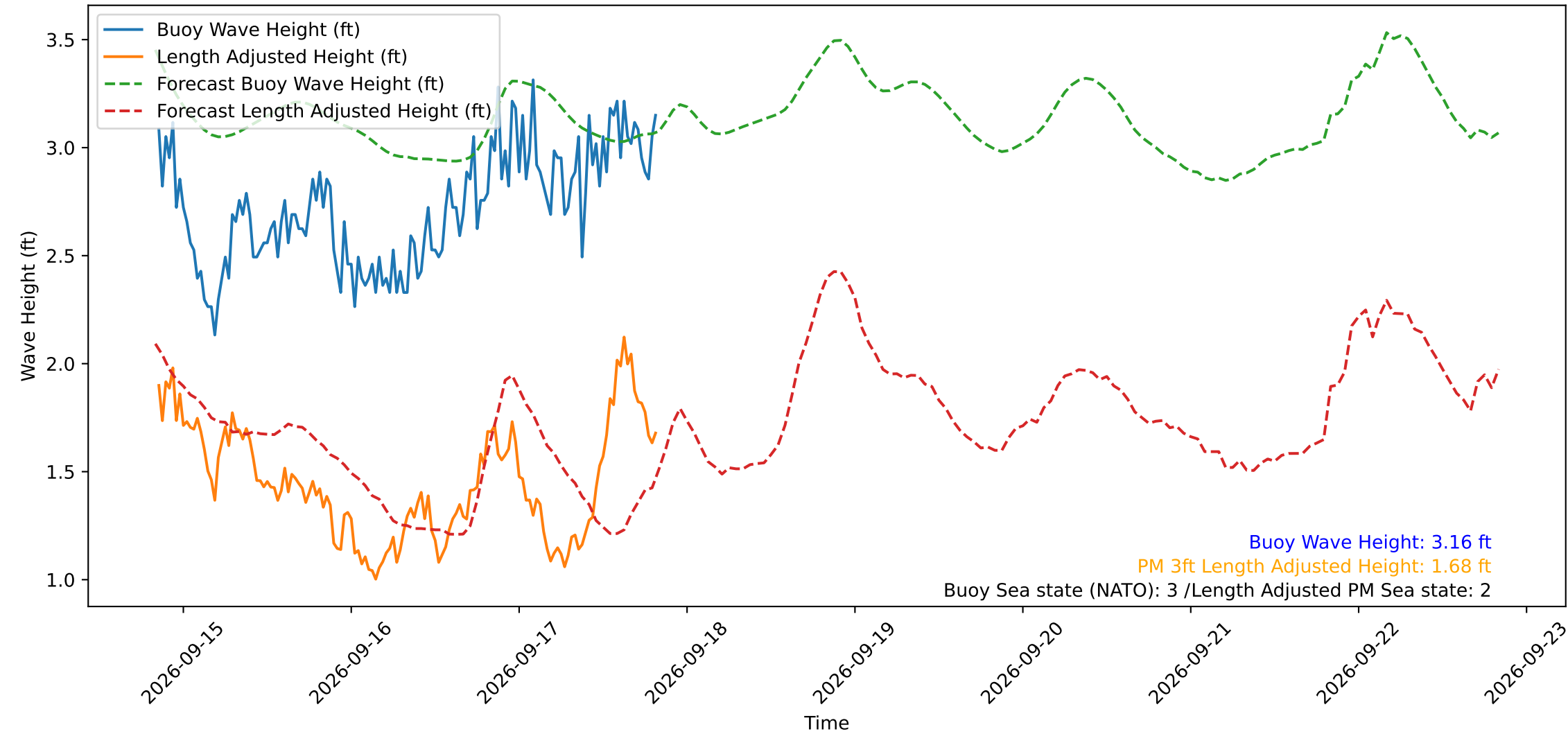
Wave Heights over Time for Green Beach at 2026-09-17 20:21:15
