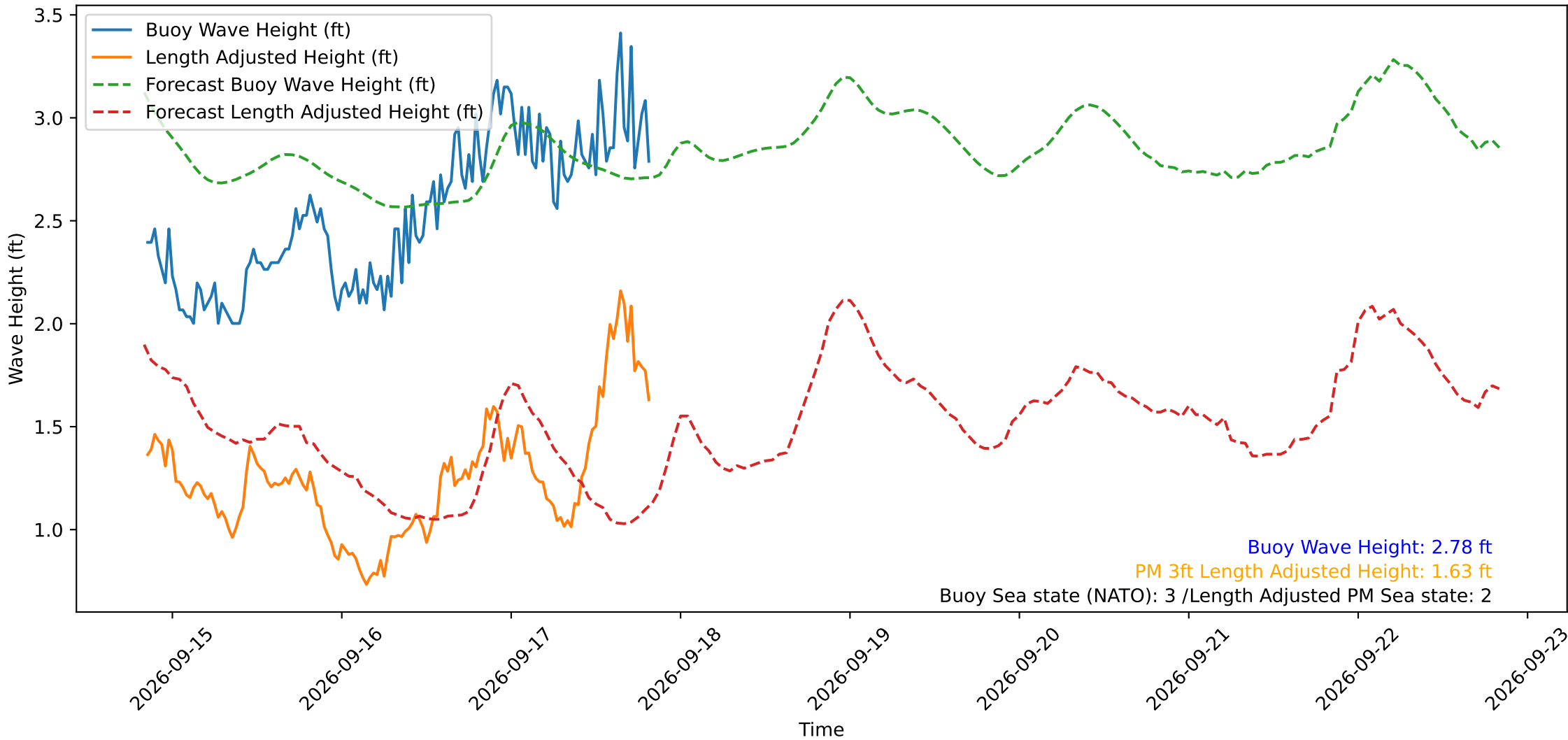
Wave Heights over Time for Red Beach at 2026-09-17 20:20:51
