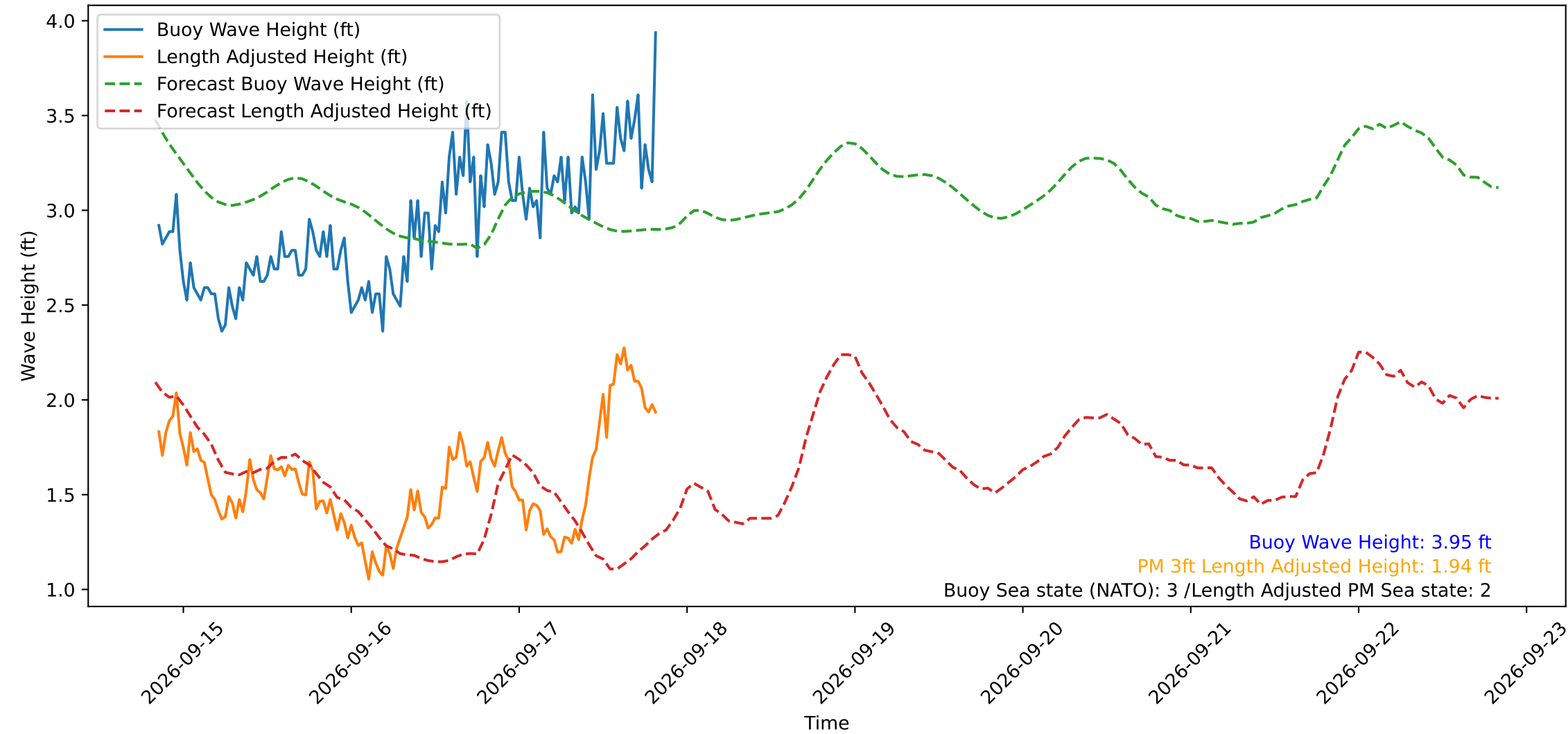
Wave Heights over Time for Oceanside Harbor at 2026-09-17 20:20:30
