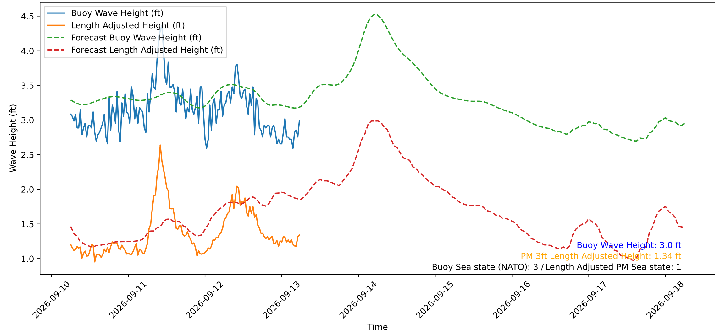
Wave Heights over Time for Oceanside Harbor at 2026-09-13 06:10:30
