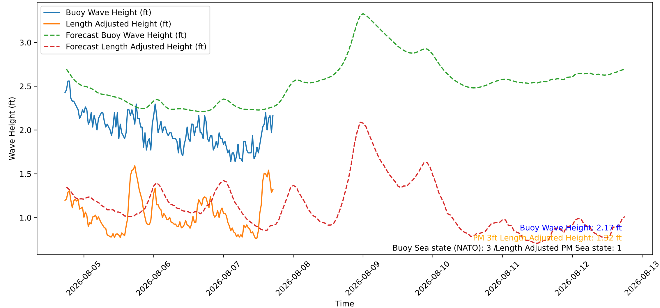
Wave Heights over Time for Oceanside Harbor at 2026-08-07 17:30:26
