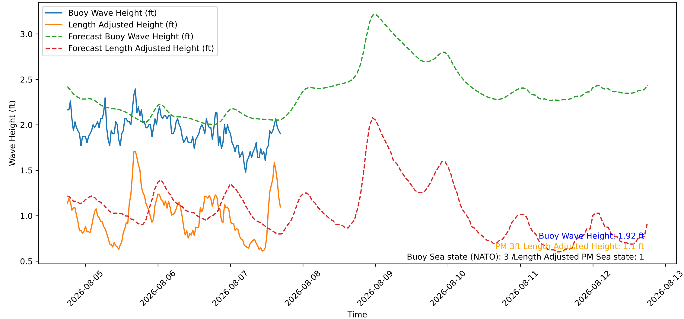
Wave Heights over Time for Red Beach at 2026-08-07 17:30:45
