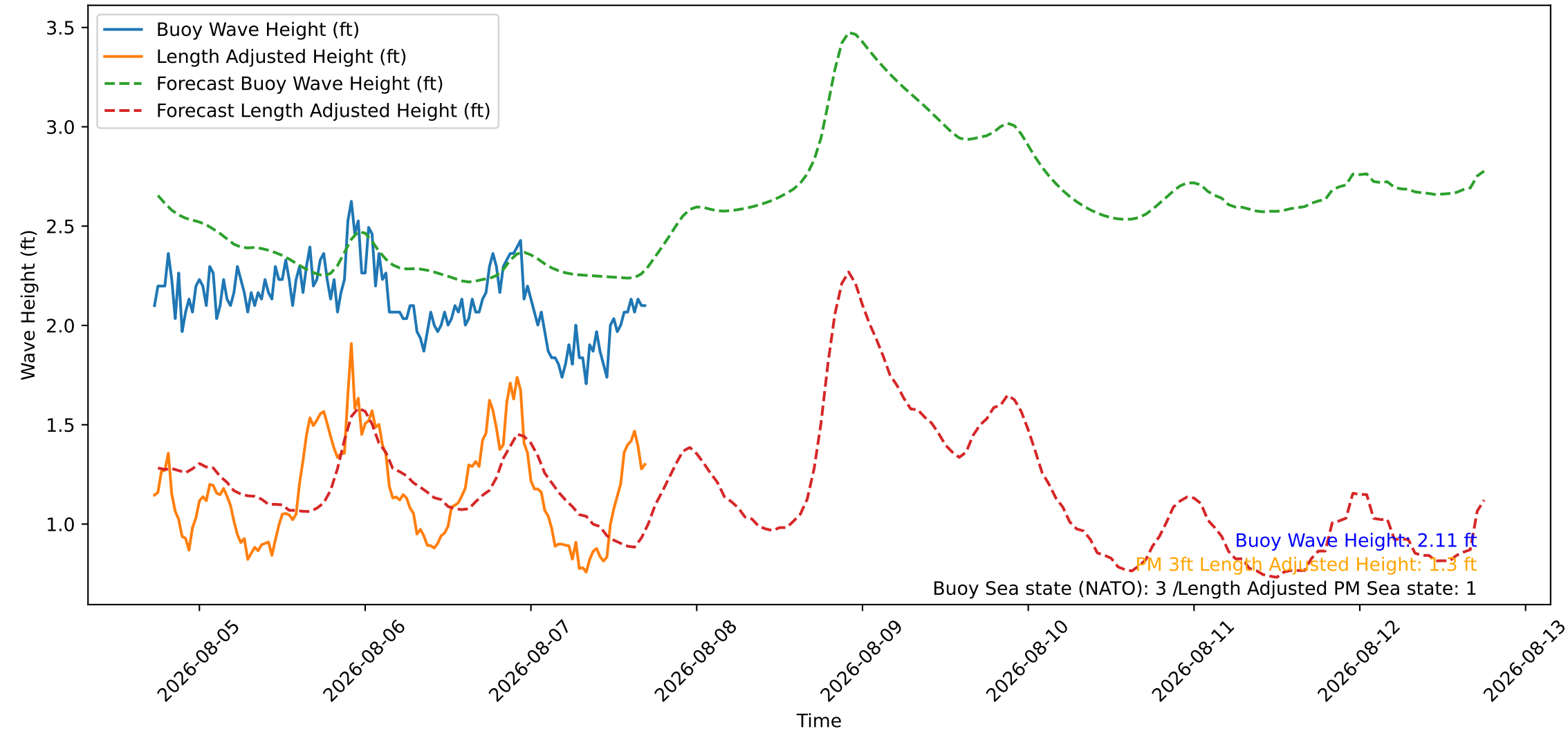
Wave Heights over Time for Green Beach at 2026-08-07 17:31:08
