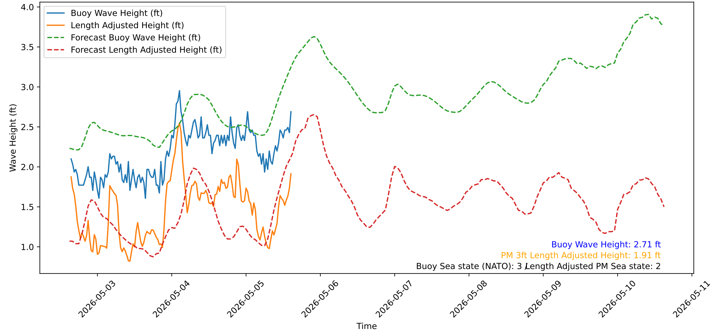
Wave Heights over Time for Red Beach at 2026-05-05 15:10:50
