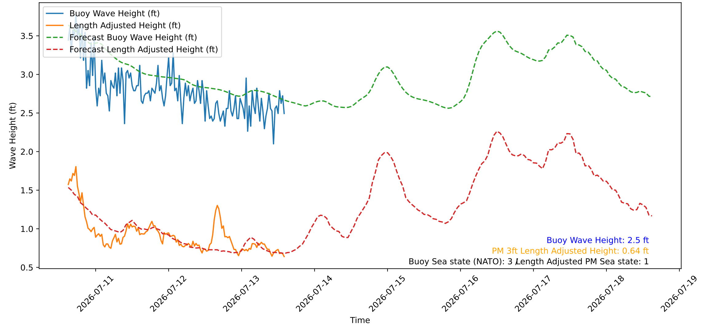
Wave Heights over Time for Oceanside Harbor at 2026-07-13 15:00:26
