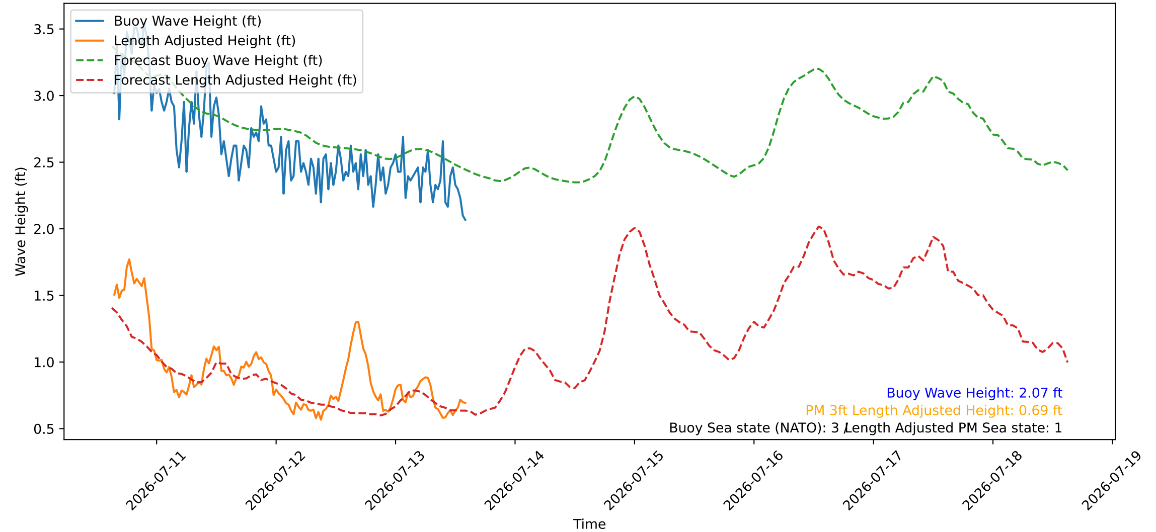
Wave Heights over Time for Red Beach at 2026-07-13 15:00:46
