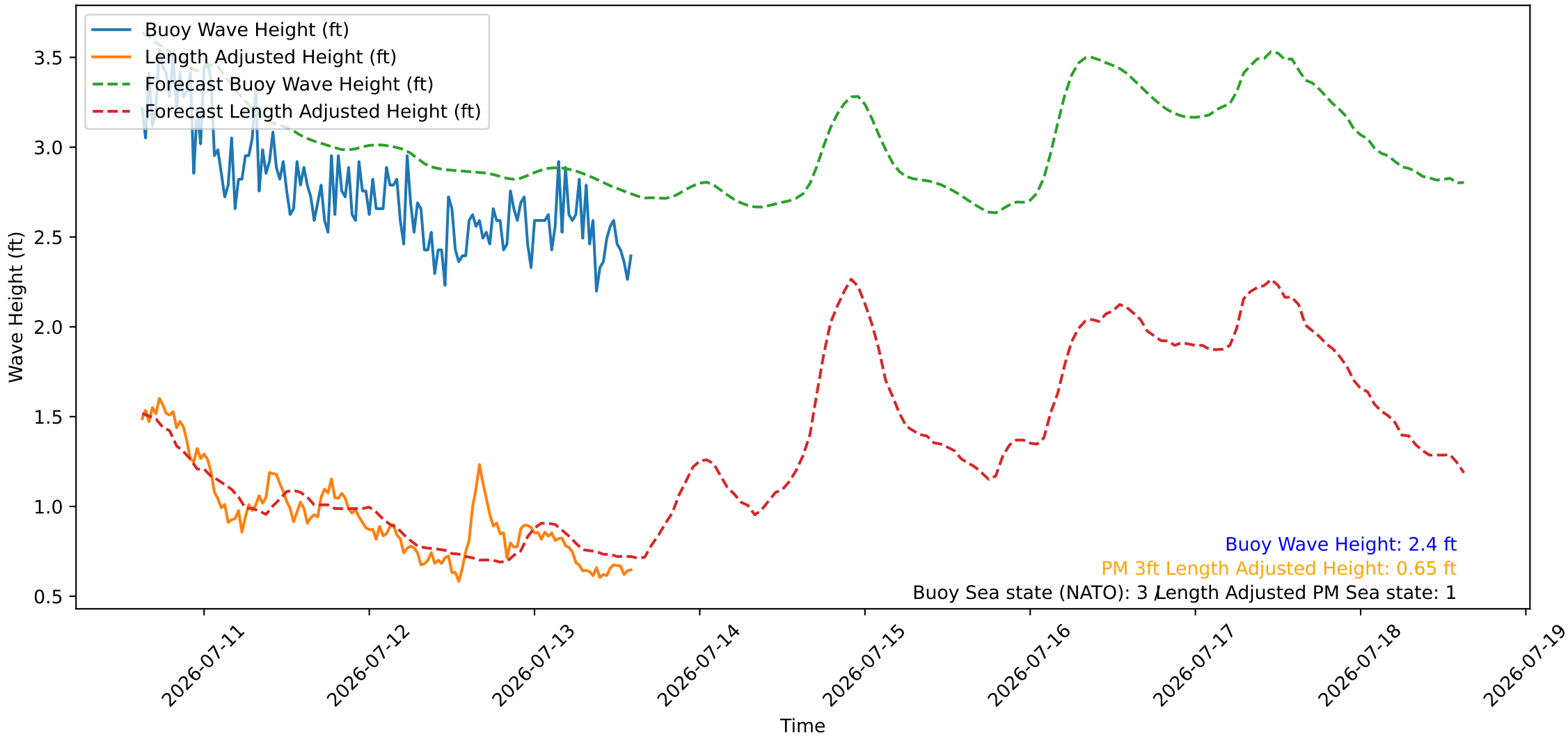
Wave Heights over Time for Green Beach at 2026-07-13 15:01:09
