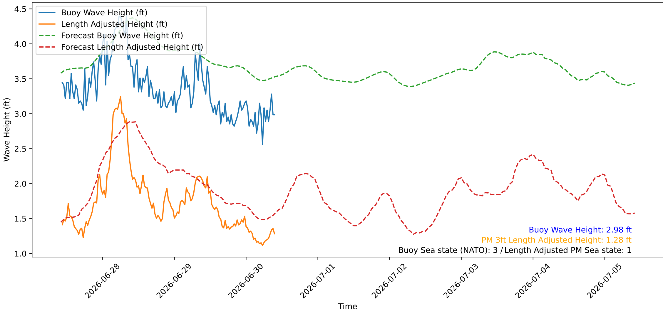
Wave Heights over Time for Oceanside Harbor at 2026-06-30 10:20:25
