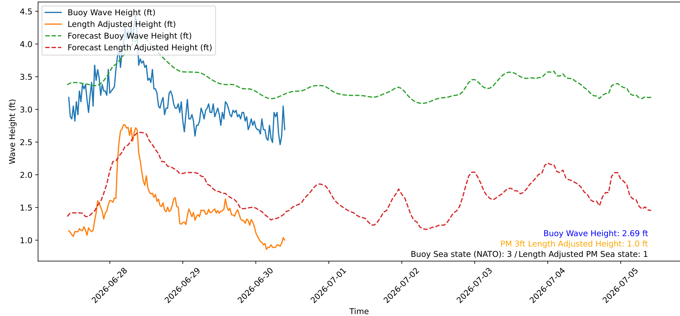
Wave Heights over Time for Red Beach at 2026-06-30 10:20:46
