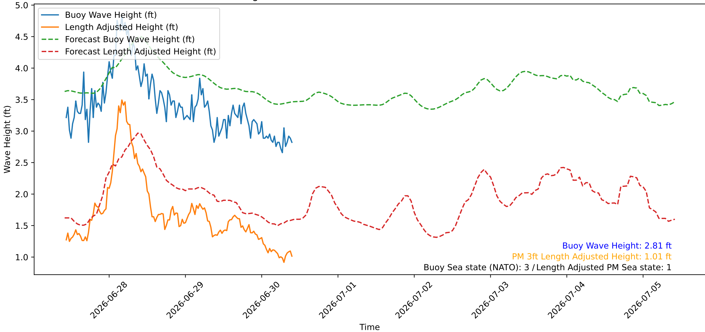
Wave Heights over Time for Green Beach at 2026-06-30 10:21:08
