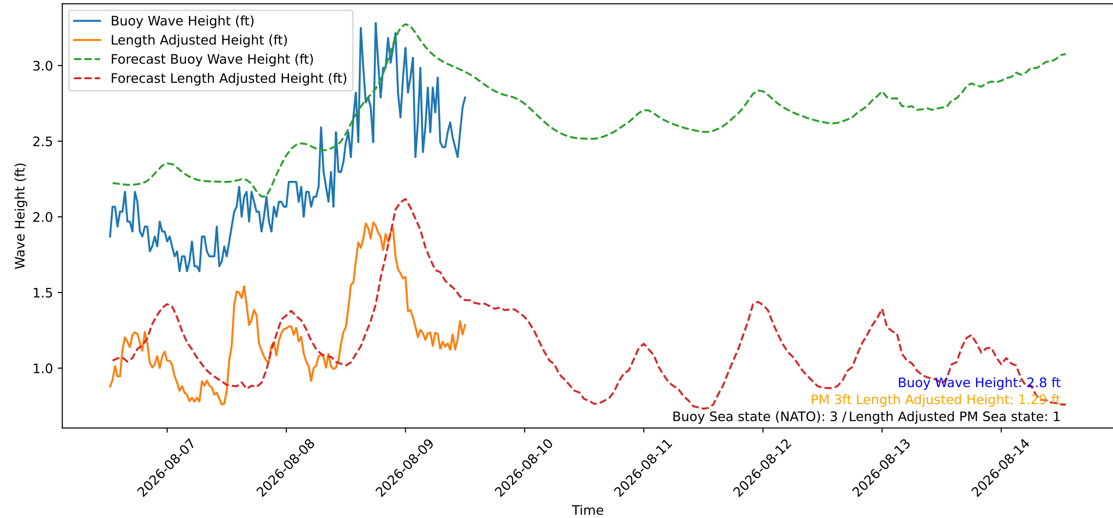
Wave Heights over Time for Oceanside Harbor at 2026-08-09 12:40:27
