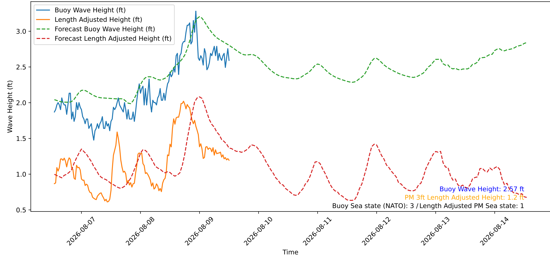
Wave Heights over Time for Red Beach at 2026-08-09 12:40:47
