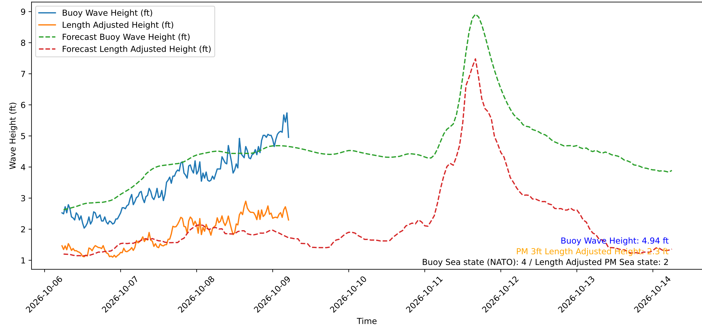
Wave Heights over Time for Oceanside Harbor at 2026-10-09 05:40:29
