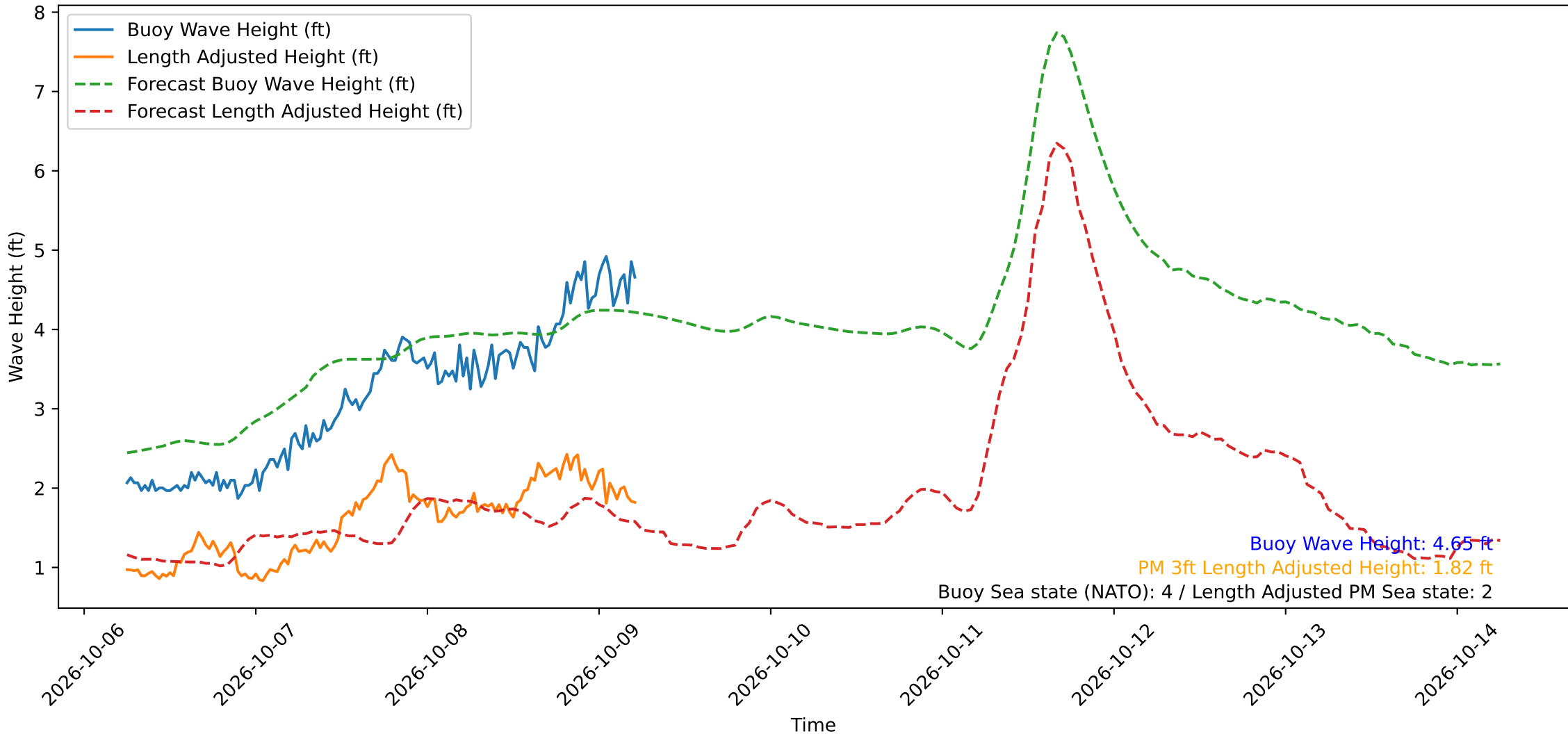
Wave Heights over Time for Red Beach at 2026-10-09 05:40:49
