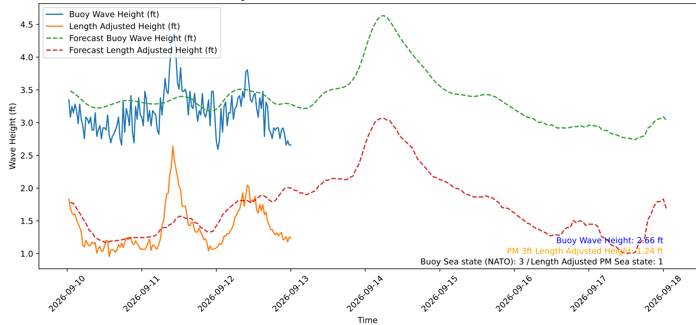
Wave Heights over Time for Oceanside Harbor at 2026-09-13 00:40:29
