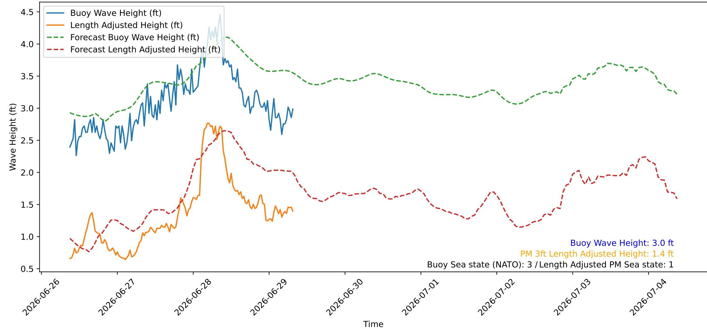
Wave Heights over Time for Red Beach at 2026-06-29 08:30:46
