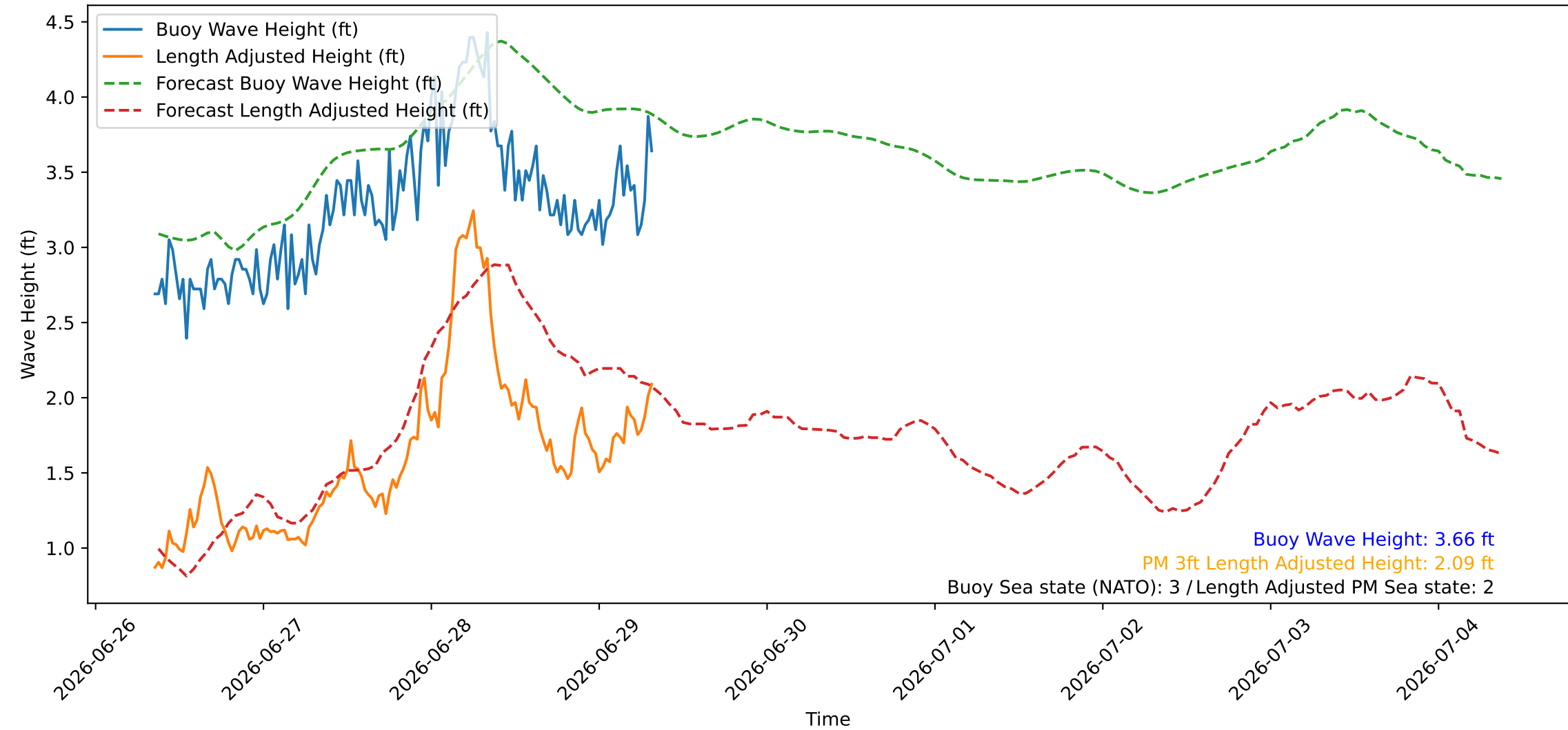
Wave Heights over Time for Oceanside Harbor at 2026-06-29 08:30:26
