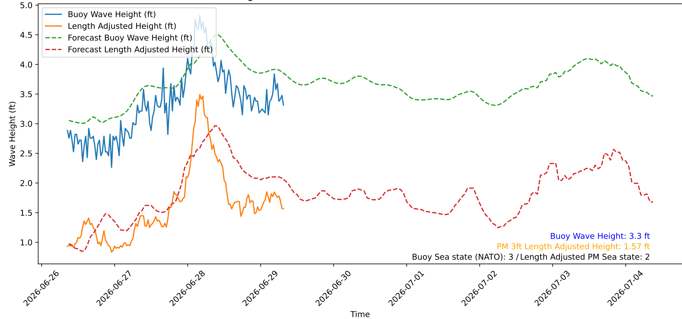
Wave Heights over Time for Green Beach at 2026-06-29 08:31:08
