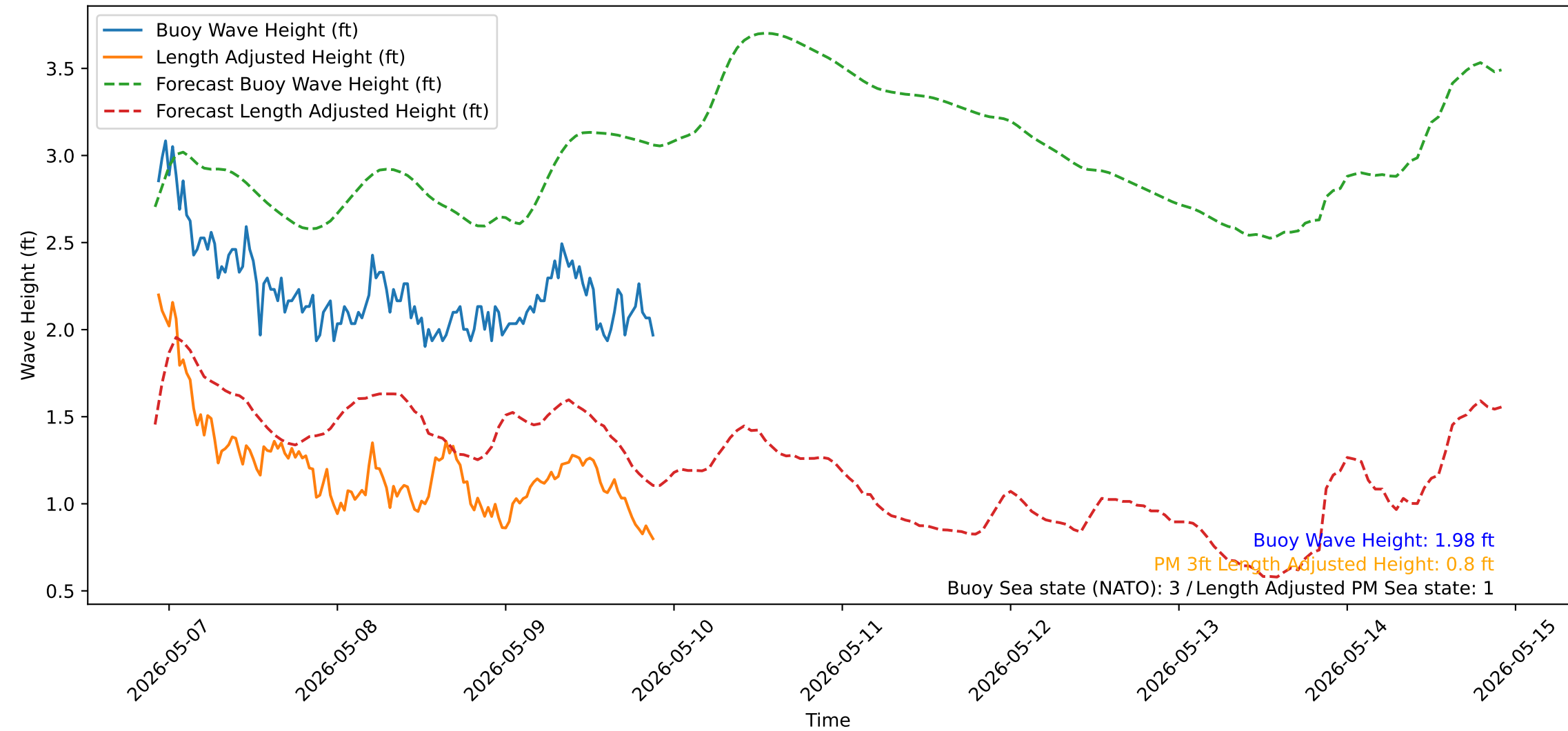
Wave Heights over Time for Red Beach at 2026-05-09 22:00:51
