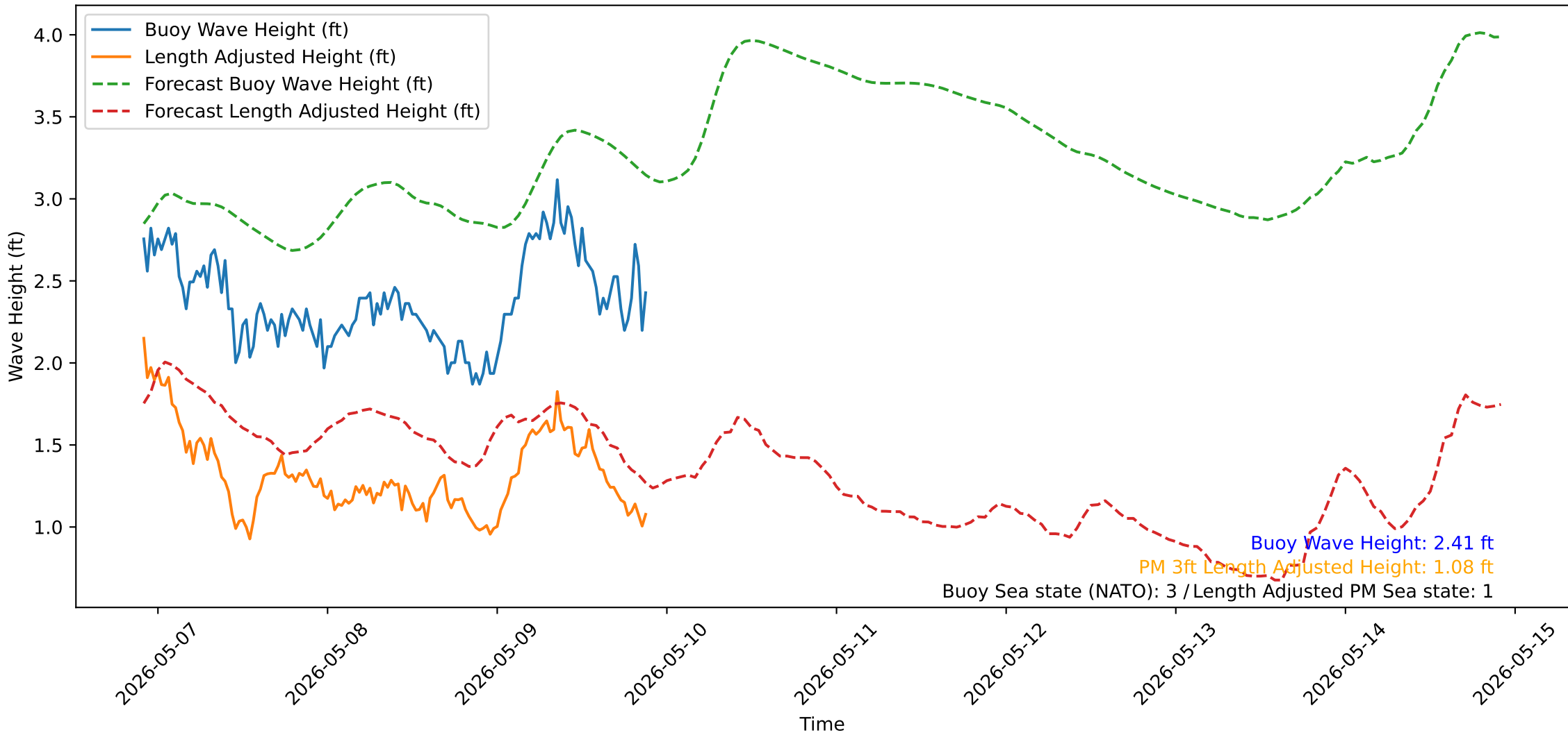
Wave Heights over Time for Oceanside Harbor at 2026-05-09 22:00:31
