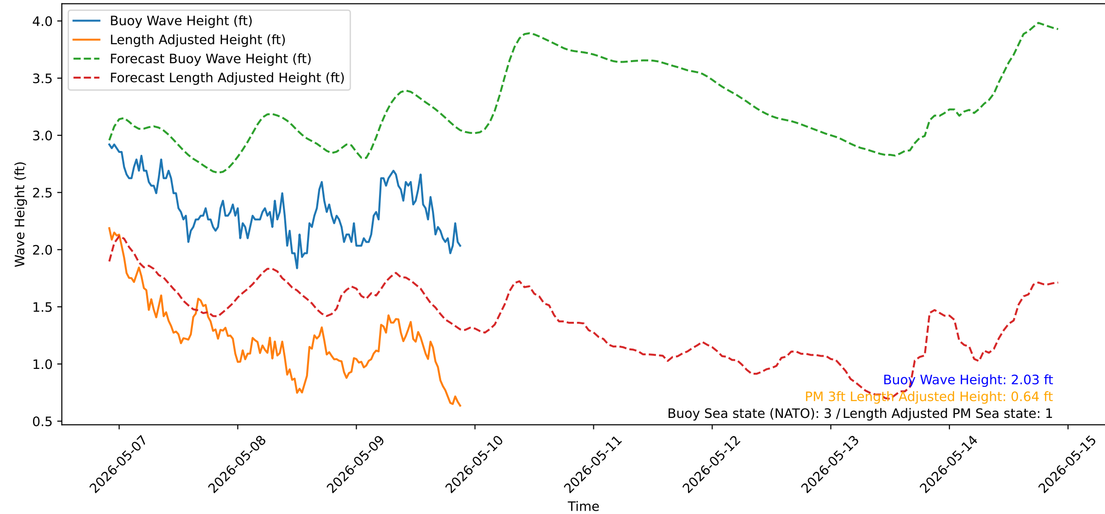
Wave Heights over Time for Green Beach at 2026-05-09 22:01:14
