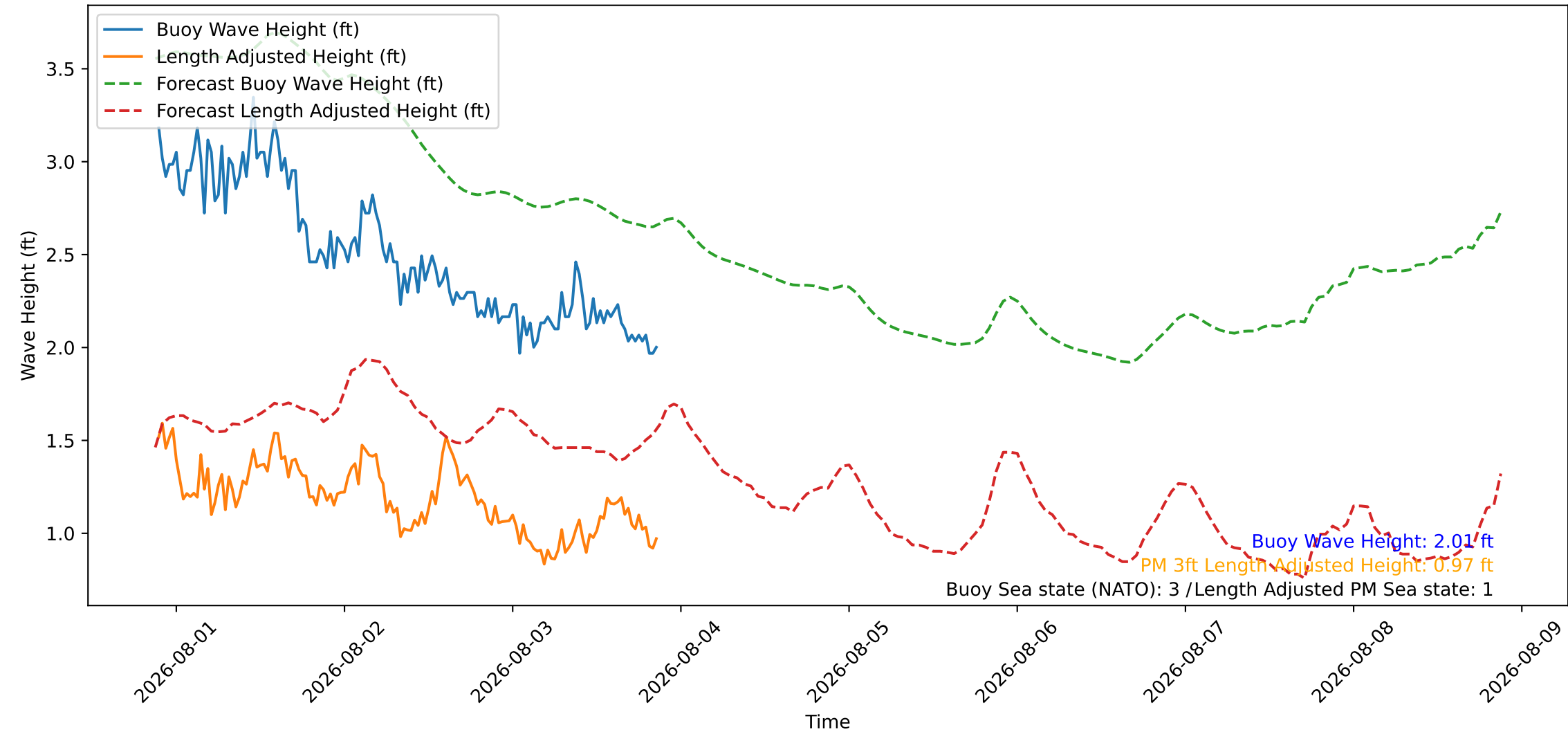
Wave Heights over Time for Red Beach at 2026-08-03 21:20:47
