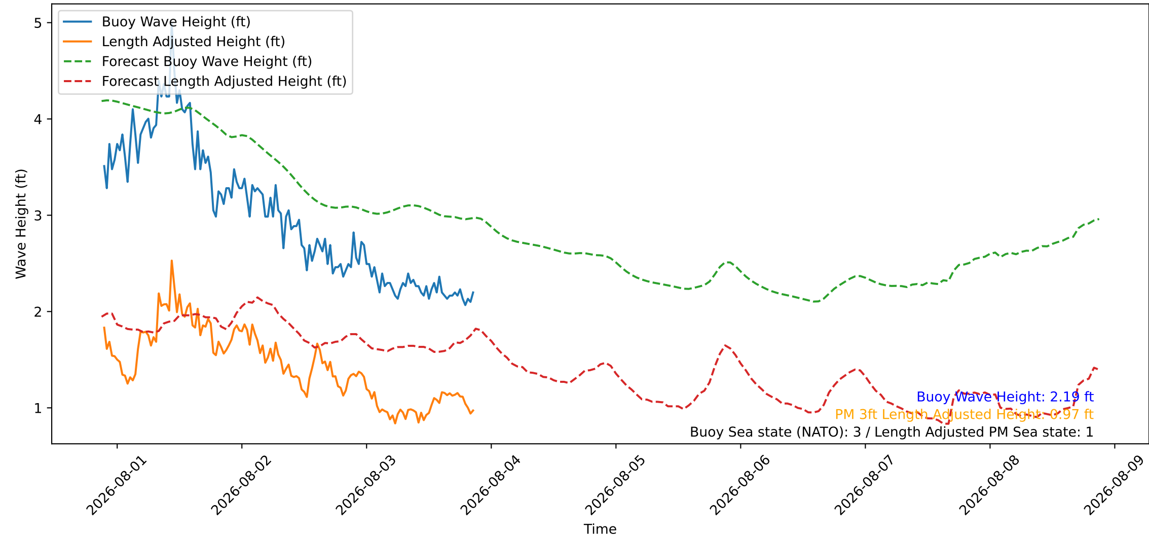
Wave Heights over Time for Green Beach at 2026-08-03 21:21:09
