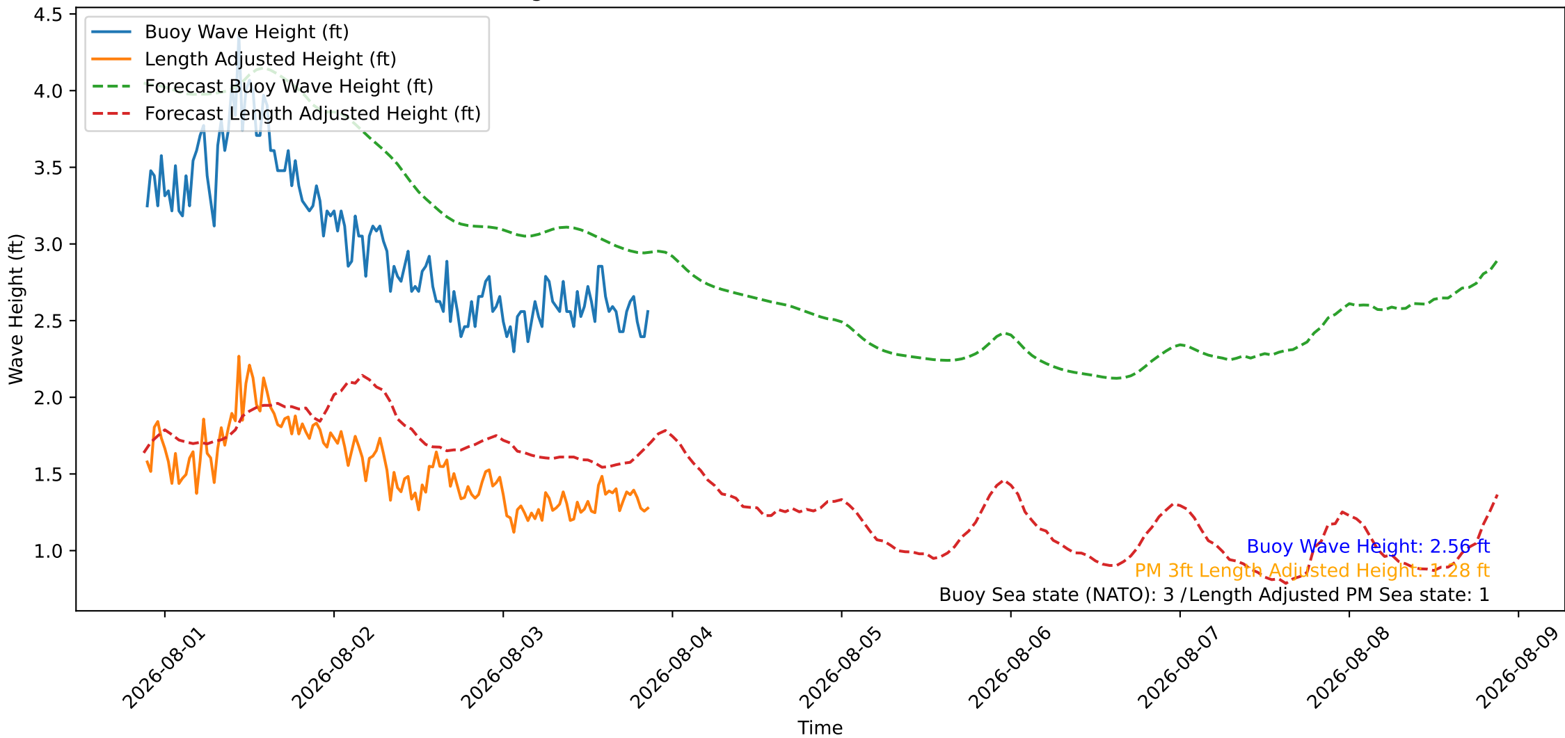
Wave Heights over Time for Oceanside Harbor at 2026-08-03 21:20:26
